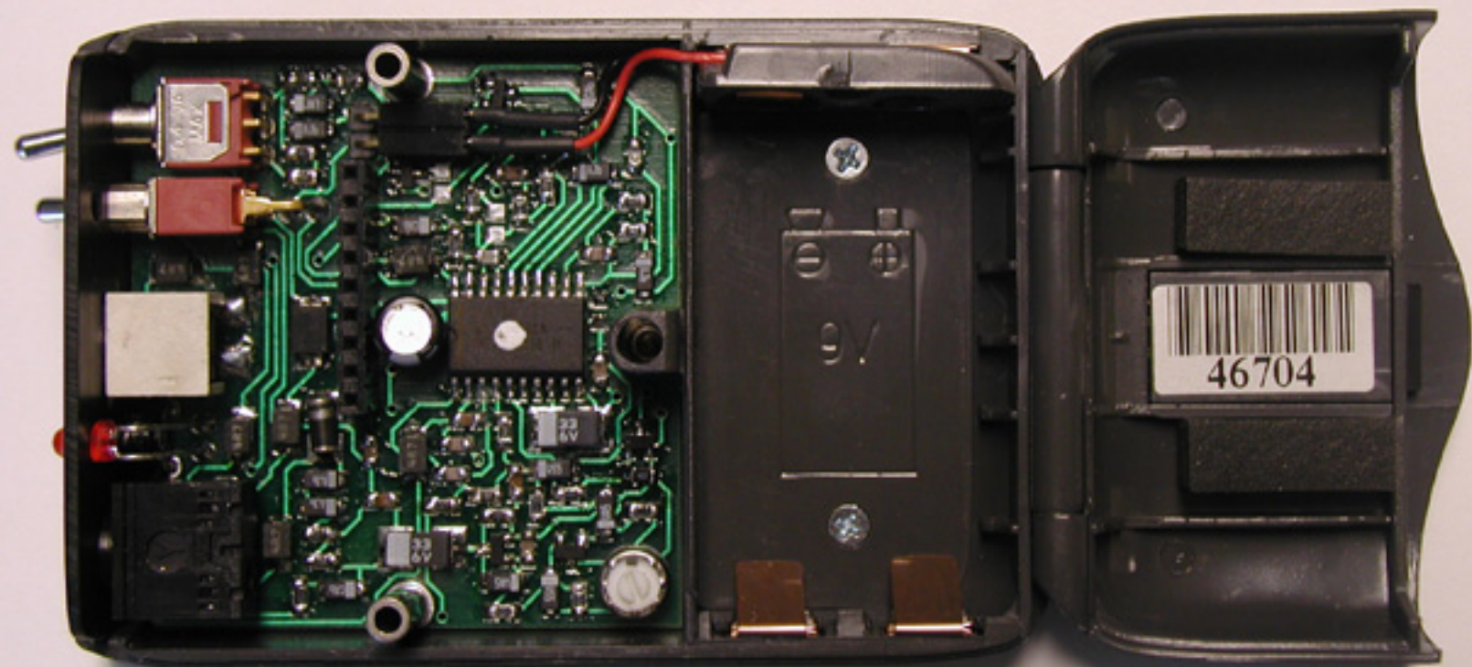
M-216 Transmitter open back view
