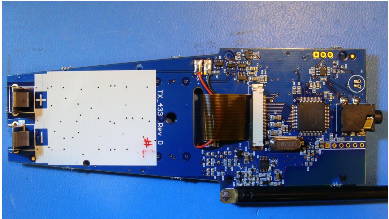
Photograph 3. PCB Rear
