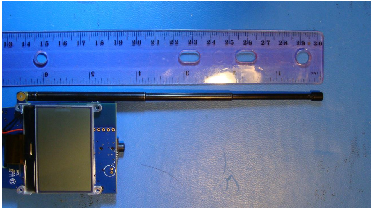
Photograph 1. Antenna
