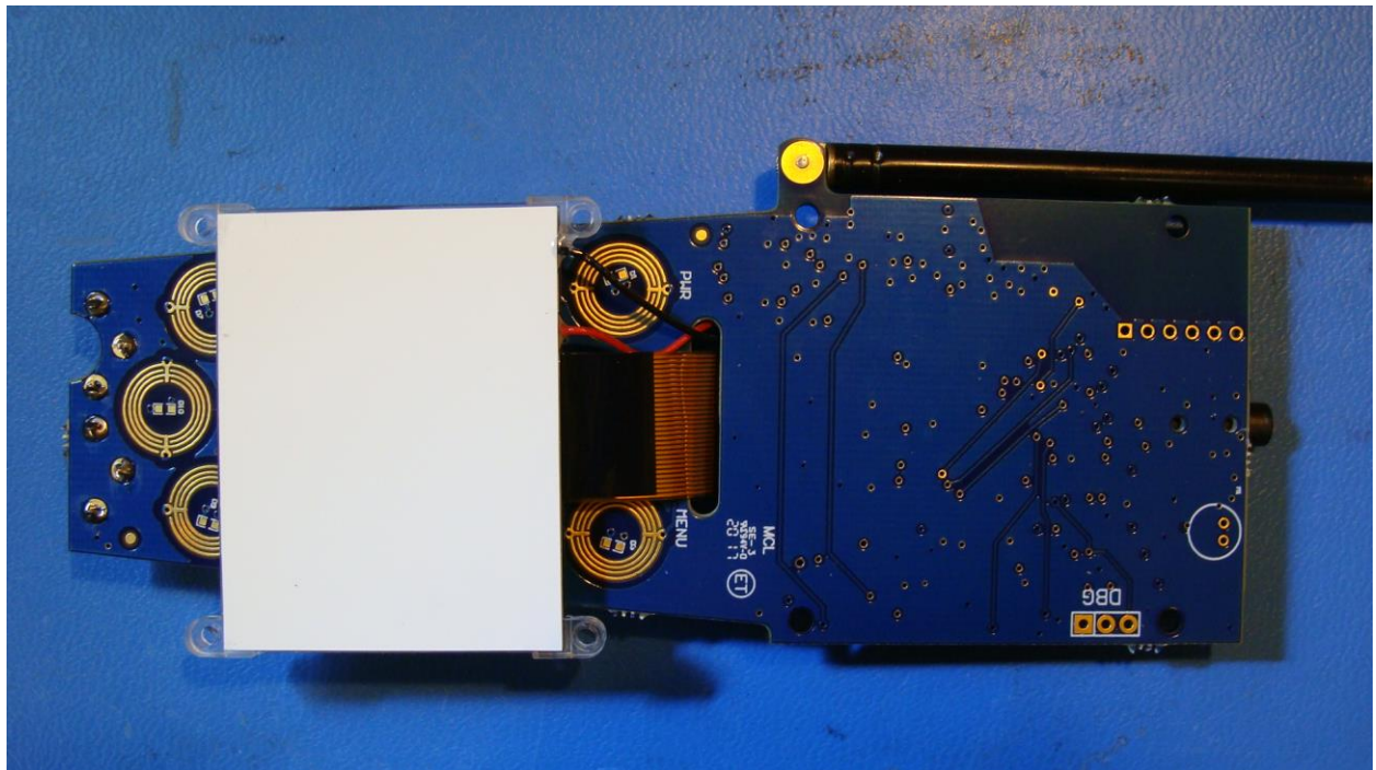
Photograph 2. PCB Front
