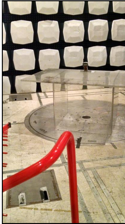
Photograph 1. Radiated Spurious Emissions, Test Setup, 30 MHz – 1 GHz
