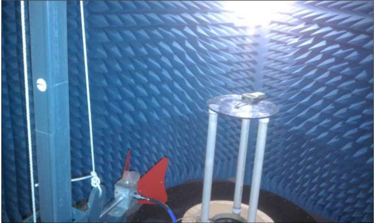
Photograph 3. Radiated Spurious Emissions, Test Setup, HF
