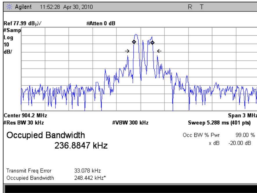
Plot 6. Occupied Bandwidth, IC Limits
