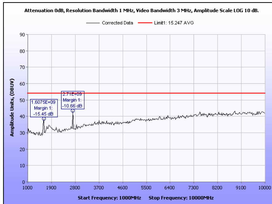
Plot 8. Radiated Spurious Emissions, 1 GHz – 10 GHz
