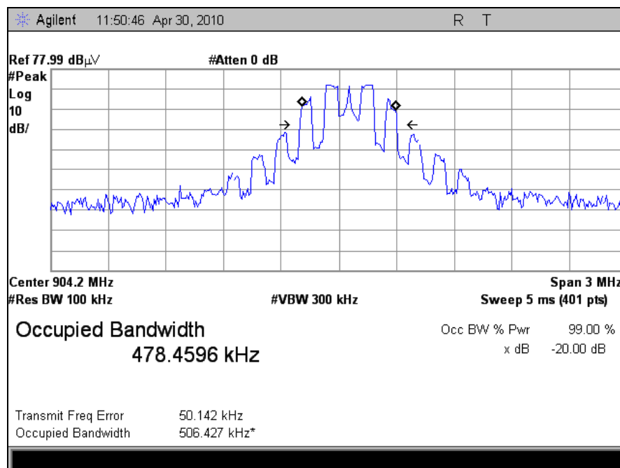
Plot 5. Occupied Bandwidth, FCC Limits
