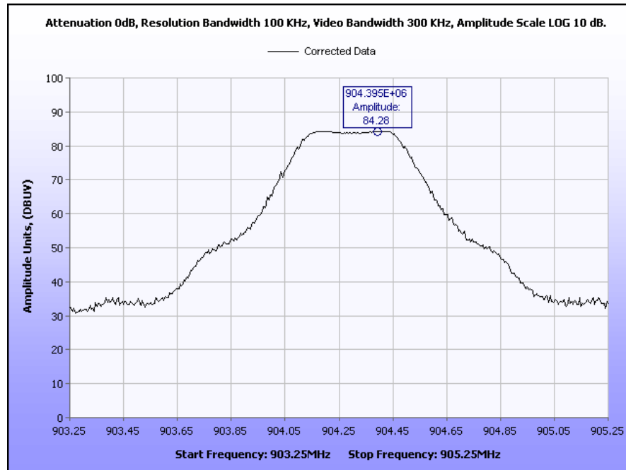
Plot 4. Fundamental Field Strength
