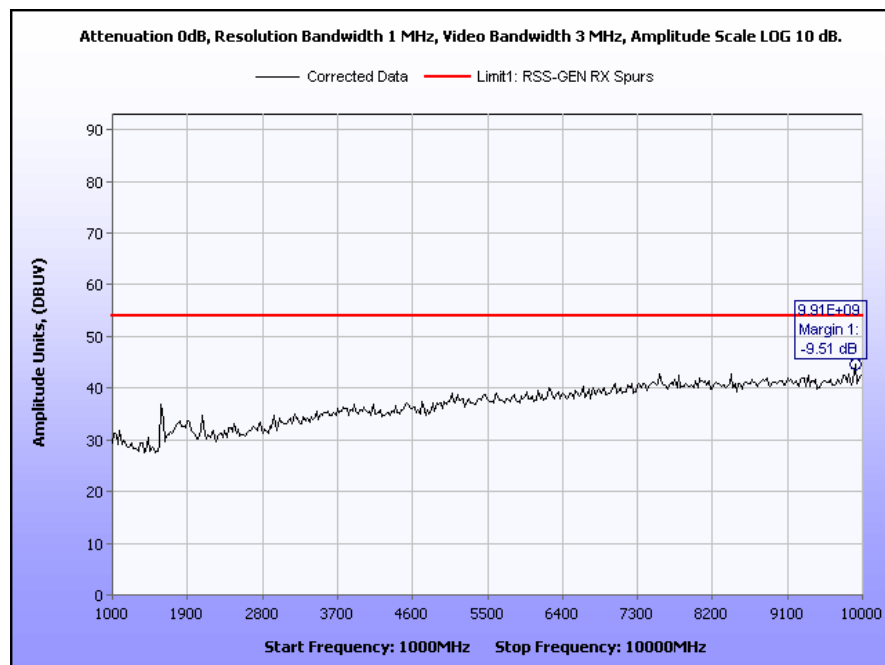
Plot 10. Receiver Spurious Emission, 1 GHz – 10 GHz
