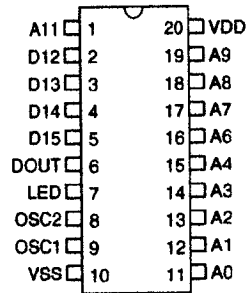
HT6207 - 20 DIP/SOP
