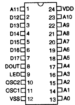
HT6247 - 24 SOP/SDIP
