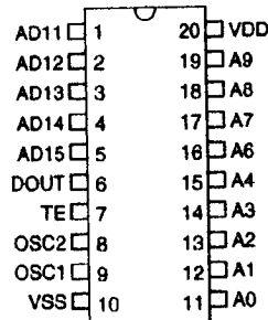
HT600 - 20 DIP/SOP
