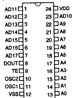
HT640 - 24 SOP/SDIP
