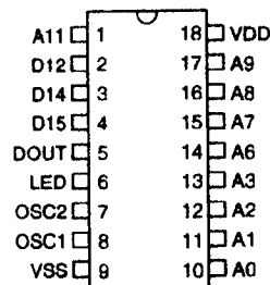
HT6187 - 18 DIP
