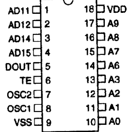
HT680 - 18 DIP/SOP
