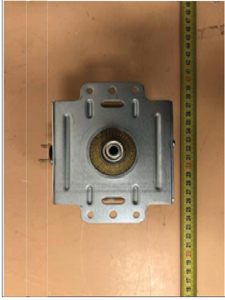
5. Rear View of Magnetron
