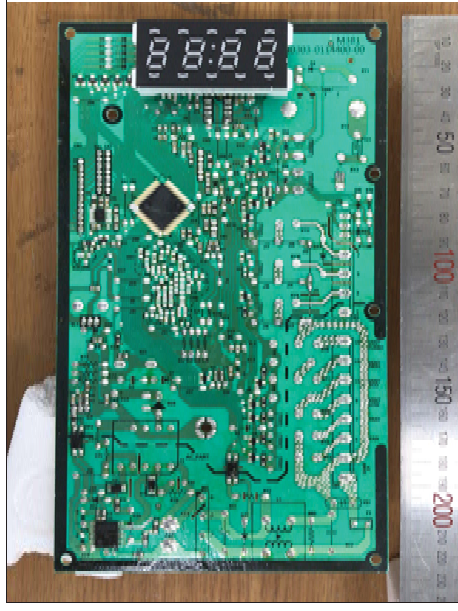
21. Rear View of Main Board
