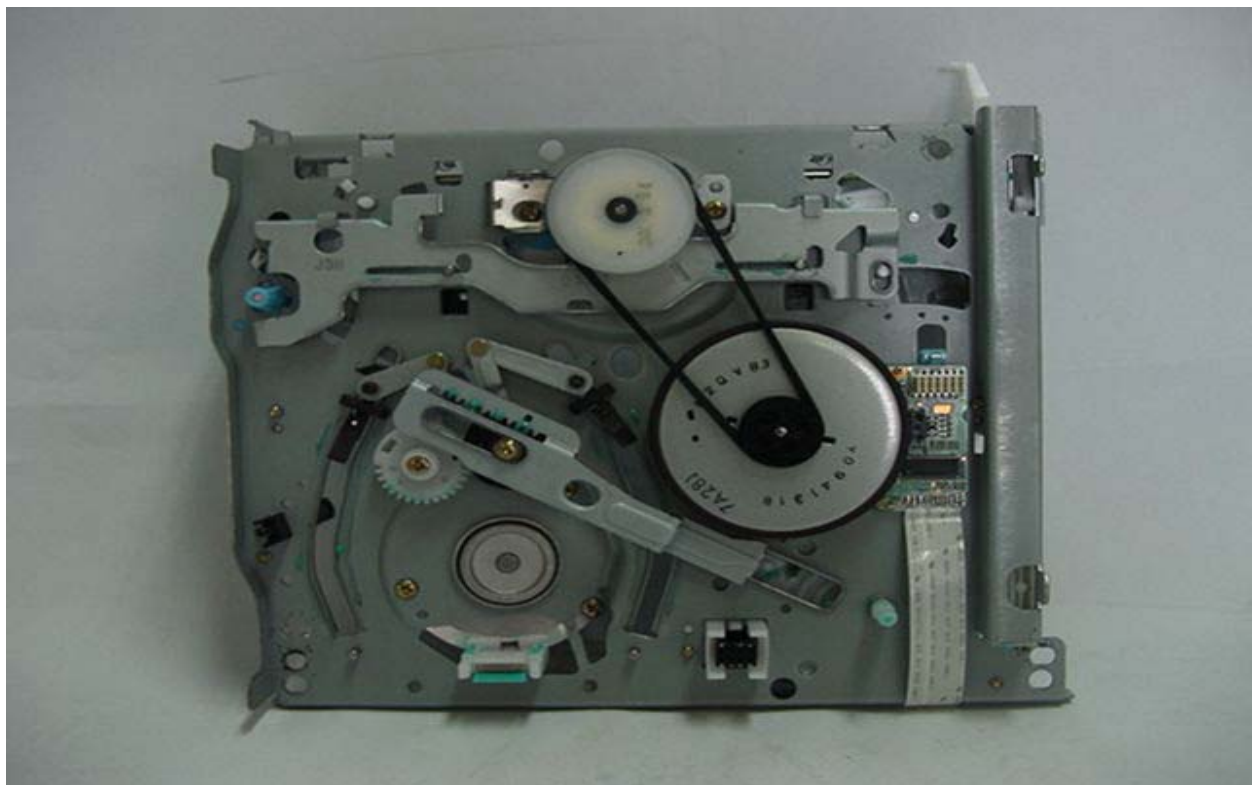
VCR Deck Bottom View
