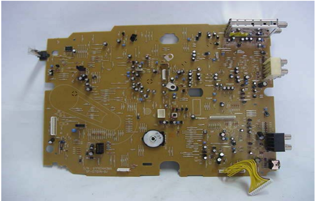
Main Board PCB Parts View
