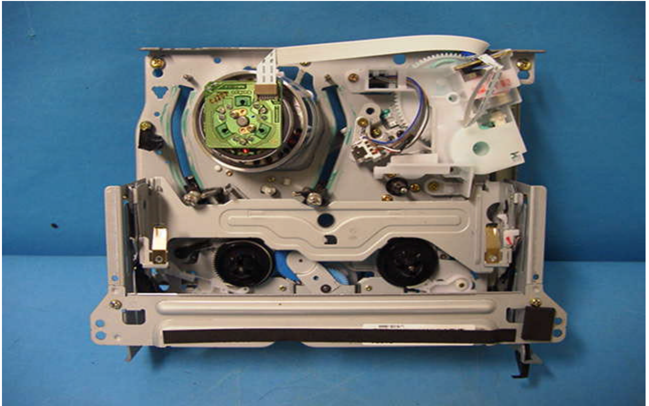
VCR Deck Top View
