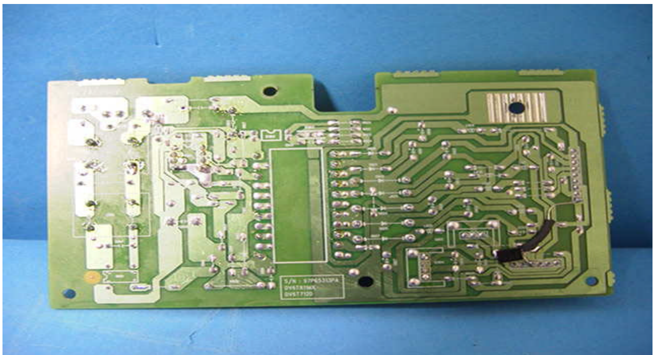
Power Board PCB Copper View
