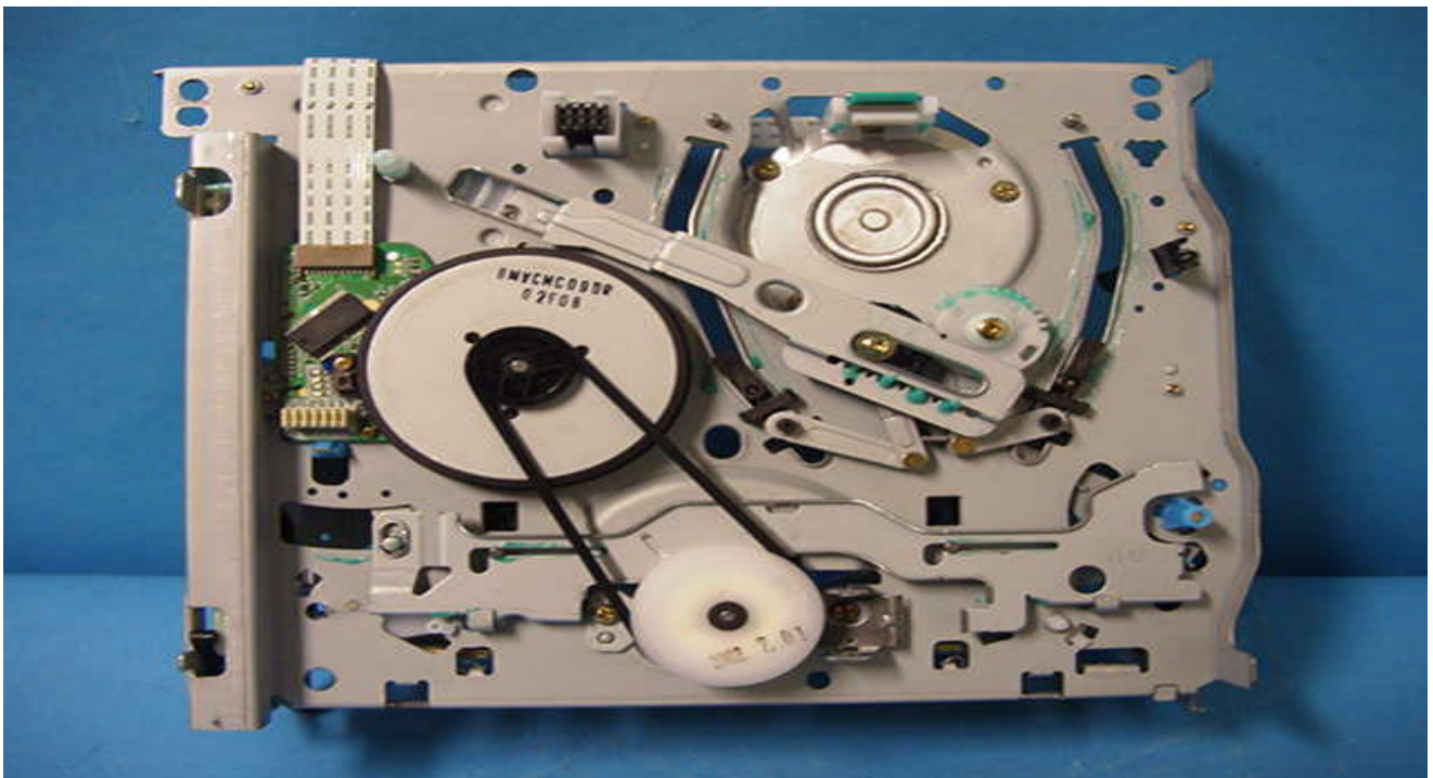
VCR Deck Bottom View
