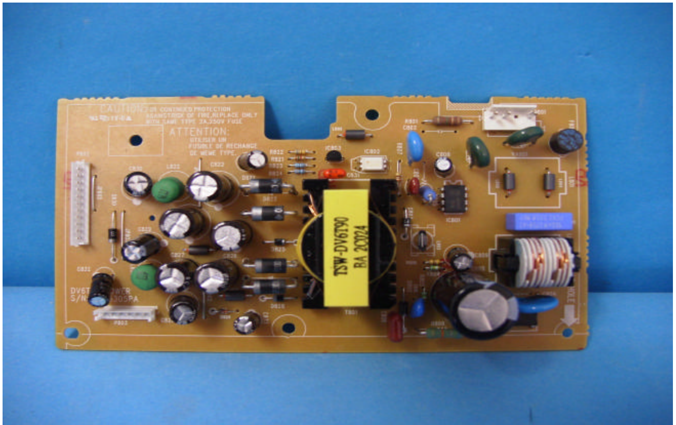
Power Board PCB Parts View
