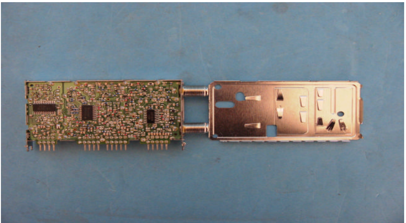
Rear View
