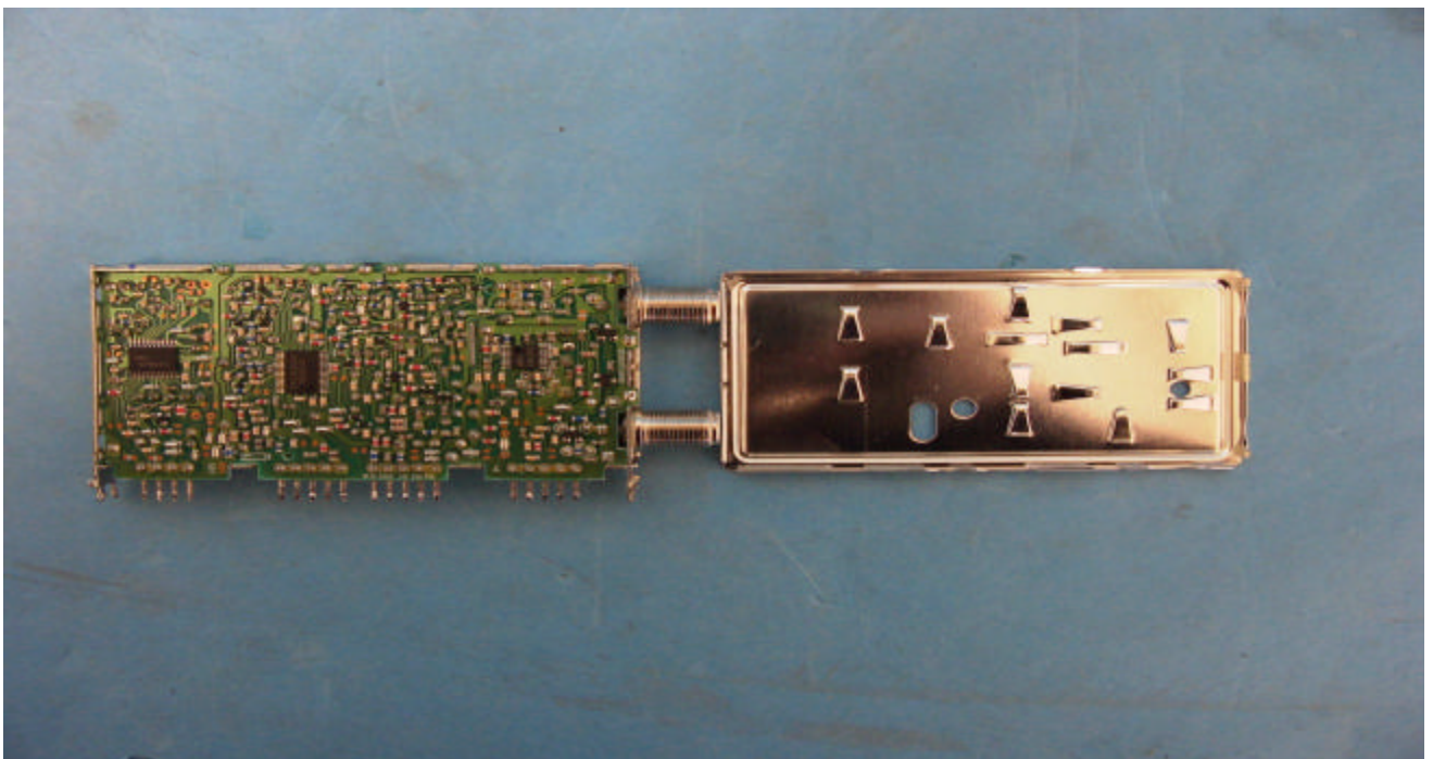
Inner View
