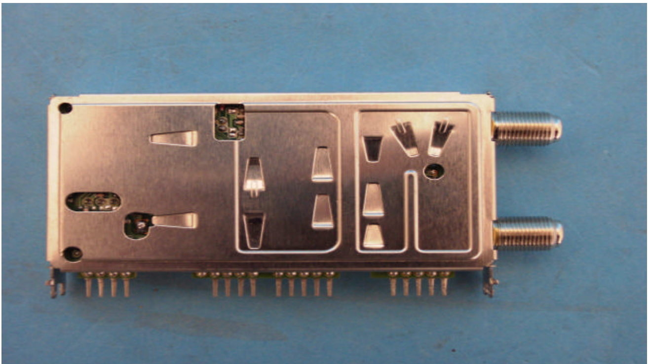
Rear View
