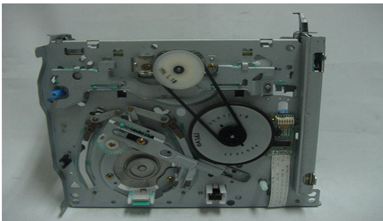
Deck Bottom View
