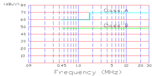
Fig. 11. Line-Conducted Limits
