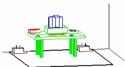
Figure 3. Line Conducted Emission Test Set-Up
