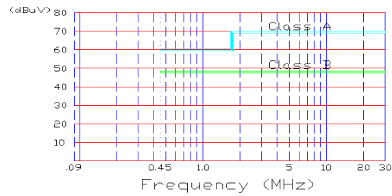
Fig. 11. Line-Conducted Limits
