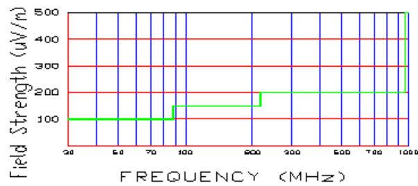
Fig. 12. FCC Class B Radiated Limits at 3 meters
