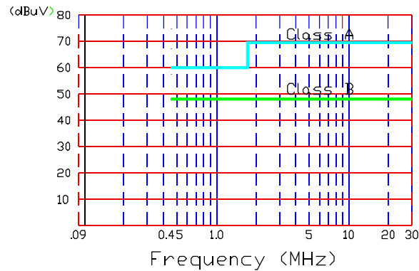
Fig. 11. Line-Conducted Limits
