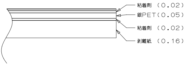
側面詳細 (SCALE 50/1)
