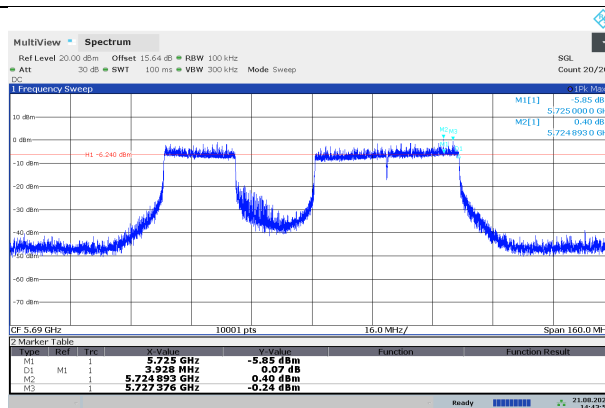
STRADDLE CHANNEL 138
