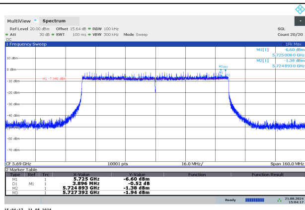
STRADDLE CHANNEL 138
