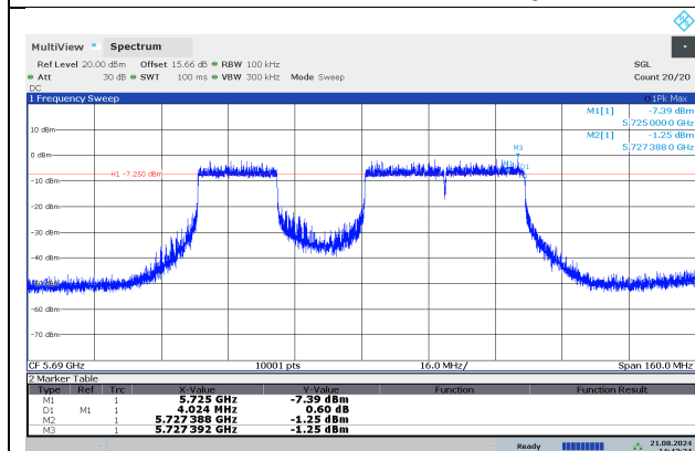
STRADDLE CHANNEL 138
