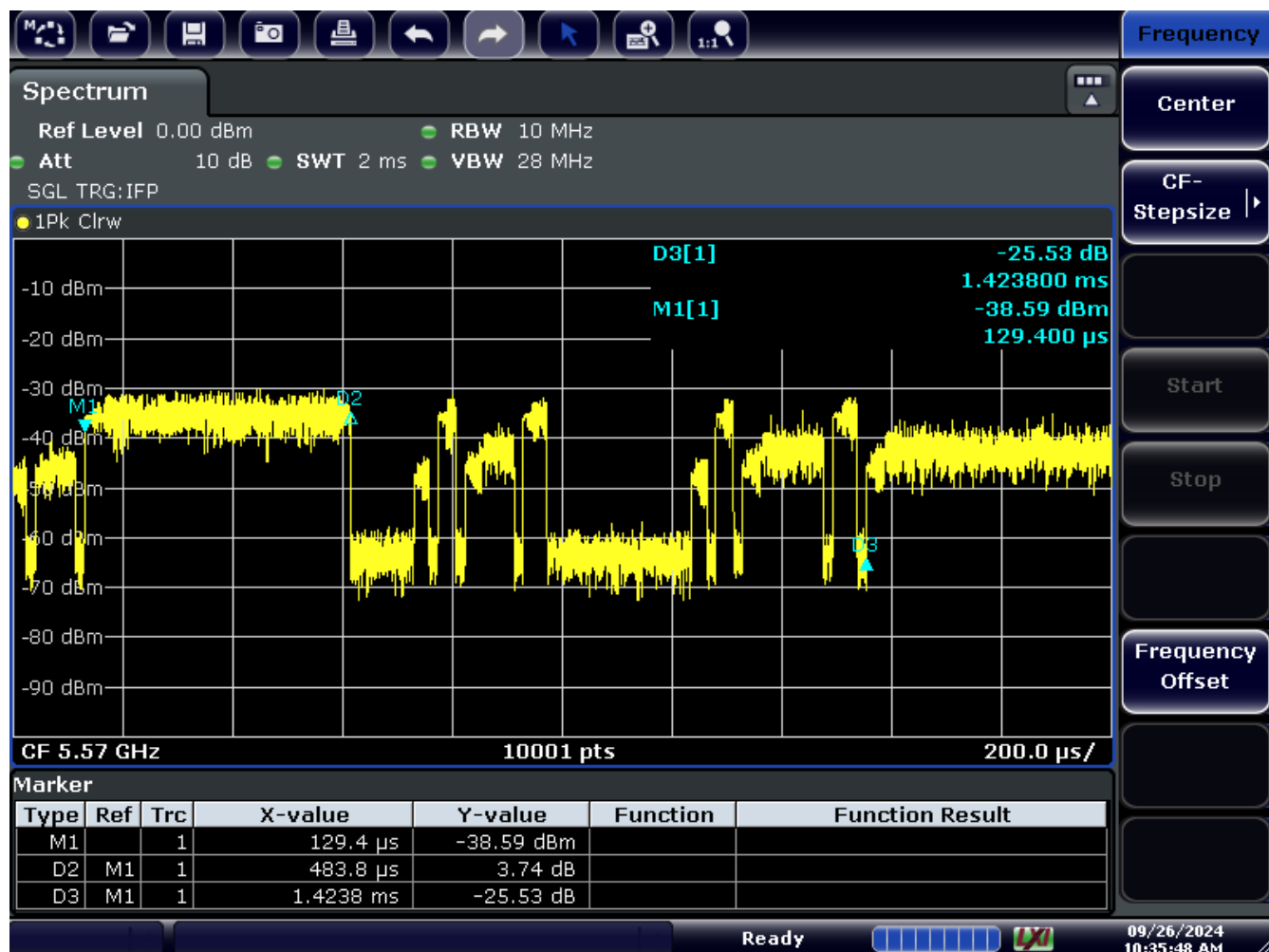
Figure 9-1. Band 2C Channel Loading
