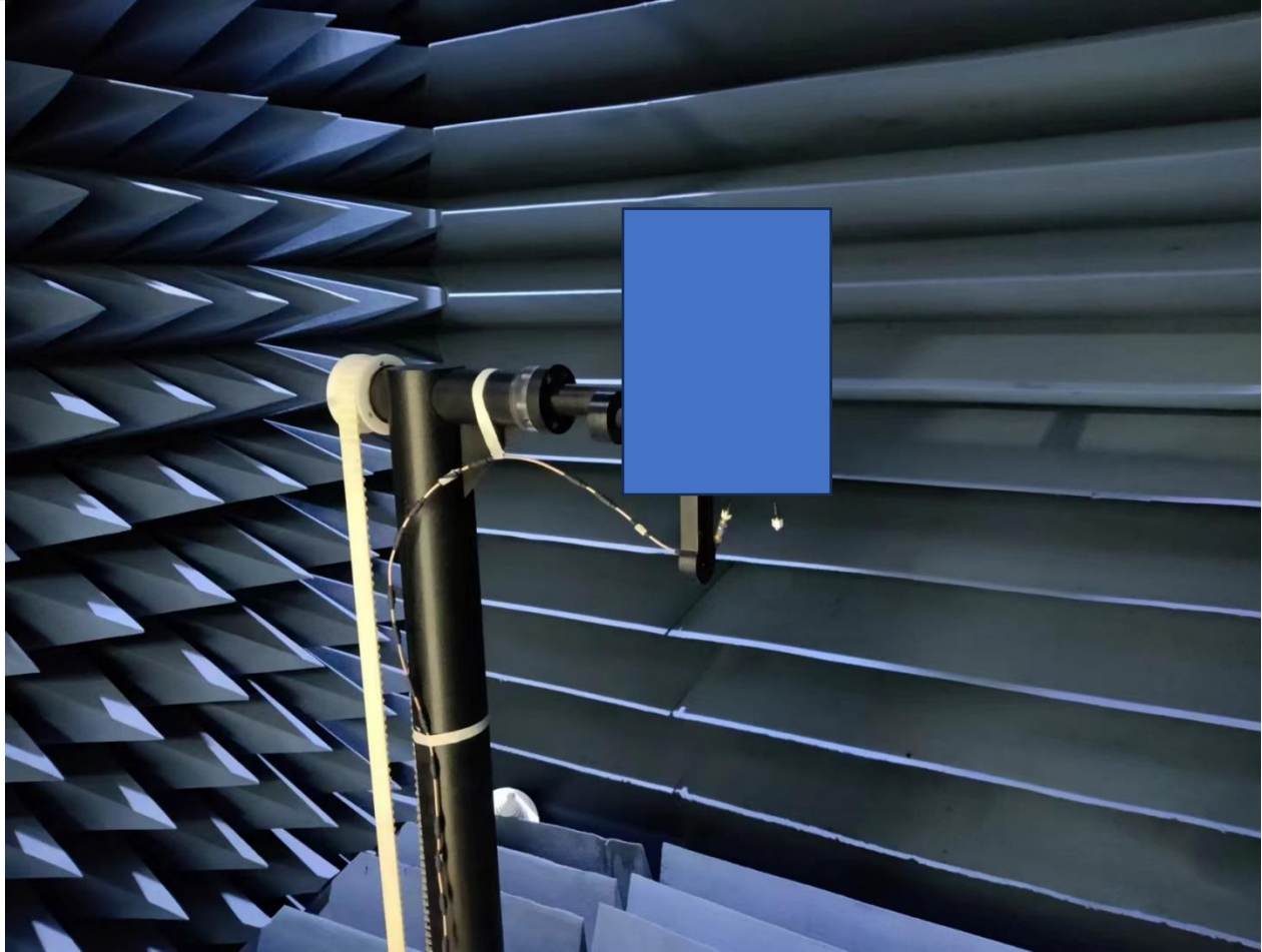
WiFi setup photo
