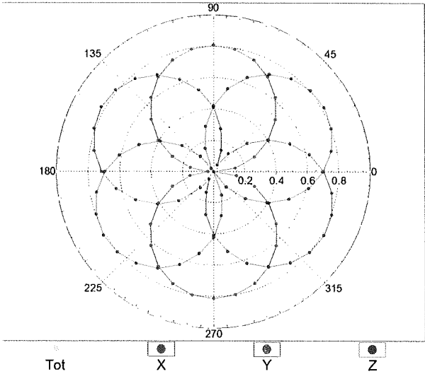
f=600 MHz,TEM
