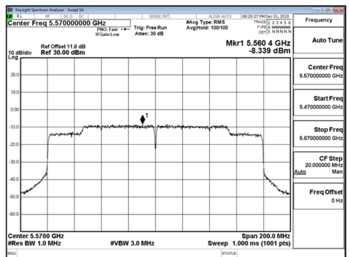
802.11ax_160MHz_5570MHz-5570
