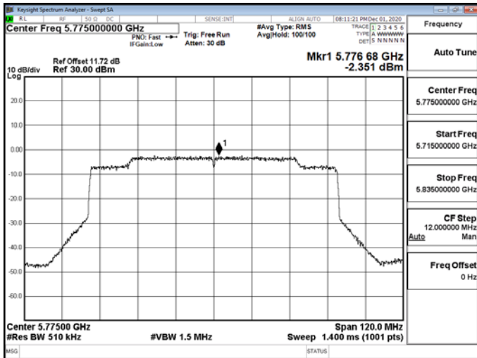
802.11ax_80MHz_RU_484_66_5775MHz-5775
