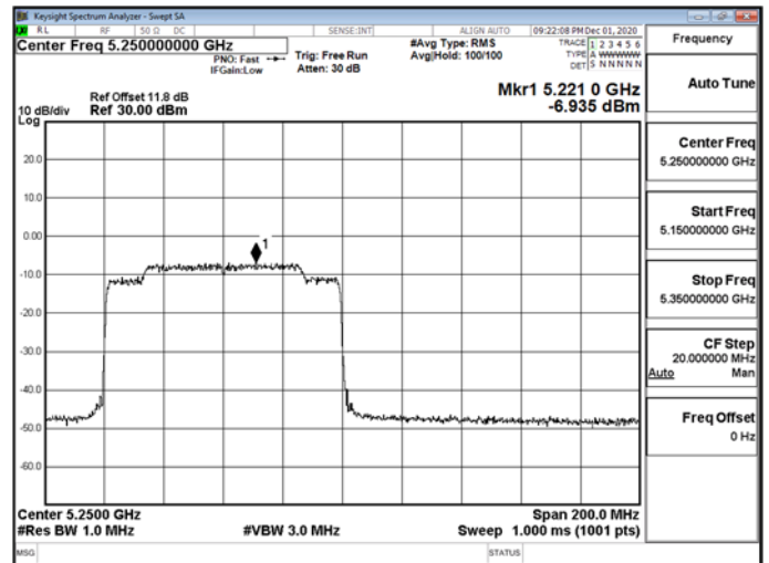
802.11ax_160MHz_RU_996_S67_5250MHz-5250
