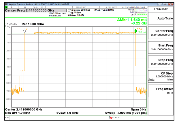
PULSE WIDTH – 2DH3
