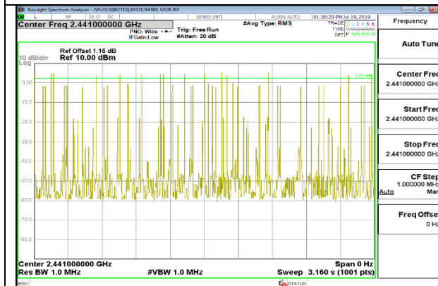
NUMBER OF PULSES IN 3.16 SECOND OBSERVATION PERIOD – 2DH3
