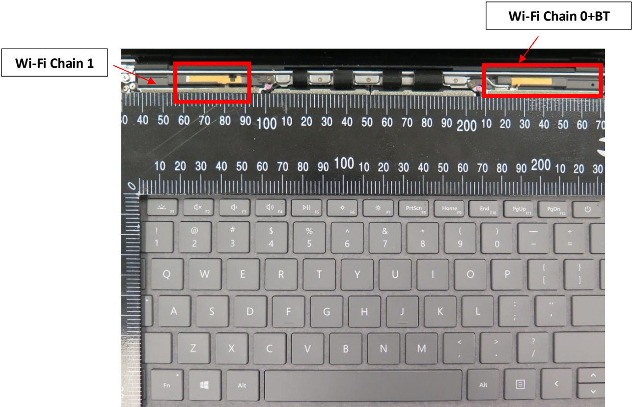
Figure 7 Wi-Fi/BT Chain 0 & 1 Antenna View
