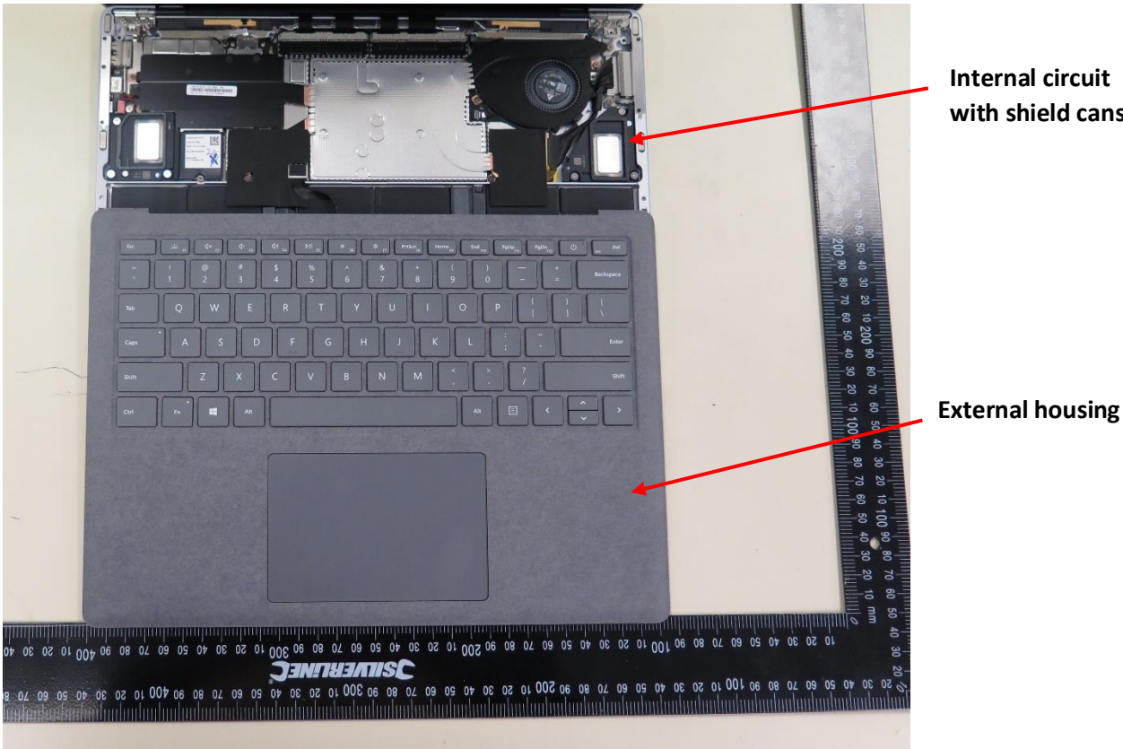
Figure 1 EUT with external housing off- showing main logic board
