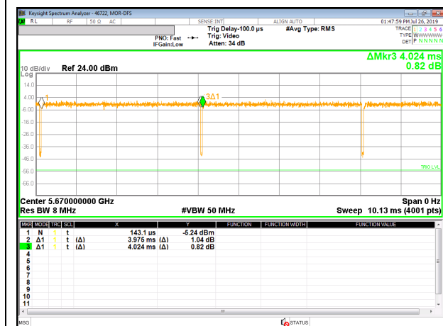
DUTY CYCLE 802.11n HT40 SDM MODE
