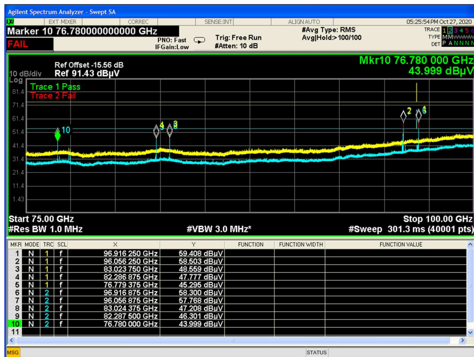
Figure 9-18. Radiated Spurious Emissions 24.2 GHz SRD_Pre Scan_Horizontal_(75-100 GHz)
