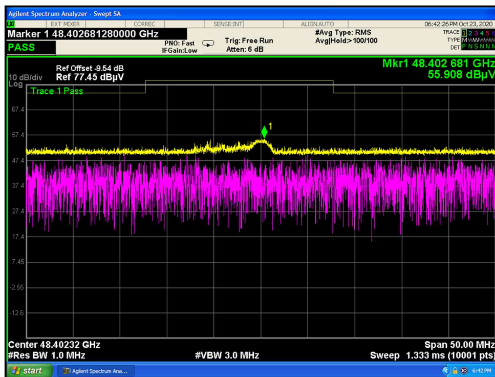
Figure 9-12. Radiated Spurious Emissions 24.2 GHz SRD_Veritical_(40 - 60 GHz)_Peak
