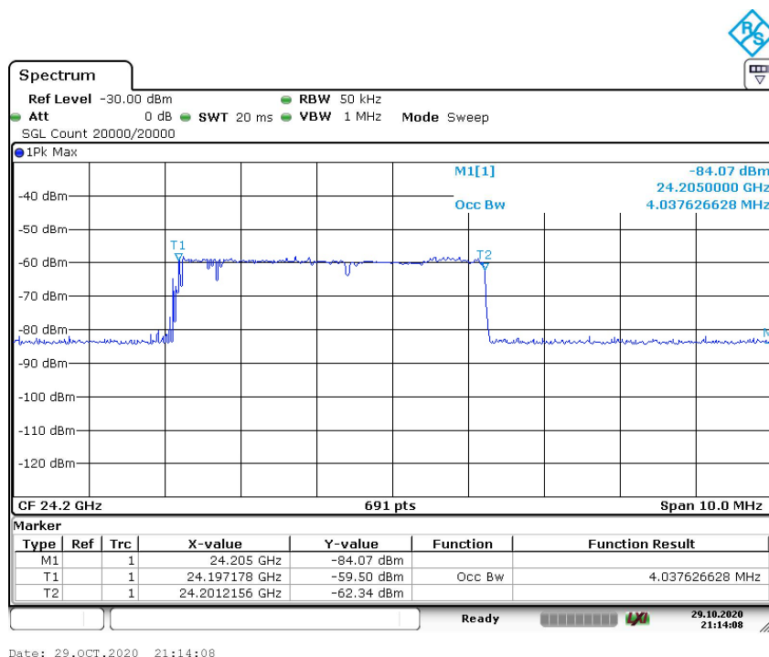
Figure 9-2. Occupied Bandwidth 24.2 GHz
