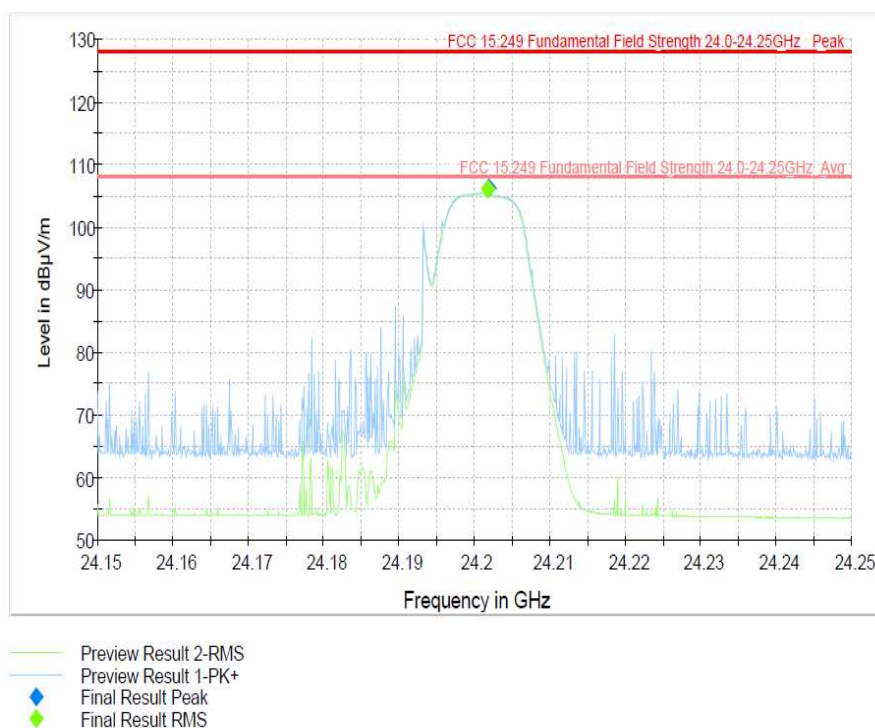
Figure 9-4. Peak Fundamental Field Strength 24.2 GHz
