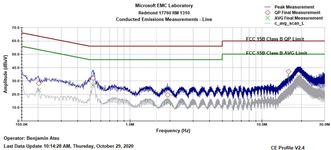
Figure 9-20 AC Line Conducted Emissions- Line (150 kHz- 30 MHz)
