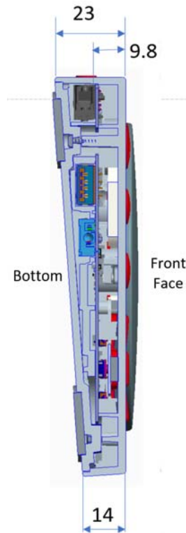
Left Edge View Showing Separation Distance from PCB which the Antennas are on to Bottom and Front Face.
