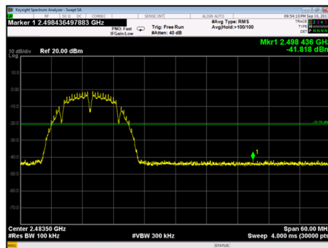
Plot 9-219 Chain B Conducted Band Edge 802.11b - Ch. 12 (2467 MHz)
