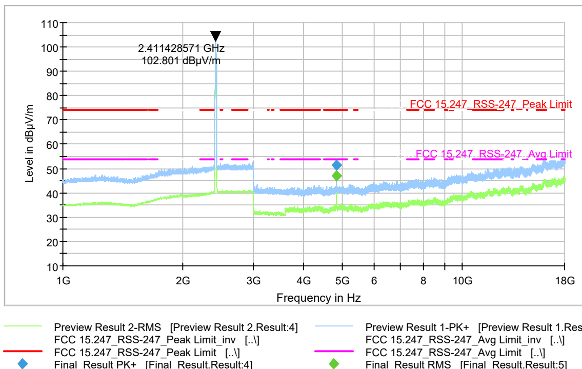
Plot 9-232 Radiated Spurious Emission 1-18GHz 802.11b - Ch.1 (2412 MHz)
