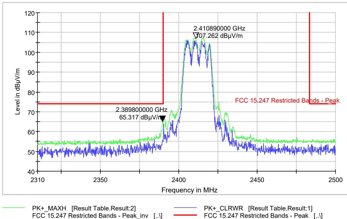
Plot 9-250 Radiated Band Edge Peak 802.11g - Ch.1 (2412 MHz)
