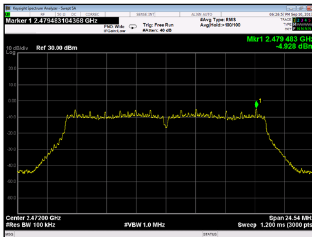
Plot 9-187 Chain B Reference Level 802.11g - Ch.13 (2472 MHz)
