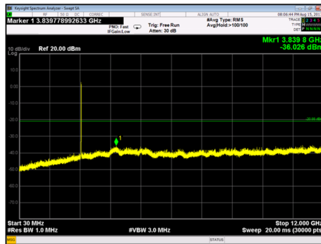
Plot 9-167 Chain B Conducted Spurious Emissions 3 0MHz - 12 GHz 802.11b - Ch.11 (2462 MHz)
