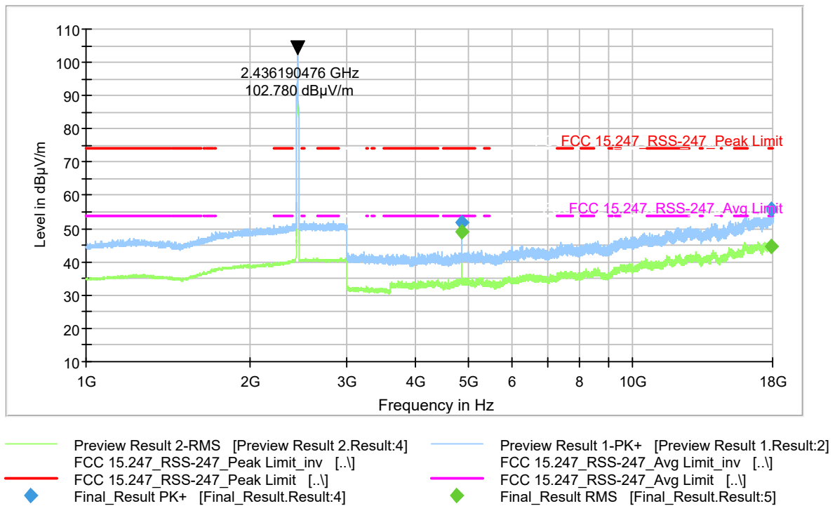
Plot 9-233 Radiated Spurious Emission 1-18GHz 802.11b - Ch.6 (2437 MHz)
