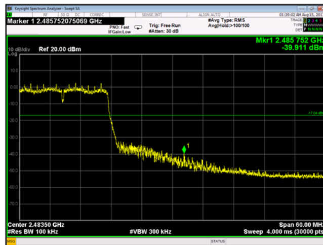
Plot 9-214 Chain A Conducted Band Edge 802.11n - Ch. 11 (2462 MHz)
