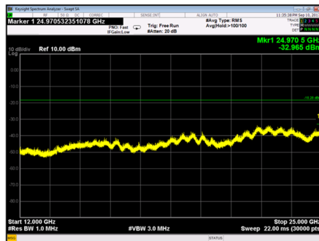
Plot 9-198 Chain B Conducted Spurious Emissions 12 - 25 GHz 802.11n - Ch.11 (2462 MHz)
