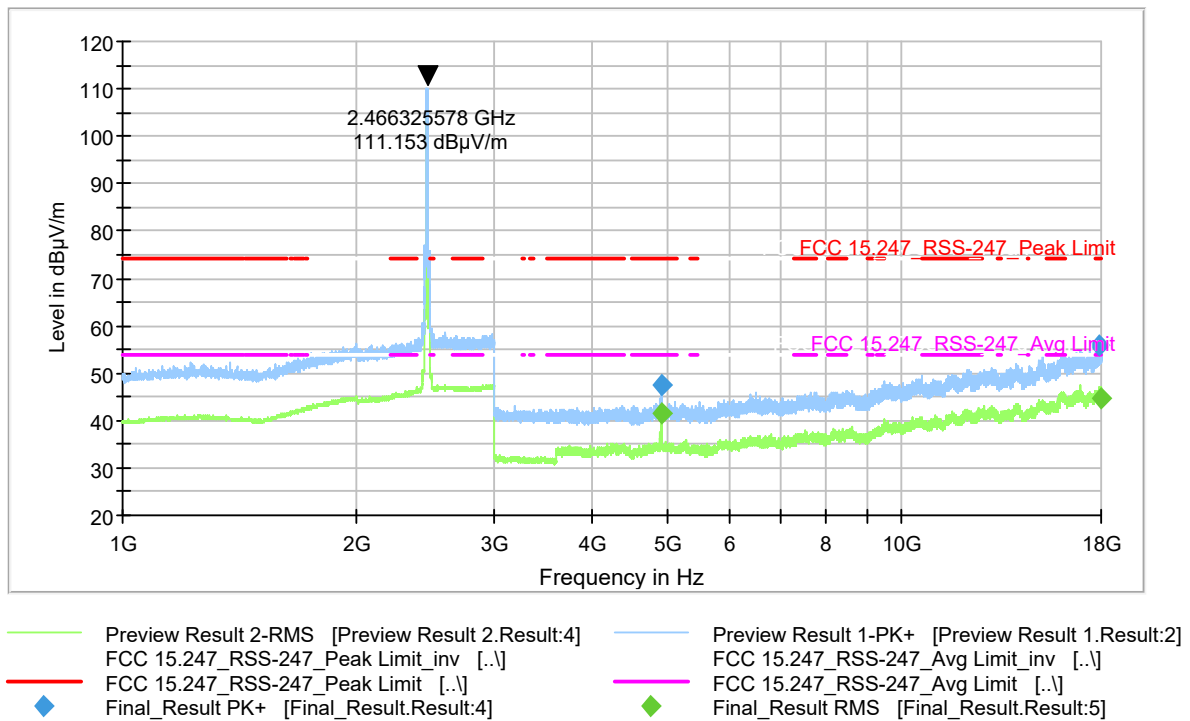
Plot 9-238 Radiated Spurious Emission 1-18GHz 802.11g - Ch.10 (2457 MHz)
