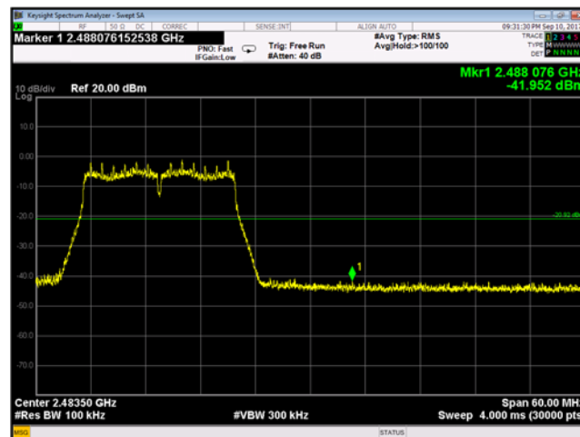
Plot 9-211 Chain A Conducted Band Edge 802.11g - Ch. 12 (2467 MHz)
