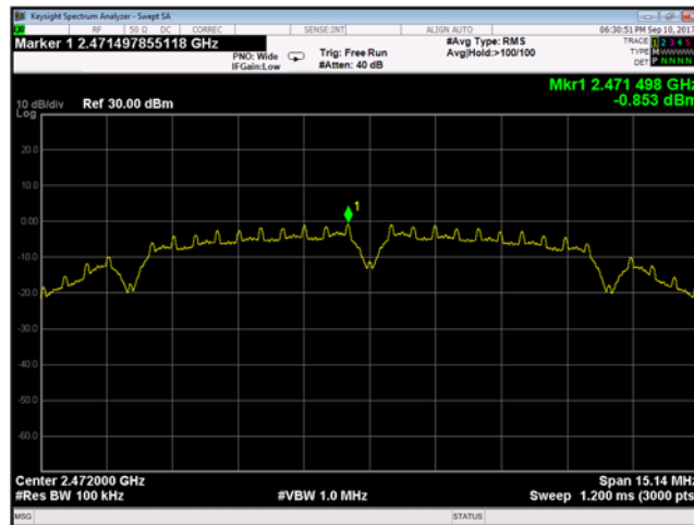
Plot 9-172 Chain B Reference Level 802.11b - Ch.13 (2472 MHz)
