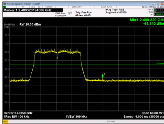
Plot 9-228 Chain B Conducted Band Edge 802.11n - Ch. 13 (2472 MHz)
