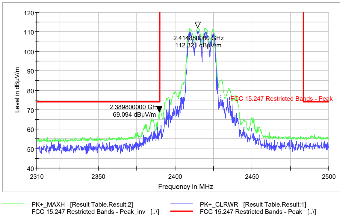
Figure 9-258 Radiated Band Edge Peak 802.11n - Ch.2 (2417 MHz)
