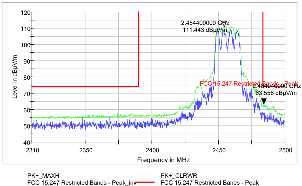
Figure 9-264 Radiated Band Edge Peak 802.11n - Ch.10 (2457 MHz)
