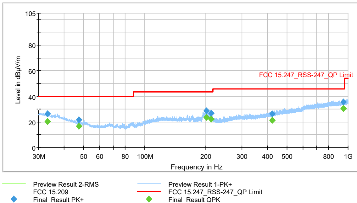
Plot 9-229 Radiated Spurious Emissions 30 – 1000 MHz 802.11b - Ch. 6 (2437 MHz)
