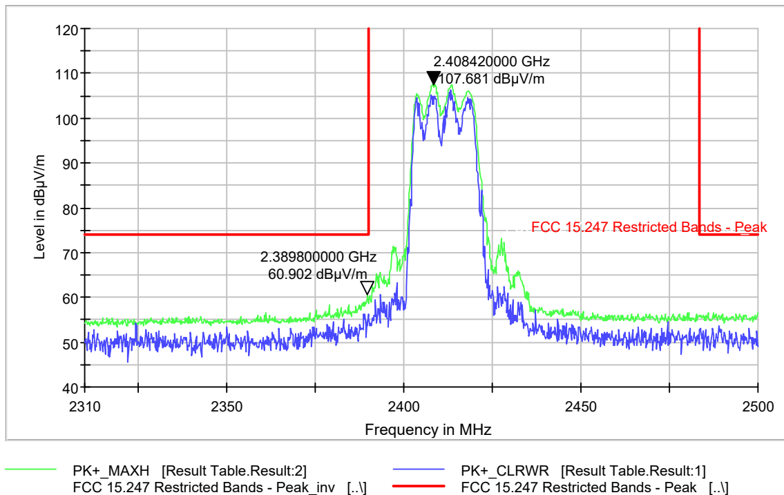
Plot 9-252 Radiated Band Edge Peak 802.11n - Ch.1 (2412 MHz)
