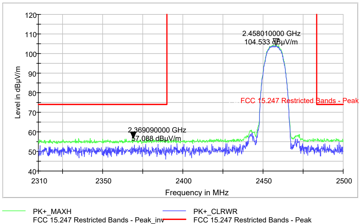
Figure 9-260 Radiated Band Edge Peak 802.11b - Ch.10 (2457 MHz)
