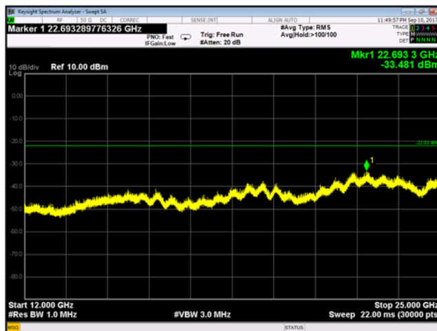
Plot 9-186 Chain B Conducted Spurious Emissions 12 - 25 GHz 802.11g - Ch.12 (2467 MHz)
