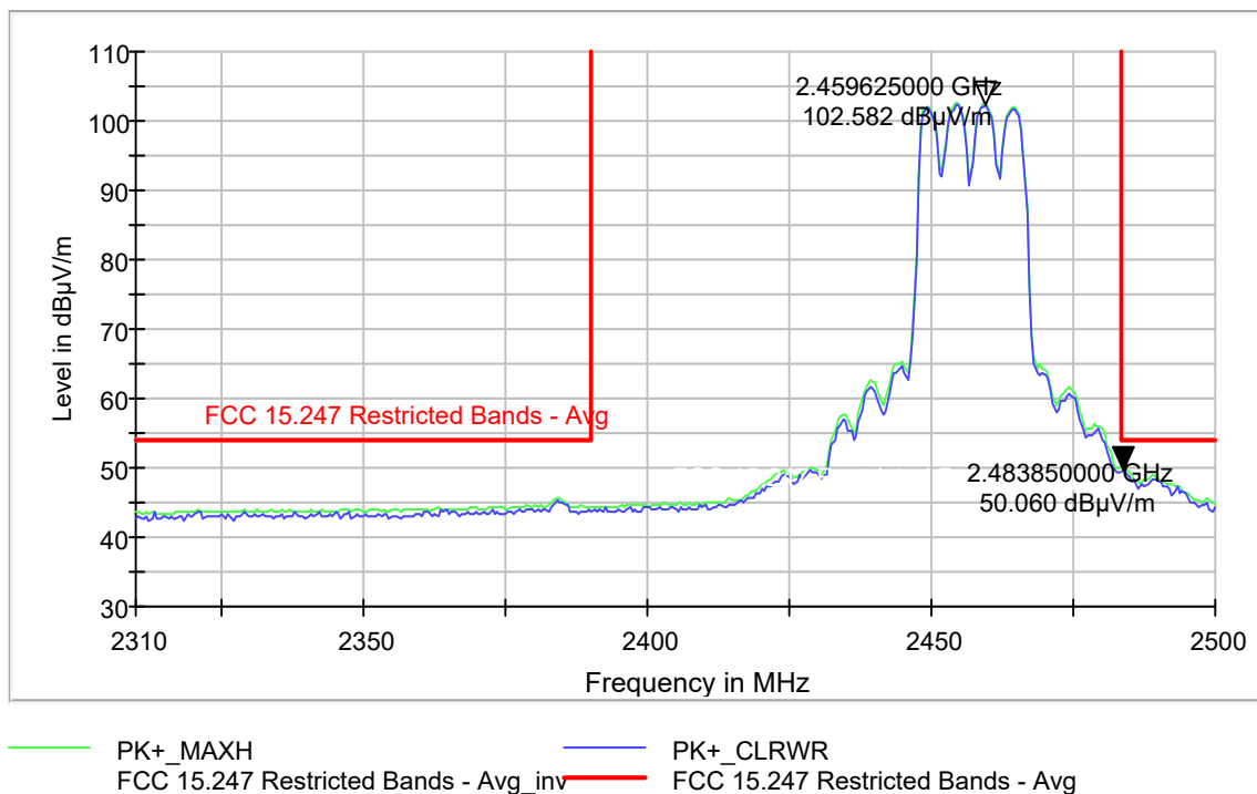
Figure 9-265 Radiated Band Edge Average 802.11n - Ch.10 (2457 MHz)
