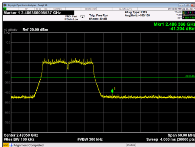
Plot 9-224 Chain B Conducted Band Edge 802.11g - Ch. 13 (2472 MHz)
