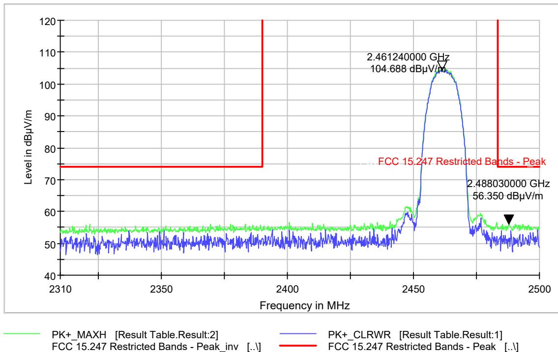
Plot 9-266 Radiated Band Edge Peak 802.11b - Ch.11 (2462 MHz)
