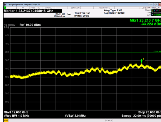
Plot 9-168 Chain B Conducted Spurious Emissions 12 - 25 GHz 802.11b - Ch.11 (2462 MHz)
