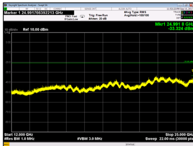
Plot 9-174 Chain B Conducted Spurious Emissions 12 - 25 GHz 802.11b - Ch.13 (2472 MHz)
