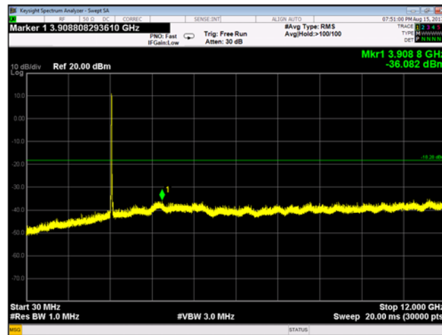
Plot 9-197 Chain B Conducted Spurious Emissions 30 MHz - 12 GHz 802.11n - Ch.11 (2462 MHz)
