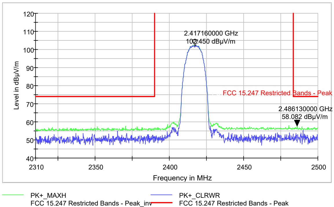
Figure 9-254 Radiated Band Edge Peak 802.11b - Ch.2 (2417 MHz)
