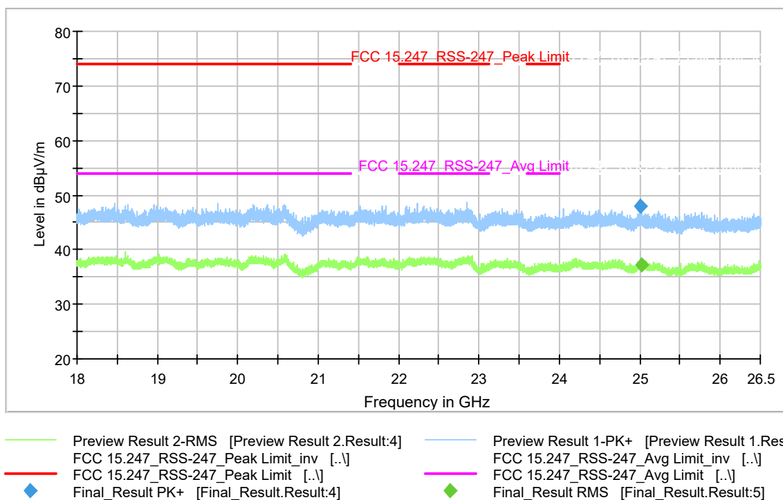
Plot 9-247 Radiated Spurious Emissions 18-26.5GHz 802.11g - Ch.10 (2457 MHz)
