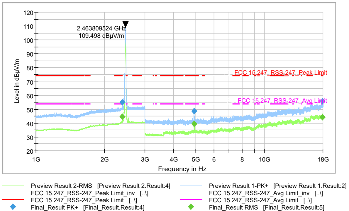
Plot 9-244 Radiated Spurious Emission 1-18GHz 802.11n - Ch.12 (2467 MHz)
