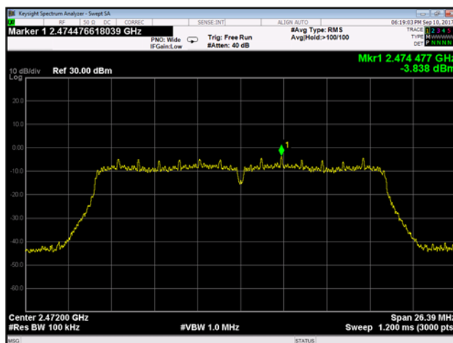
Plot 9-157 Chain A Reference Level 802.11n - Ch.13 (2472 MHz)
