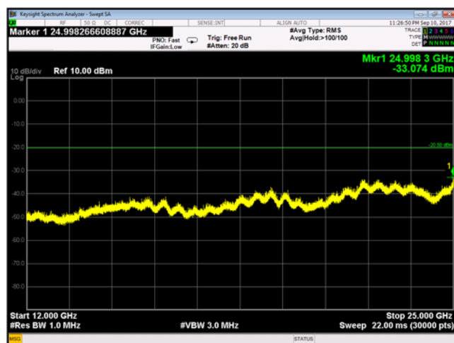
Plot 9-177 Chain B Conducted Spurious Emissions 12 - 25 GHz 802.11g - Ch.1 (2412 MHz)
