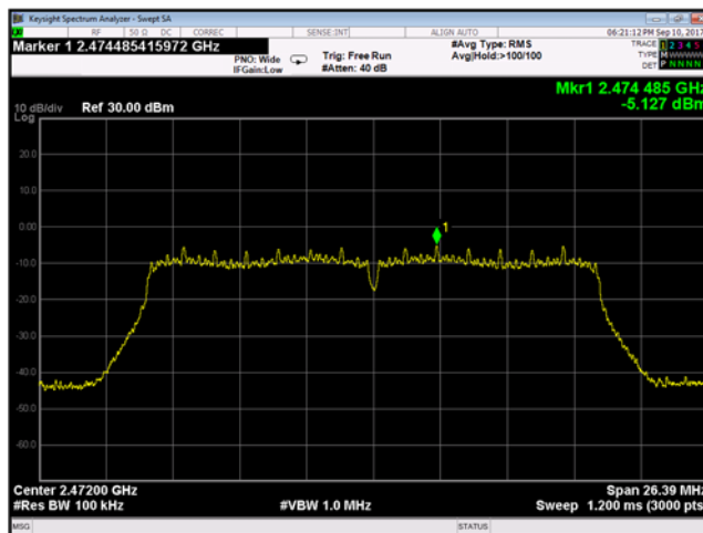
Plot 9-202 Chain B Reference Level 802.11n - Ch.13 (2472 MHz)
