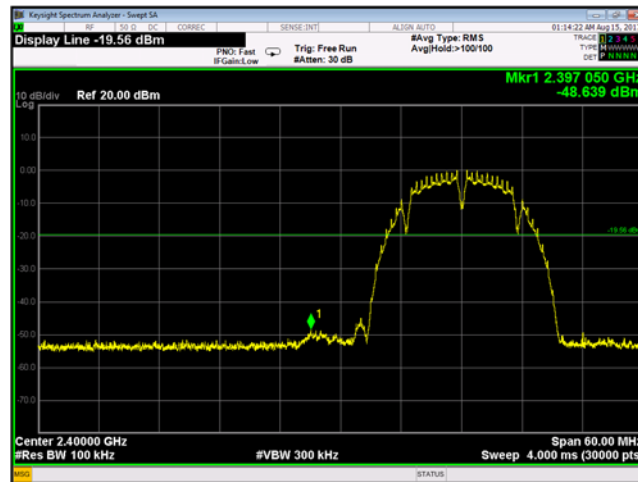
Plot 9-217 Chain B Conducted Band Edge 802.11b - Ch. 1 (2412 MHz)
