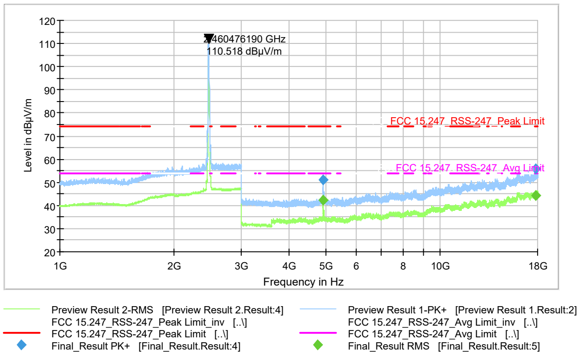
Plot 9-239 Radiated Spurious Emission 1-18GHz 802.11g - Ch.11 (2462 MHz)
