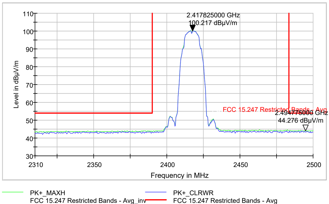
Figure 9-255 Radiated Band Edge Average 802.11b - Ch.2 (2417 MHz)
