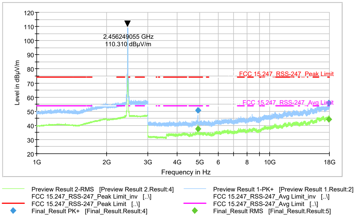
Plot 9-243 Radiated Spurious Emission 1-18GHz 802.11n - Ch.10 (2457 MHz)
