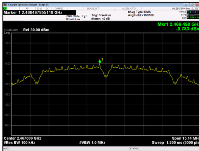
Plot 9-169 Chain B Reference Level 802.11b - Ch.12 (2467 MHz)
