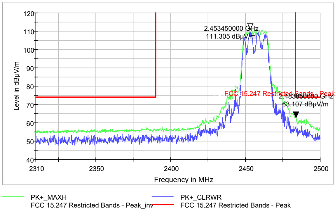
Figure 9-262 Radiated Band Edge Peak 802.11g - Ch.10 (2457 MHz)
