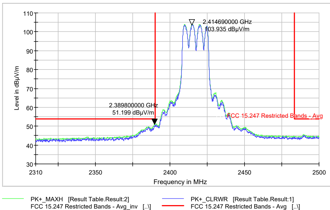
Figure 9-257 Radiated Band Edge Average 802.11g - Ch.2 (2417 MHz)
