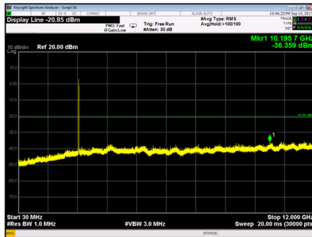
Plot 9-173 Chain B Conducted Spurious Emissions 30 MHz - 12 GHz 802.11b - Ch.13 (2472 MHz)
