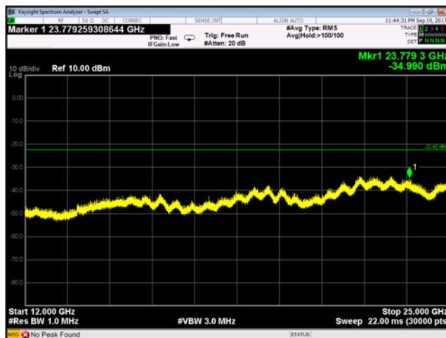
Plot 9-201 Chain B Conducted Spurious Emissions 12 - 25 GHz 802.11n - Ch.12 (2467 MHz)
