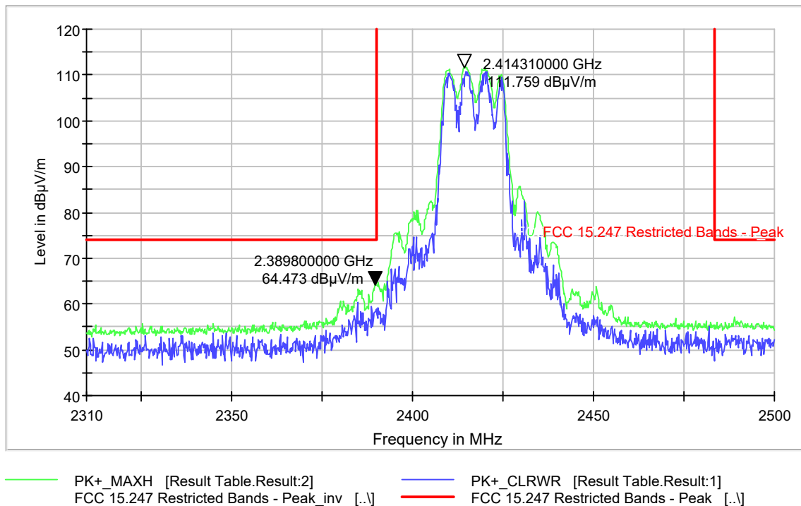
Figure 9-256 Radiated Band Edge Peak 802.11g - Ch.2 (2417 MHz)
