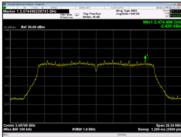
Plot 9-199 Chain B Reference Level 802.11n - Ch.12 (2467 MHz)
