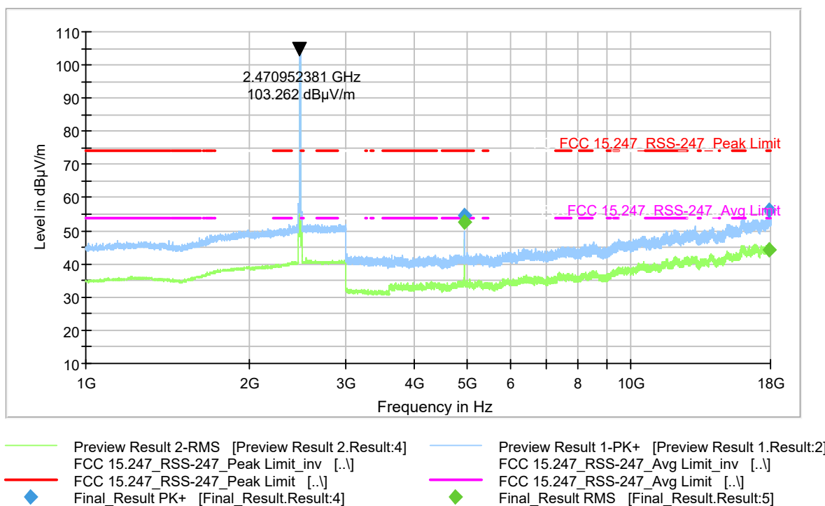
Plot 9-235 Radiated Spurious Emission 1-18GHz 802.11b - Ch.13 (2472 MHz)
