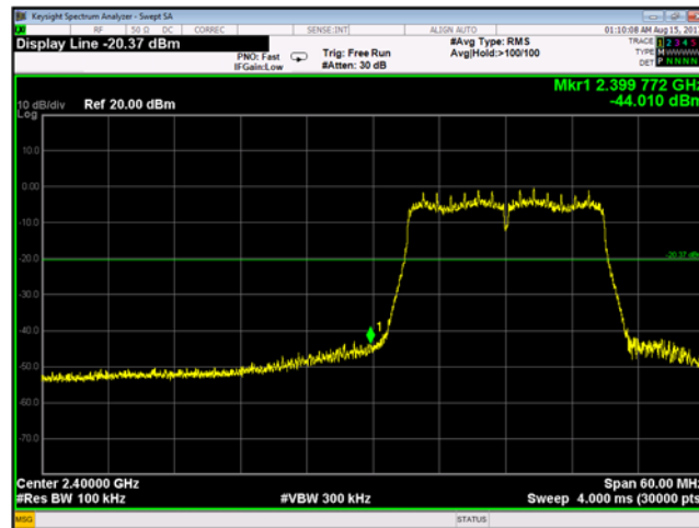
Plot 9-213 Chain A Conducted Band Edge 802.11n - Ch. 1 (2412 MHz)
