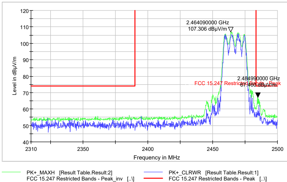
Plot 9-274 Radiated Band Edge Peak 802.11g - Ch.12 (2467 MHz)
