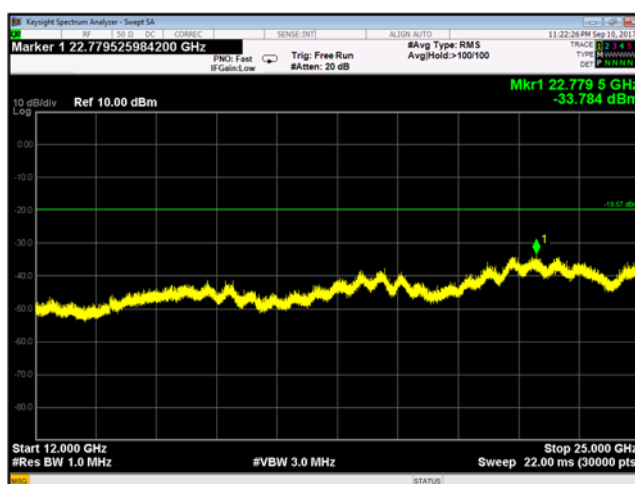
Plot 9-165 Chain B Conducted Spurious Emissions 12 - 25 GHz 802.11b - Ch.6 (2437 MHz)
