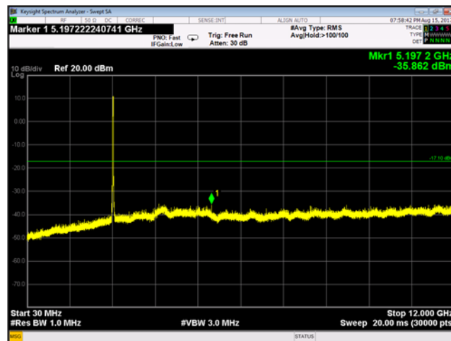
Plot 9-179 Chain B Conducted Spurious Emissions 30 MHz - 12 GHz 802.11g - Ch.6 (2437 MHz)
