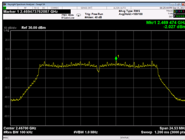
Plot 9-184 Chain B Reference Level 802.11g - Ch.12 (2467 MHz)
