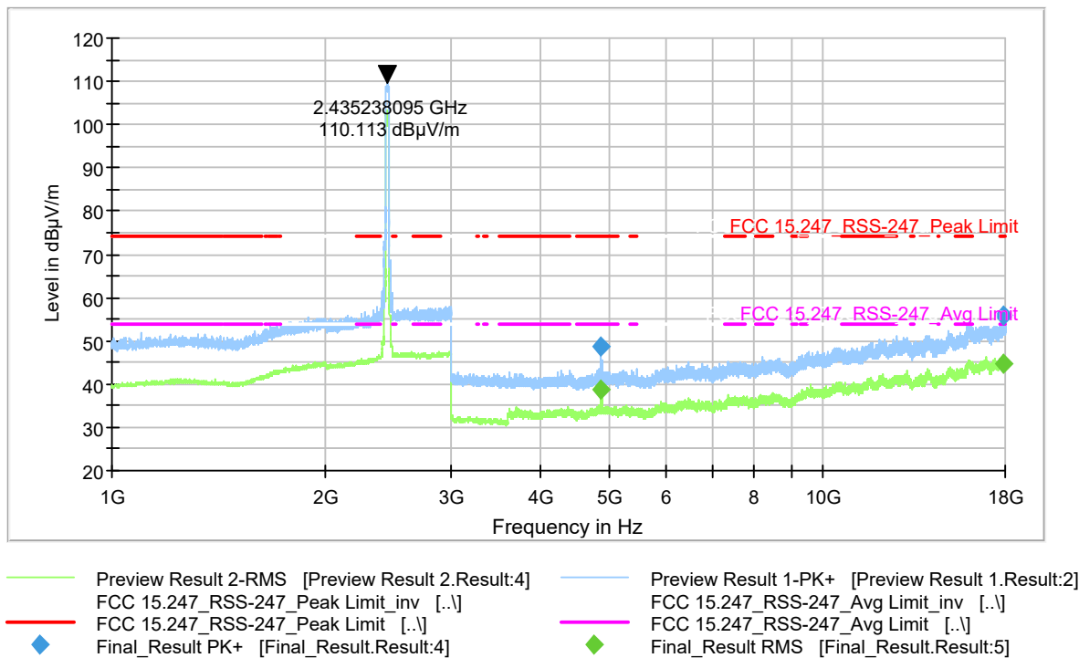
Plot 9-242 Radiated Spurious Emission 1-18GHz 802.11n - Ch.6 (2437 MHz)
