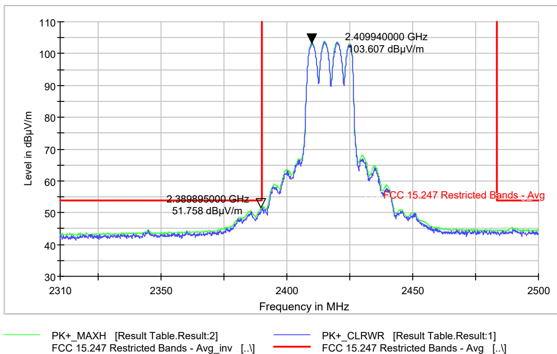
Figure 9-259 Radiated Band Edge Average 802.11n - Ch.2 (2417 MHz)
