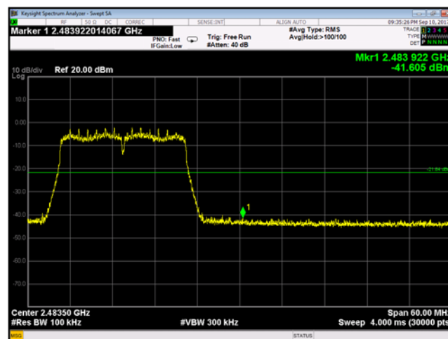
Plot 9-215 Chain A Conducted Band Edge 802.11n - Ch. 12 (2467 MHz)
