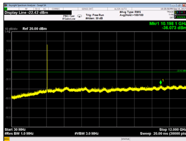
Plot 9-200 Chain B Conducted Spurious Emissions 30 MHz - 12 GHz 802.11n - Ch.12 (2467 MHz)
