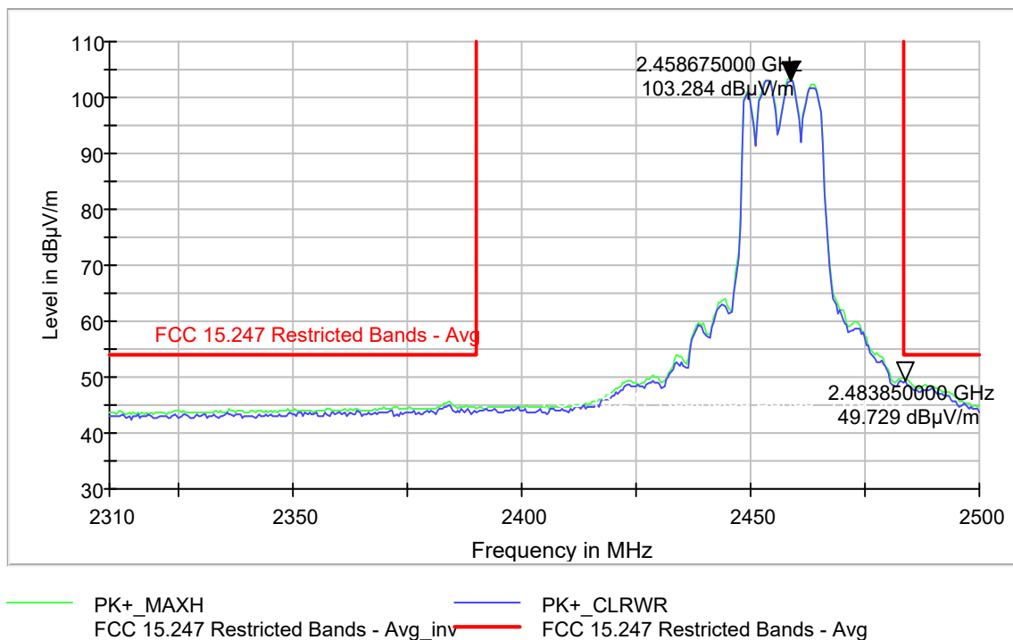
Figure 9-263 Radiated Band Edge Average 802.11g - Ch.10 (2457 MHz)
