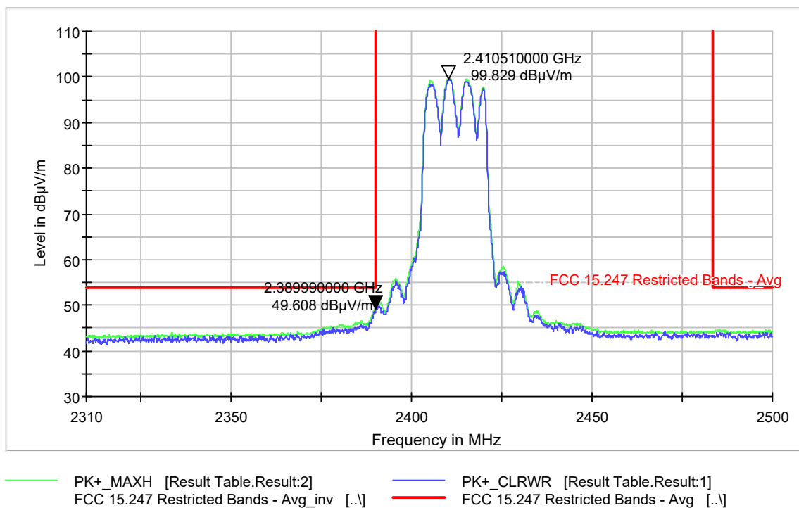
Plot 9-251 Radiated Band Edge Average 802.11g - Ch.1 (2412 MHz)
