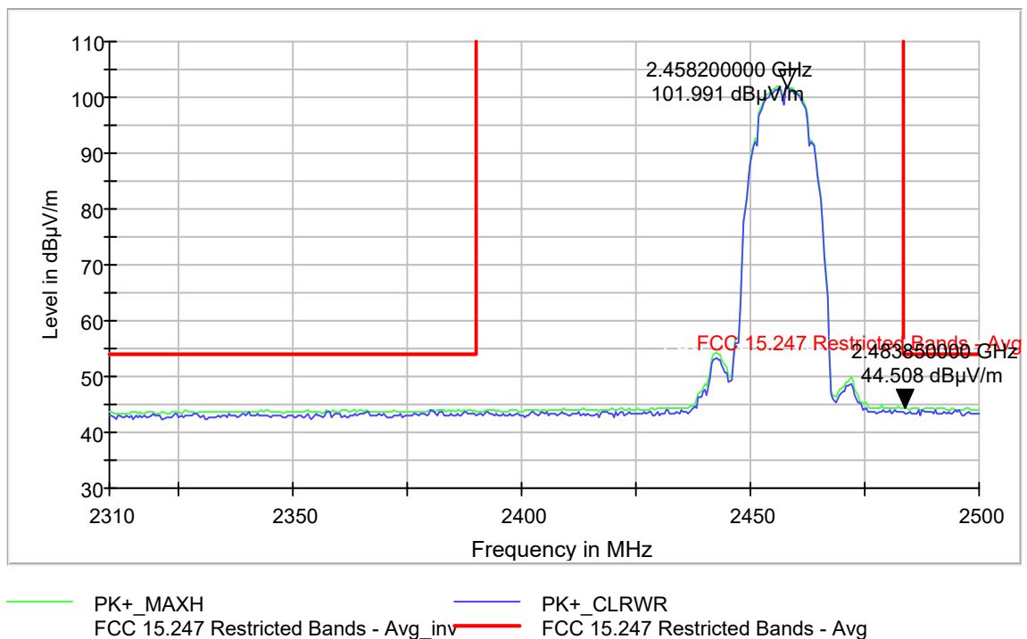
Figure 9-261 Radiated Band Edge Average 802.11b - Ch.10 (2457 MHz)
