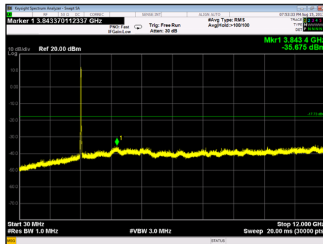
Plot 9-194 Chain B Conducted Spurious Emissions 30 MHz - 12 GHz 802.11n - Ch.6 (2437 MHz)
