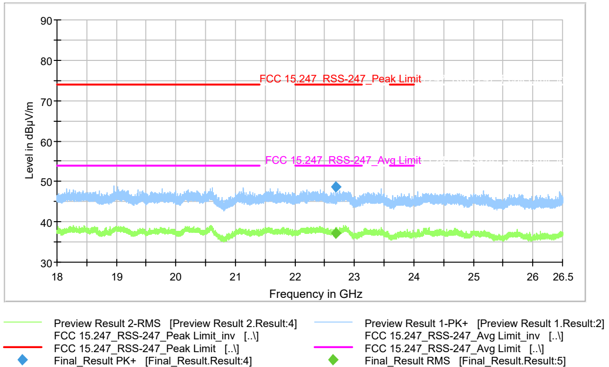
Plot 9-245 Radiated Spurious Emissions 18-26.5GHz 802.11b - Ch.10 (2457 MHz)
