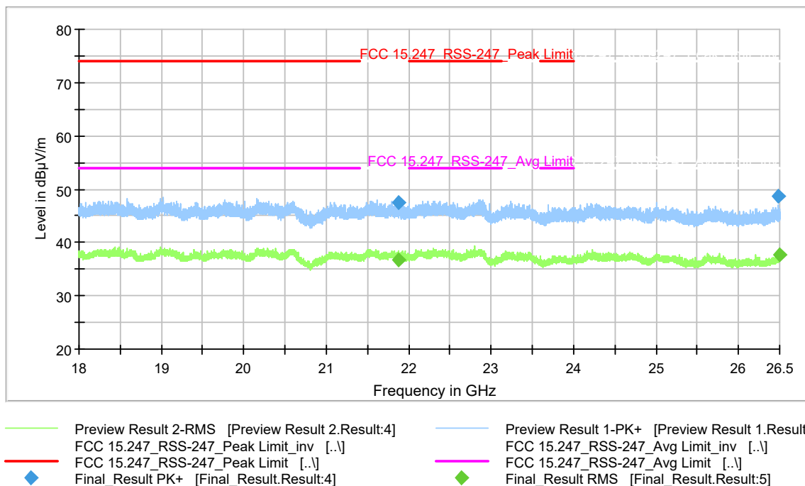
Plot 9-246 Radiated Spurious Emissions 18-26.5GHz 802.11g - Ch.2 (2417 MHz)
