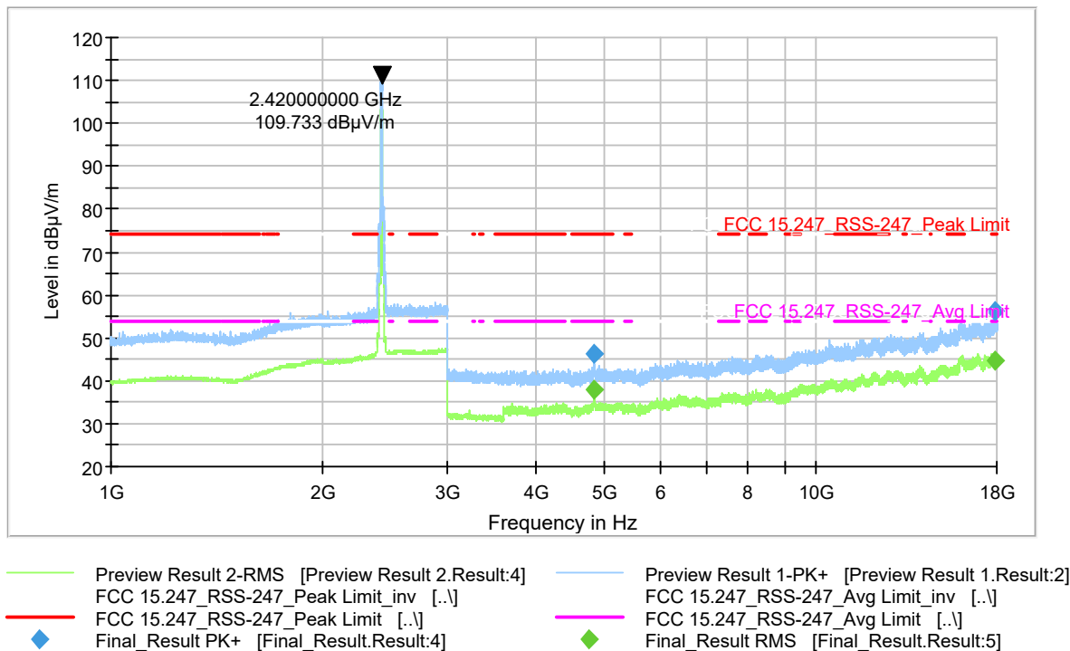
Plot 9-241 Radiated Spurious Emission 1-18GHz 802.11n - Ch.2 (2417 MHz)
