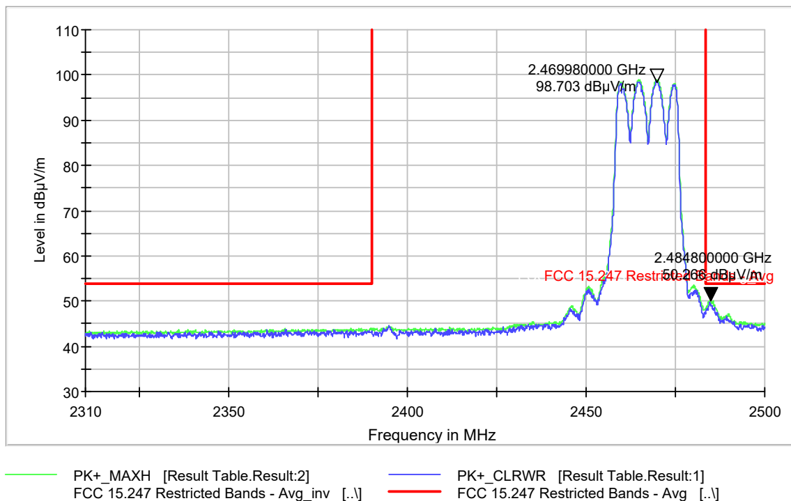
Plot 9-275 Radiated Band Edge Average 802.11g - Ch.12 (2467 MHz)
