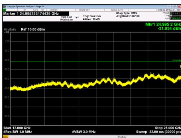
Plot 9-156 Chain A Conducted Spurious Emissions 12 - 25 GHz 802.11n - Ch.12 (2467 MHz)
