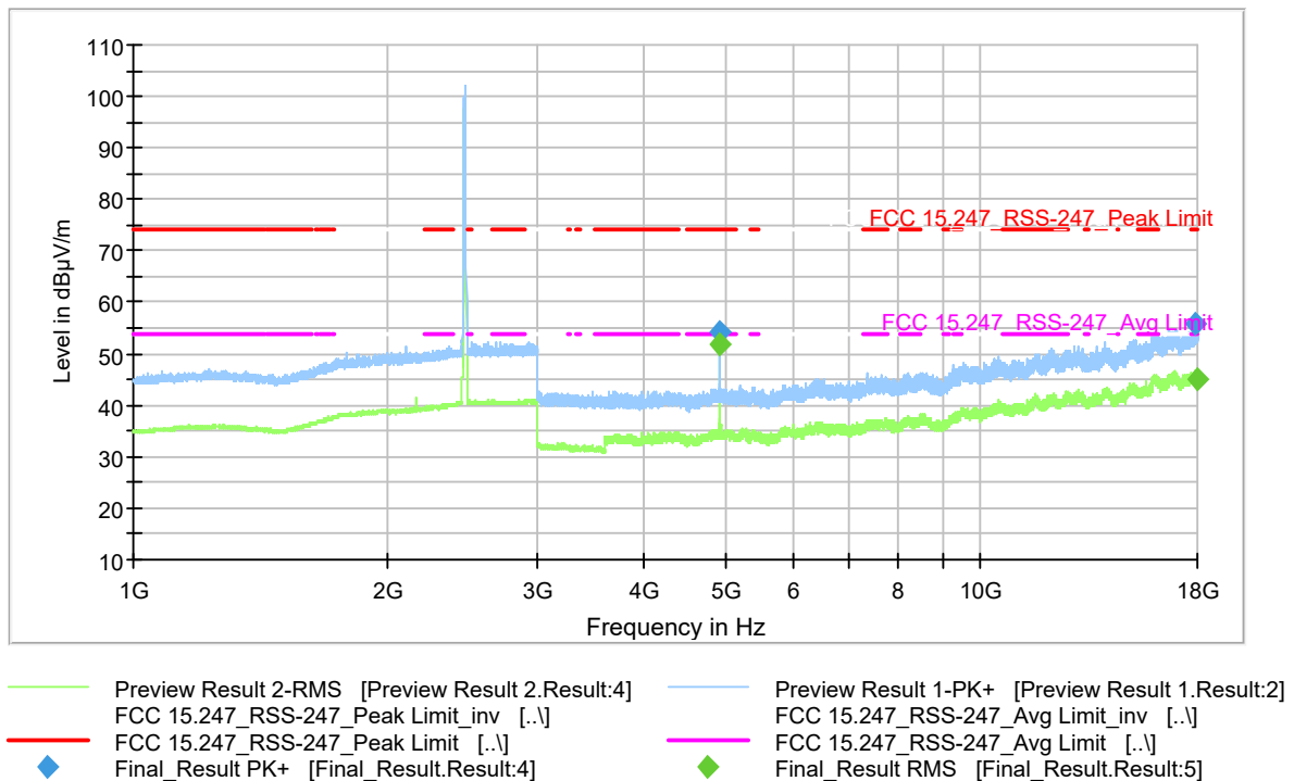
Plot 9-234 Radiated Spurious Emission 1-18GHz 802.11b - Ch.11 (2462 MHz)
