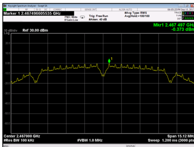
Plot 9-124 Chain A Reference Level 802.11b - Ch.12 (2467 MHz)
