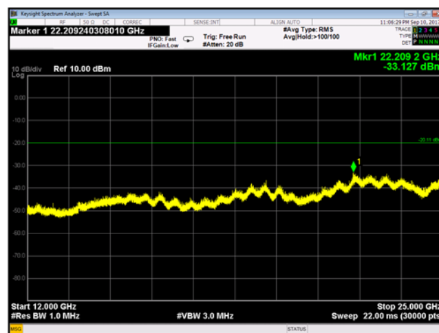
Plot 9-123 Chain A Conducted Spurious Emissions 12 - 25 GHz 802.11b - Ch.11 (2462 MHz)
