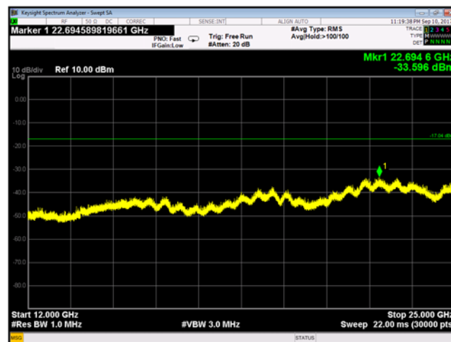
Plot 9-153 Chain A Conducted Spurious Emissions 12 - 25 GHz 802.11n - Ch.11 (2462 MHz)
