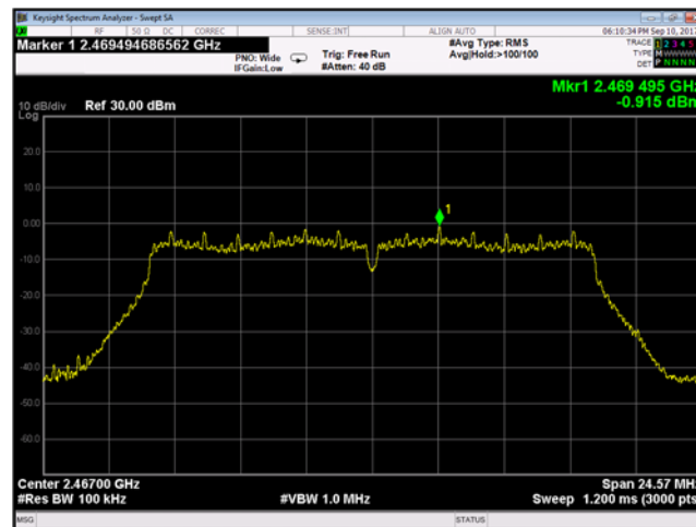
Plot 9-89 Chain A Peak Power Spectral Density 802.11g - Ch.12 (2467 MHz)
