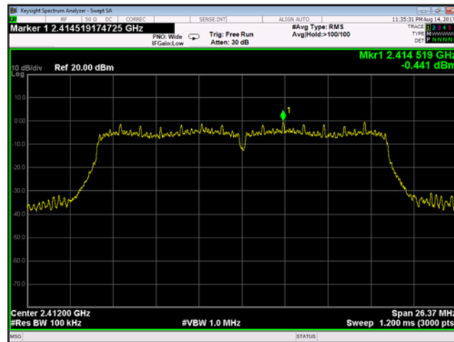
Plot 9-109 Chain B Peak Power Spectral Density 802.11n - Ch.1 (2412 MHz)
