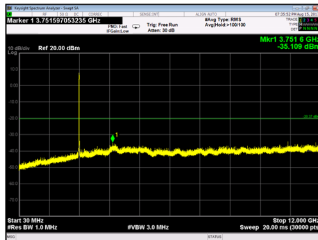
Plot 9-146 Chain A Conducted Spurious Emissions 30 MHz - 12 GHz 802.11n - Ch.1 (2412 MHz)
