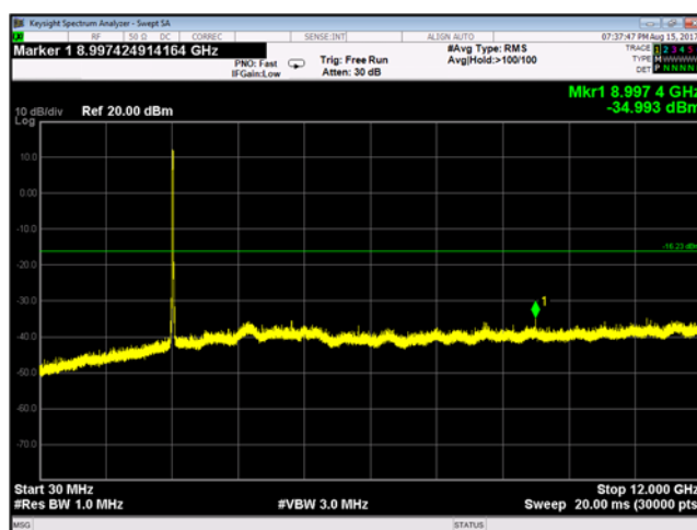
Plot 9-149 Chain A Conducted Spurious Emissions 30 MHz - 12 GHz 802.11n - Ch.6 (2437 MHz)
