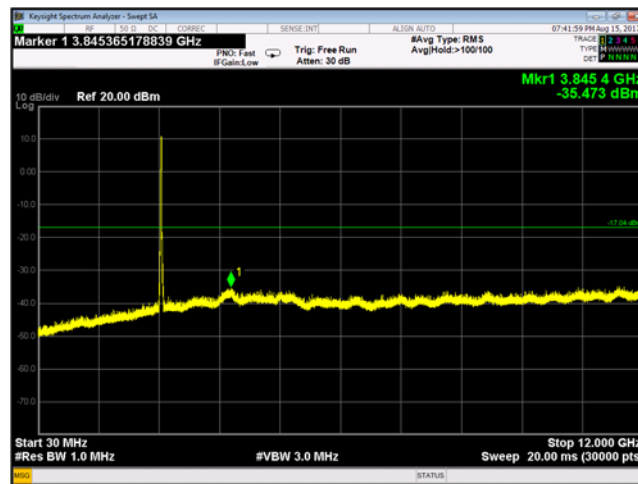
Plot 9-152 Chain A Conducted Spurious Emissions 30 MHz - 12 GHz 802.11n - Ch.11 (2462 MHz)
