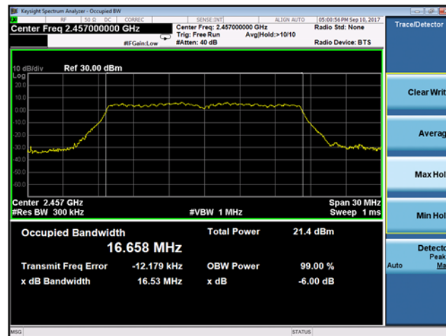
Plot 9-69 Chain B 99% Bandwidth 802.11g - Ch.10 (2457 MHz)
