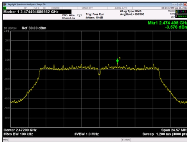
Plot 9-142 Chain A Reference Level 802.11g - Ch.13 (2472 MHz)
