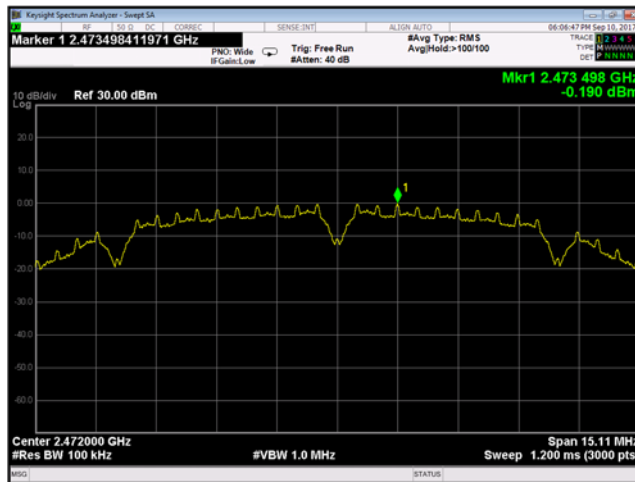
Plot 9-127 Chain A Reference Level 802.11b - Ch.13 (2472 MHz)
