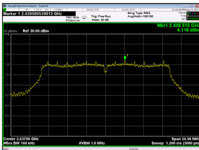
Plot 9-133 Chain A Reference Level 802.11g - Ch.6 (2437 MHz)
