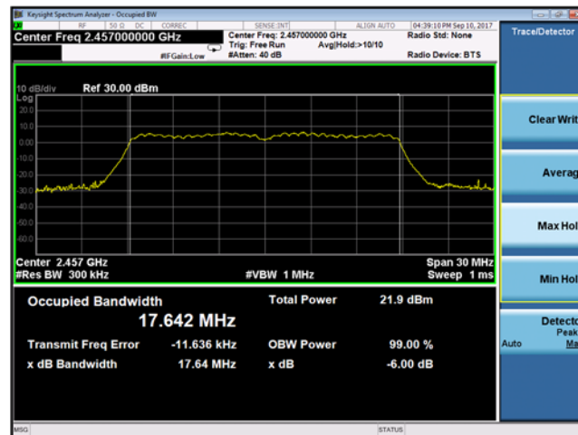
Plot 9-75 Chain B 99% Bandwidth 802.11n - Ch.10 (2457 MHz)
