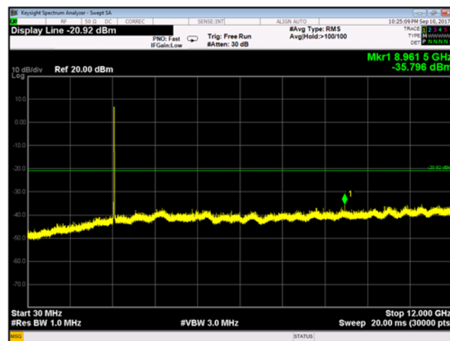
Plot 9-140 Chain A Conducted Spurious Emissions 30 MHz - 12 GHz 802.11g - Ch.12 (2467 MHz)
