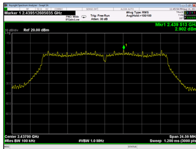
Plot 9-104 Chain B Peak Power Spectral Density 802.11g - Ch.6 (2437 MHz)
