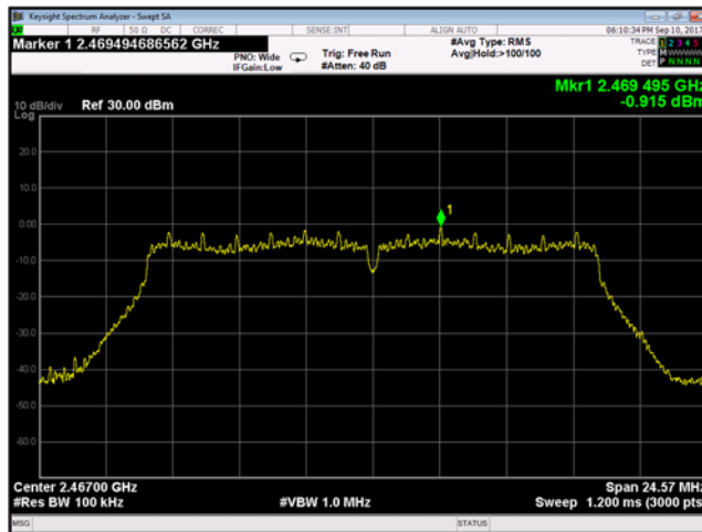
Plot 9-139 Chain A Reference Level 802.11g - Ch.12 (2467 MHz)
