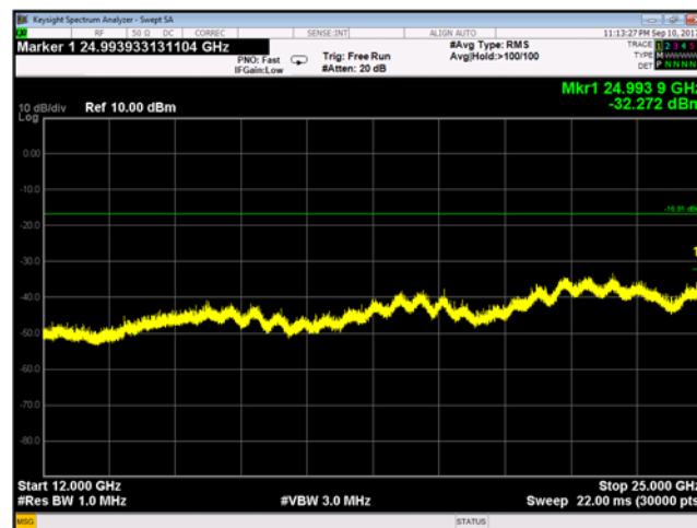
Plot 9-138 Chain A Conducted Spurious Emissions 12 - 25 GHz 802.11g - Ch.11 (2462 MHz)
