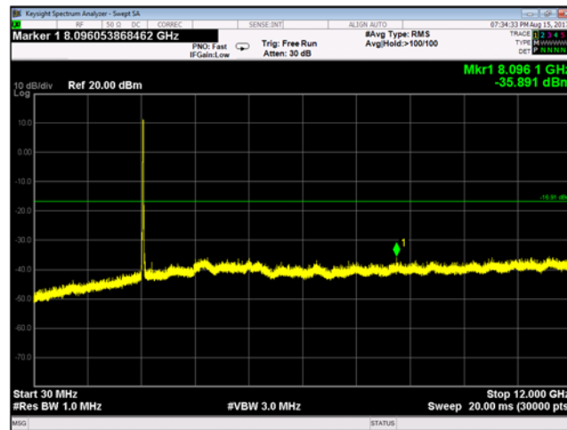
Plot 9-137 Chain A Conducted Spurious Emissions 30 MHz - 12 GHz 802.11g - Ch.11 (2462 MHz)
