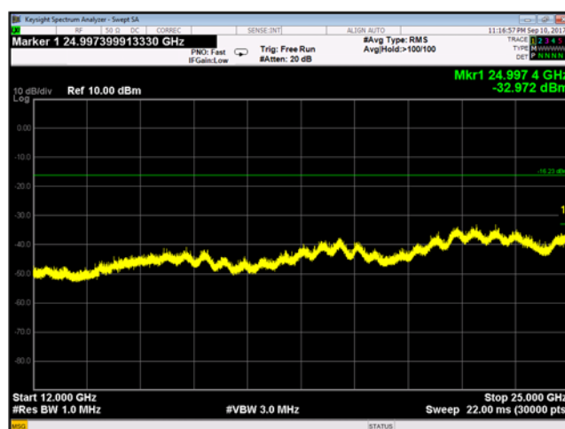
Plot 9-150 Chain A Conducted Spurious Emissions 12 - 25 GHz 802.11n - Ch.6 (2437 MHz)
