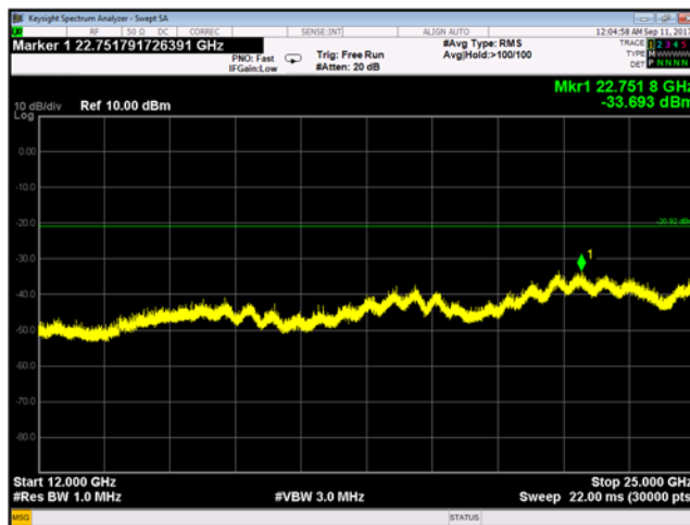
Plot 9-141 Chain A Conducted Spurious Emissions 12 - 25 GHz 802.11g - Ch.12 (2467 MHz)
