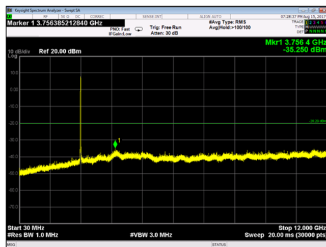
Plot 9-131 Chain A Conducted Spurious Emissions 30 MHz - 12 GHz 802.11g - Ch.1 (2412 MHz)
