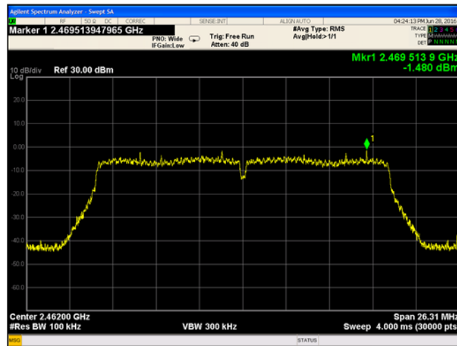
Plot 9-106 Chain A Reference Level 802.11n - Ch.11 (2462 MHz)
