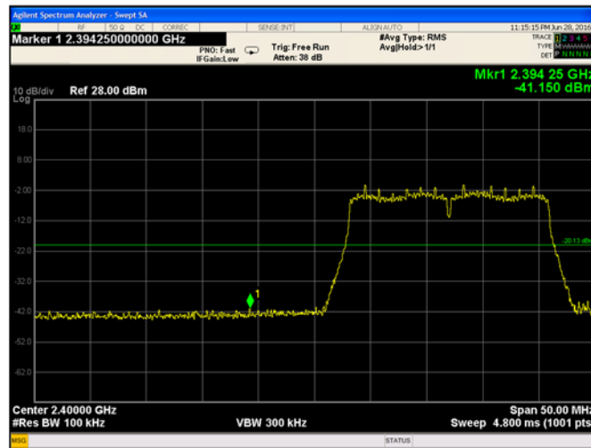
Plot 9-163 Chain B Conducted Band Edge 802.11n - Ch. 1 (2412 MHz)
