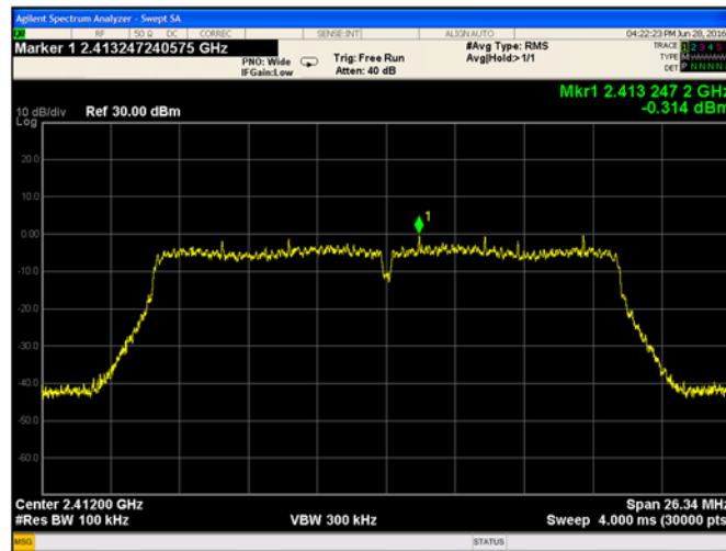
Plot 9-100 Chain A Reference Level 802.11n - Ch.1 (2412 MHz)
