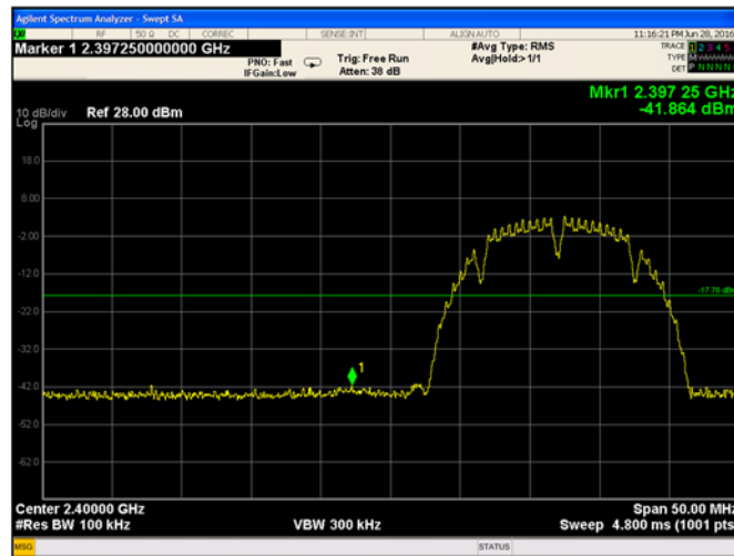
Plot 9-157 Chain B Conducted Band Edge 802.11b - Ch. 1 (2412 MHz)
