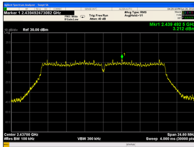
Plot 9-127 Chain B Reference Level 802.11g - Ch.6 (2437 MHz)
