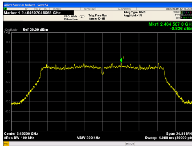
Plot 9-94 Chain A Reference Level 802.11g - Ch.11 (2462 MHz)
