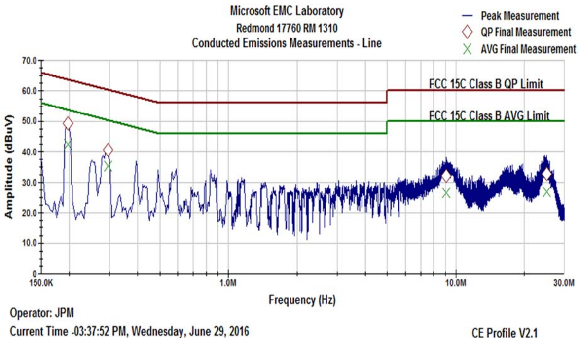
Plot 9-37. AC Line Conducted Emissions- Line (150 kHz- 30 MHz)
