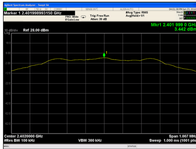
Plot 9-13. Power Spectral Density (Ch. 0)
