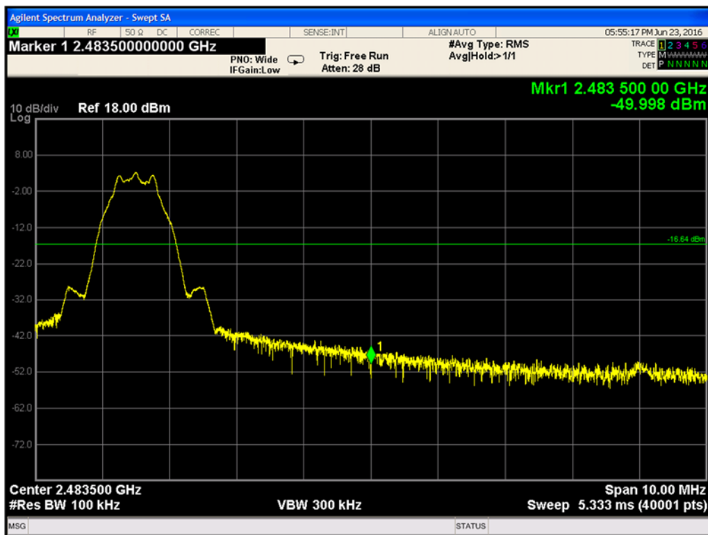
Plot 9-26. Conducted- High Band Edge (Ch. 39)
