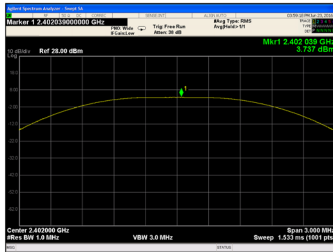
Plot 9-10. Peak Power (Ch. 0)
