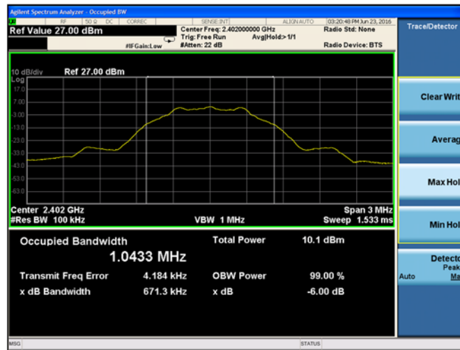
Plot 9-4. 6dB Bandwidth (Ch. 0)
