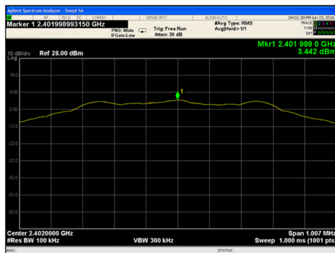
Figure 9-16. Reference Level Measurement (Ch.0)
