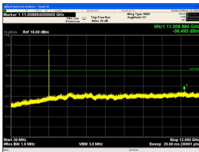
Plot 9-20. Conducted Spurious Emissions 30-12000 MHz (Ch. 19)
