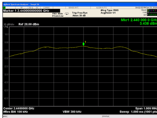
Plot 9-14. Power Spectral Density (Ch. 19)
