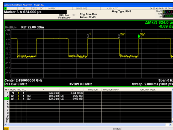
Figure 9-3. Duty Cycle 2480MHz (Ch.39)
