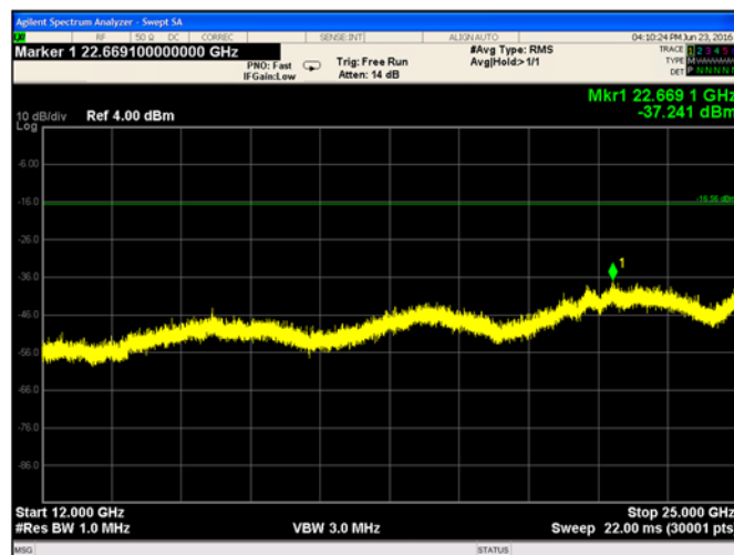
Figure 9-18. Conducted Spurious Emissions 12-25 GHz (Ch.0)
