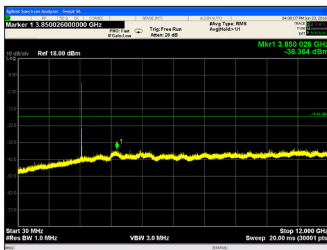
Figure 9-23. Conducted Spurious Emissions 30-12000 MHz (Ch.39)
