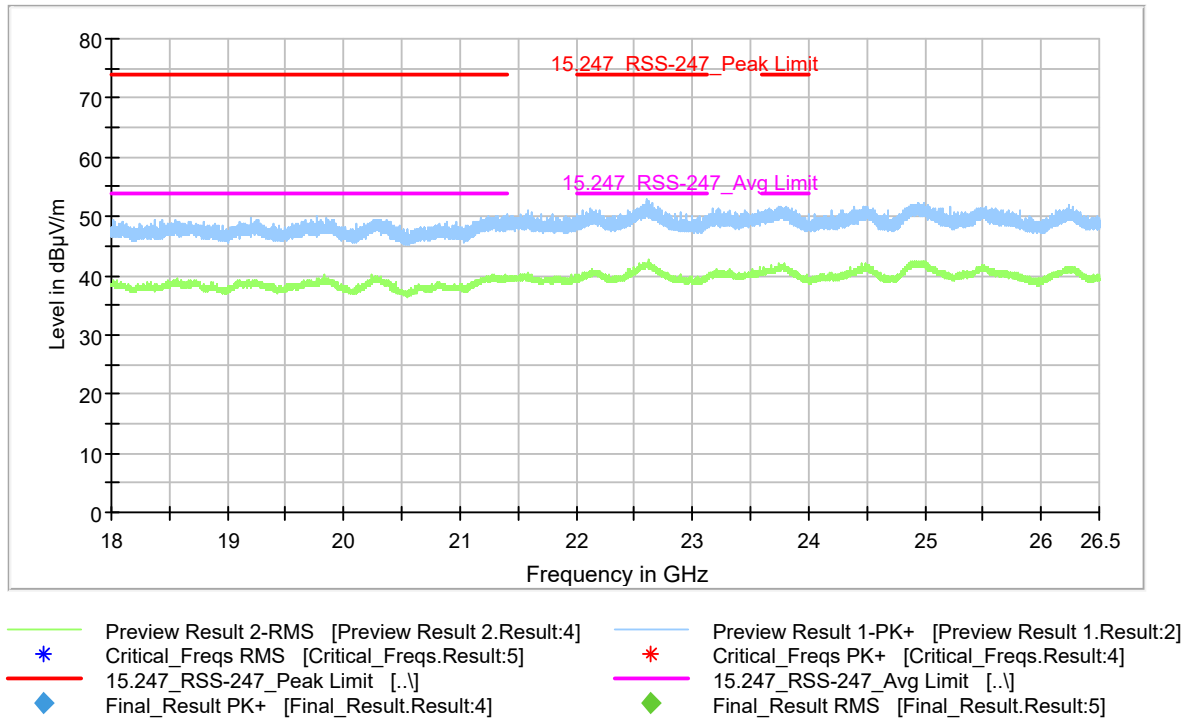
Plot 9-35. Radiated Spurious Emissions (Ch. 0) (18 – 26.5 GHz)
