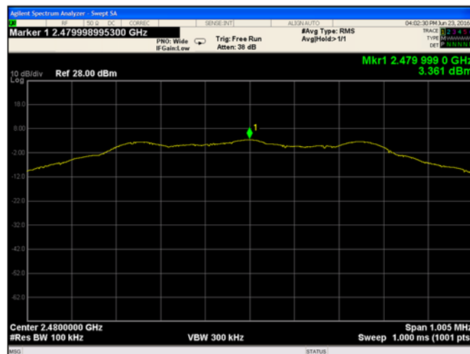
Plot 9-15. Power Spectral Density (Ch. 39)
