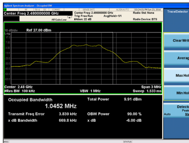
Plot 9-6. 6dB Bandwidth (Ch. 39)
