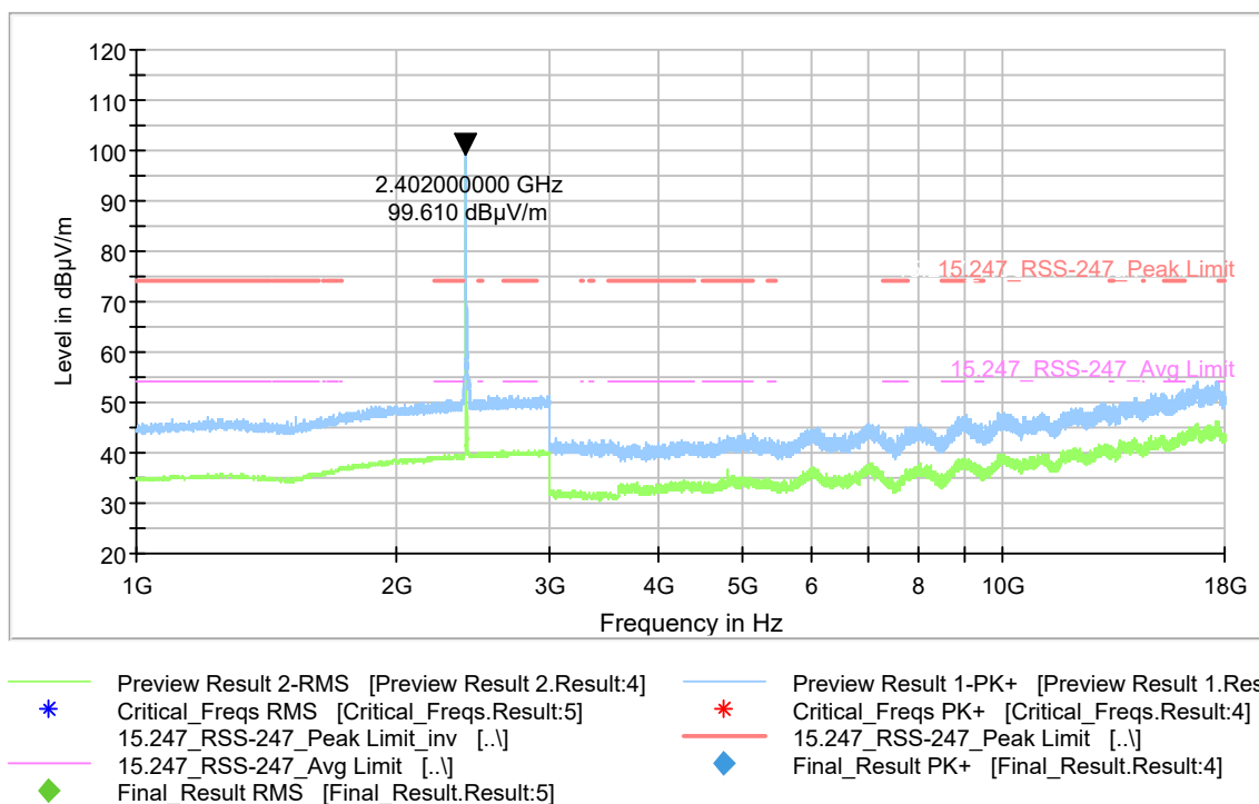
Plot 9-32. Radiated Spurious Emissions 1-18 GHz (Ch. 0)
