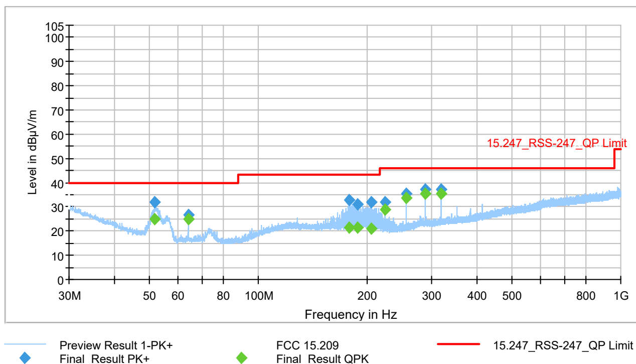
Plot 9-31. Radiated Spurious Emissions (Ch. 0) 2402 (30MHz - 1GHz)
