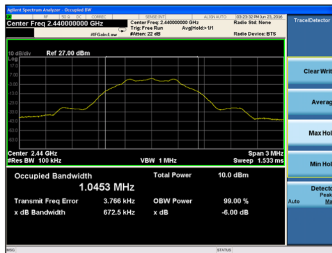
Plot 9-5. 6dB Bandwidth (Ch. 19)
