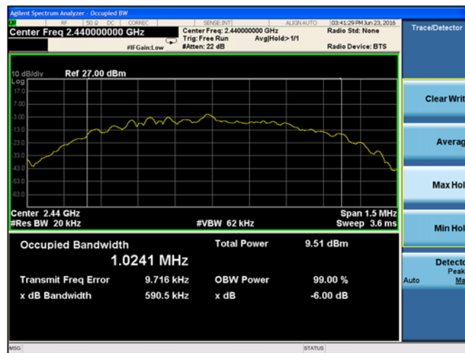
Plot 9-8. 99% Bandwidth (Ch. 19)
