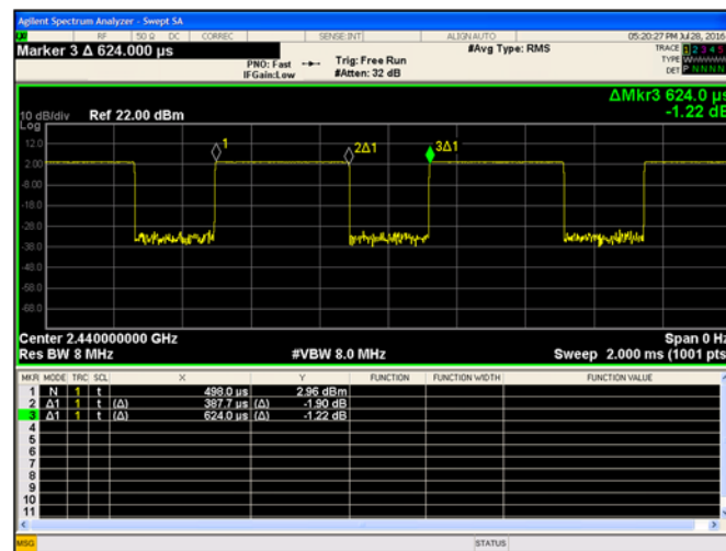
Figure 9-2. Duty Cycle 2440MHz (Ch.19)
