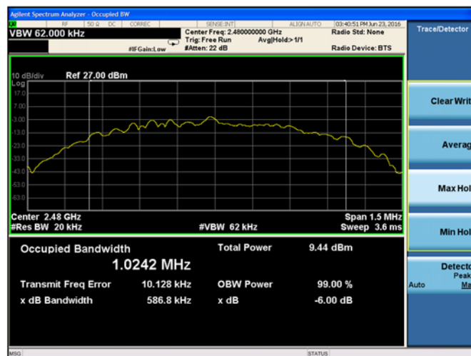
Plot 9-9. 99% Bandwidth (Ch. 39)
