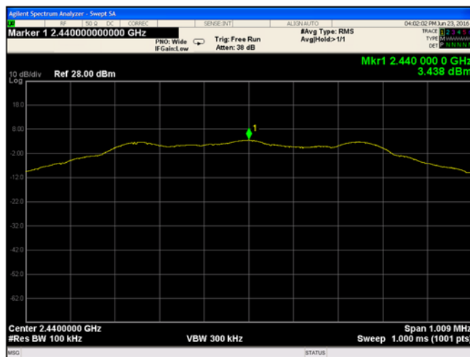
Figure 9-19. Reference Level Measurement (Ch.19)
