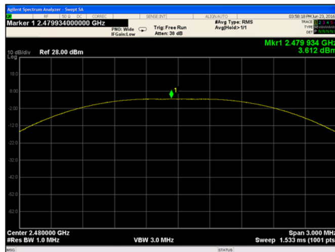
Plot 9-12. Peak Power (Ch. 39)
