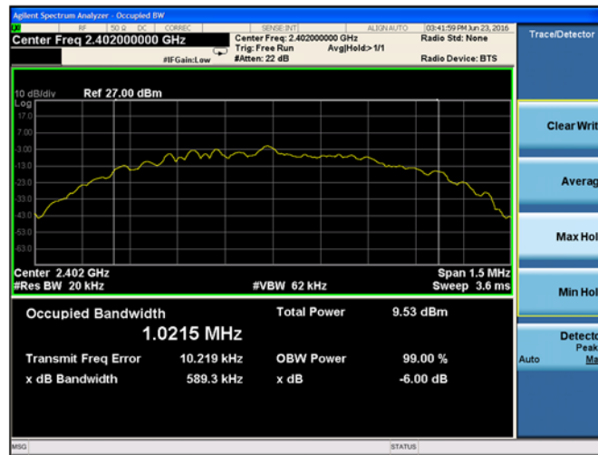
Plot 9-7. 99% Bandwidth (Ch. 0)
