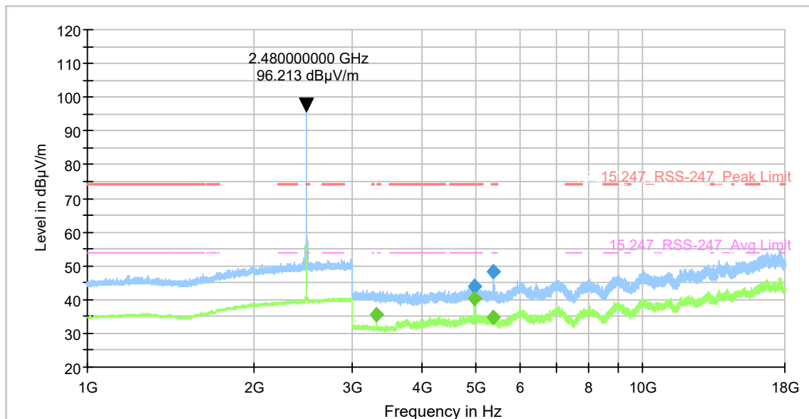
Plot 9-33. Radiated Spurious Emissions 1-18 GHz (Ch. 19)
