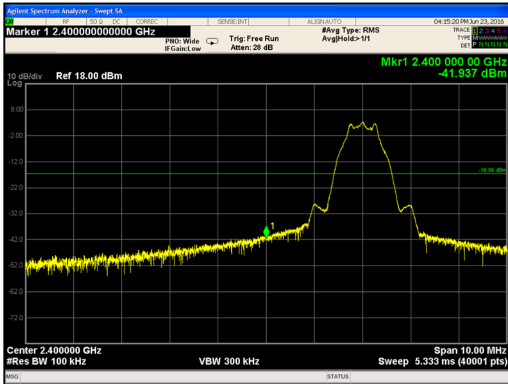
Plot 9-25. Conducted-Low Band Edge (Ch. 0)
