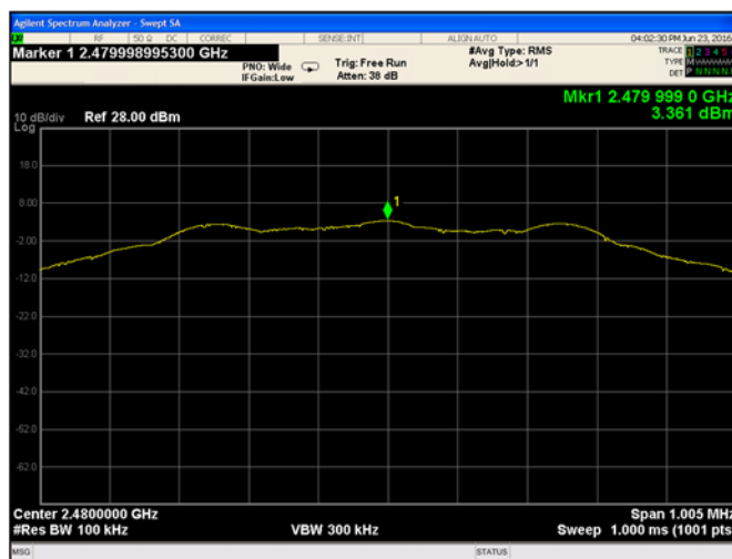
Figure 9-22. Reference Level Measurement (Ch.39)
