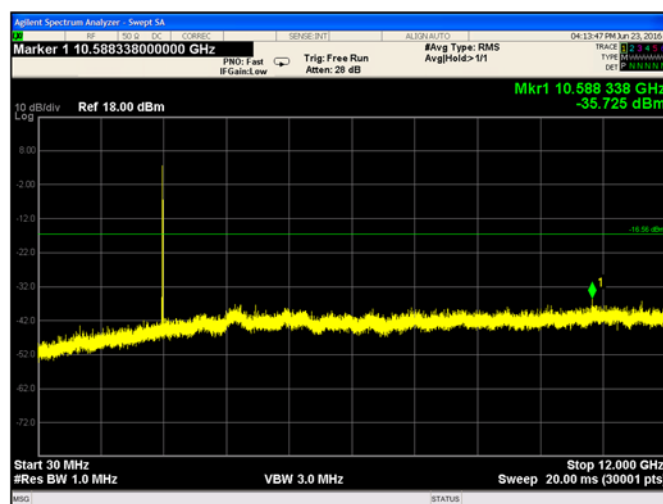
Plot 9-17. Conducted Spurious Emissions 30-12000 MHz (Ch. 0)
