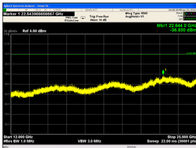
Plot 9-21. Conducted Spurious Emissions 12-25 GHz (Ch. 19)
