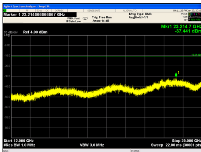
Figure 9-24. Conducted Spurious Emissions 12-25GHz (Ch.39)
