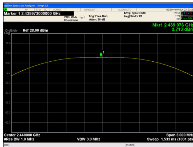
Plot 9-11. Peak Power (Ch. 19)
