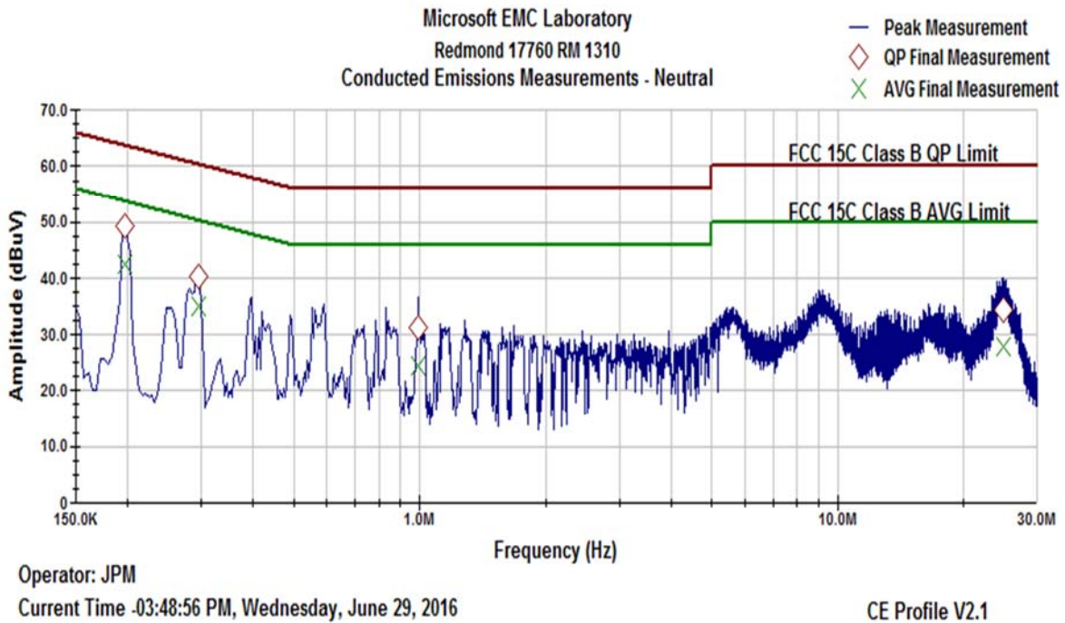
Plot 9-36. AC Line Conducted Emissions- Neutral (150 kHz- 30 MHz)
