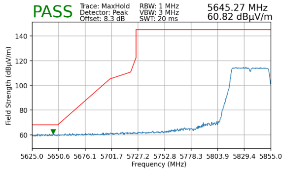
Plot 7-36. Lower Band Edge Plot MIMO (Peak – UNII Band 4)
