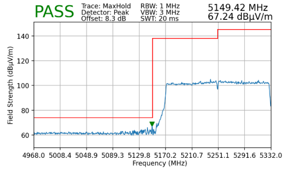
Plot 7-41. Lower Band Edge Plot MIMO (Peak – UNII Band 1)
