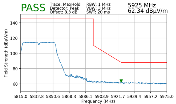
Plot 7-38. Upper Band Edge Plot MIMO (Peak – UNII Band 4)
