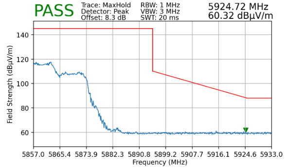
Plot 7-31. Upper Band Edge Plot MIMO (Peak – UNII Band 4)
