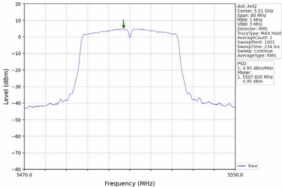
802.11n(HT40)_LCH_5510MHz_MIMO_NTNV
