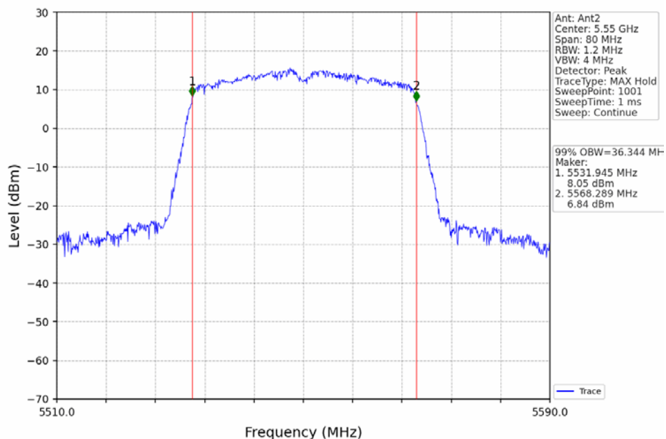
802.11n(HT40)_MCH_5550MHz_Ant2_NTNV
