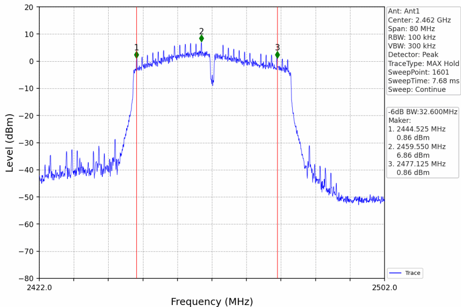
11N40_HCH_2462MHz_Ant1_NTNV
