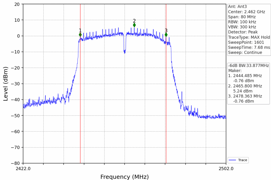
11N40_HCH_2462MHz_Ant3_NTNV
