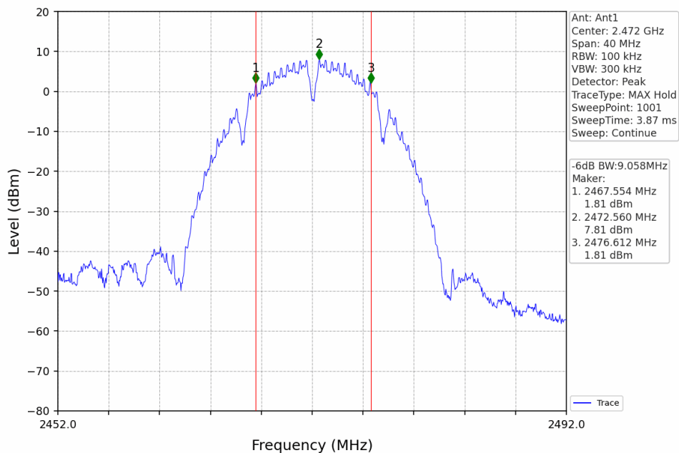
11B_HCH_2472MHz_Ant1_NTNV
