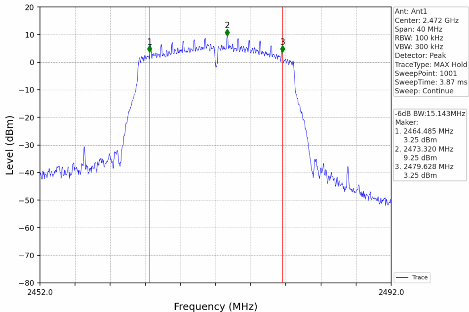
11N20_HCH_2472MHz_Ant1_NTNV
