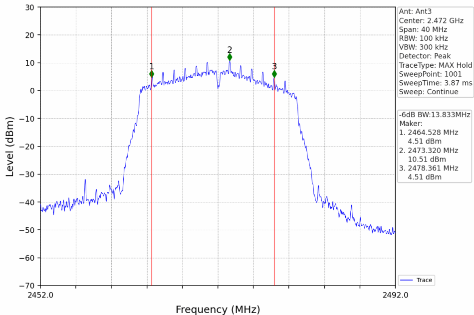
11N20_HCH_2472MHz_Ant3_NTNV
