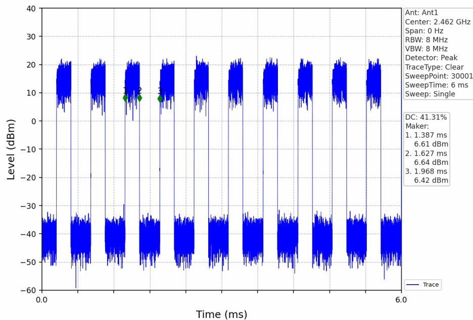
11N40_HCH_2462MHz_Ant1_NTNV
