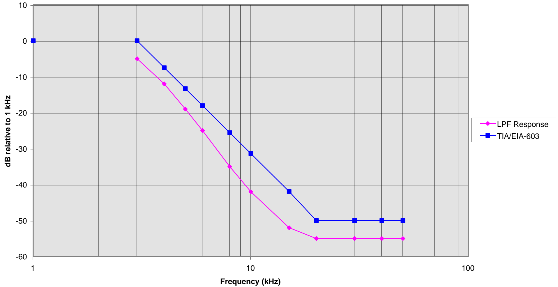
Audio Low Pass Filter Response
