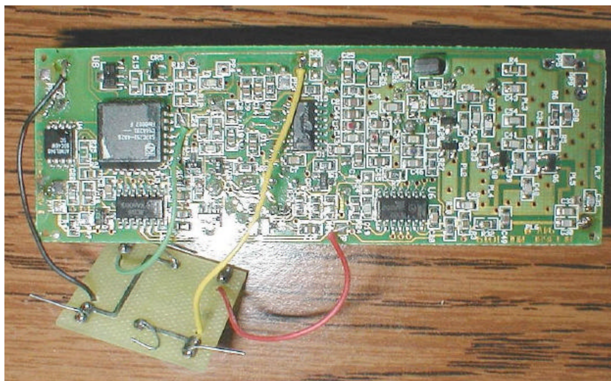
PCB1 Bottom View
