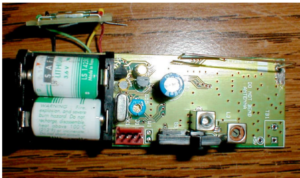
PCB1 Bottom View
