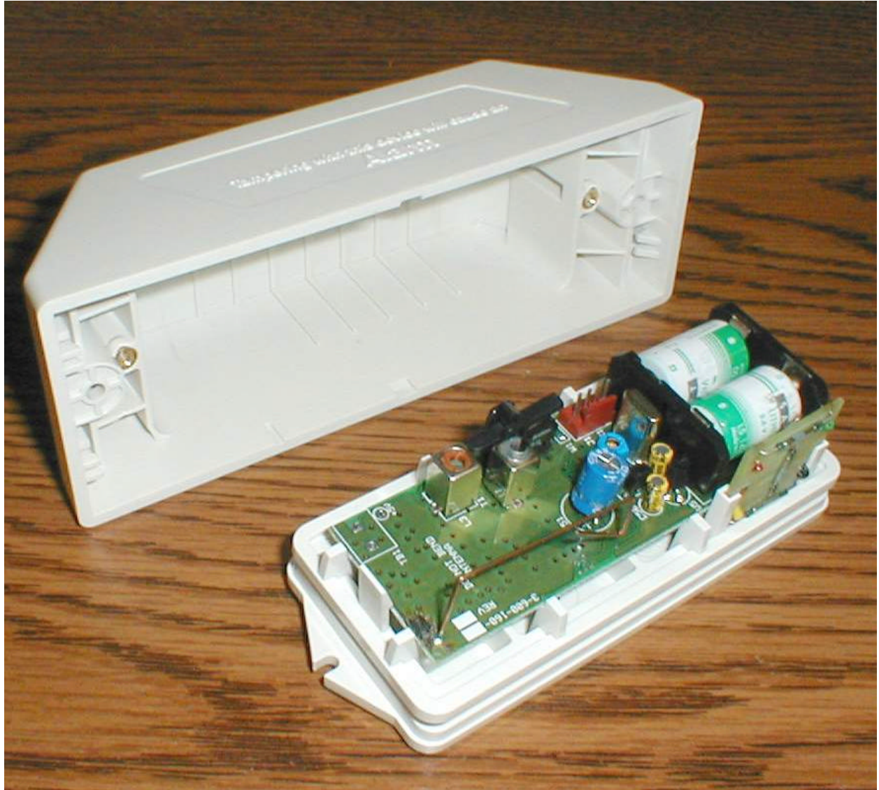
Top Cover Removed
