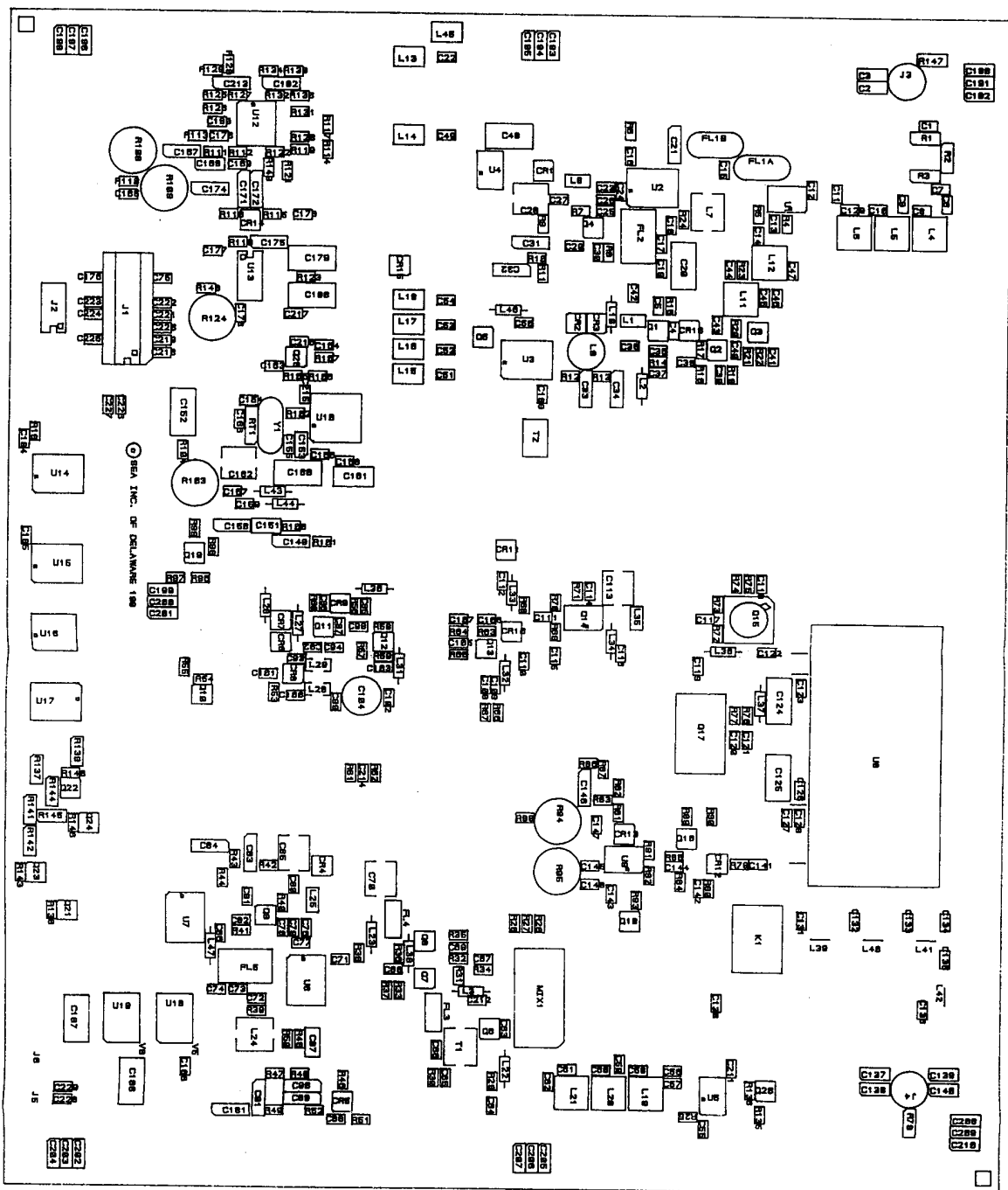
ASY-7157-01 RF Circuit Board Component Detail Figure 7.2
