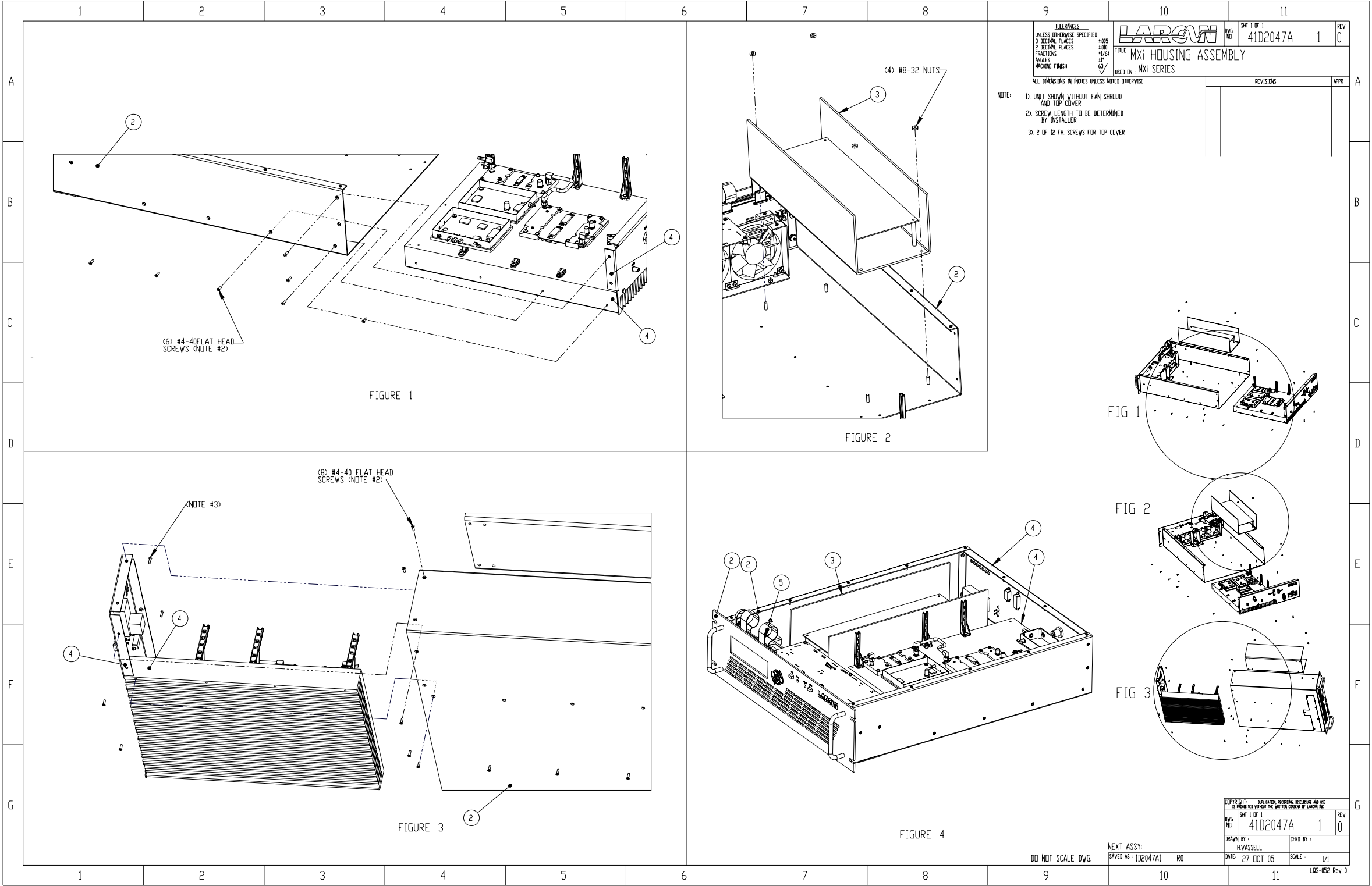
Figure 3 41D2047A MXi Housing Assembly sht1 Rev 0
