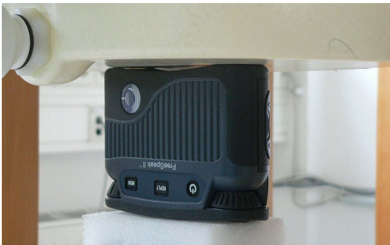
Fig. 12: Body worn configuration for Clear-Com BP1G9, position 4, bottom edge towards the phantom, 0 mm distance.
