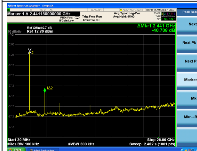
BLE-Out of Band Emission-Mid-2Mbps
