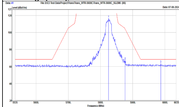
TX, 802.11n(HT20) (Ch 165) Band Edge (Peak), Horizontal
