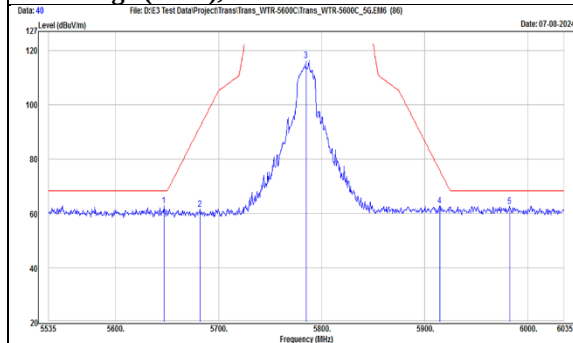
TX, 802.11n(HT20) (Ch 157) Band Edge (Peak), Horizontal
