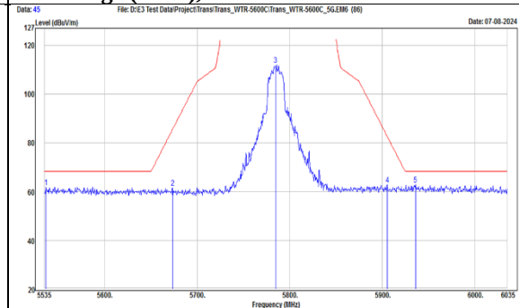
TX, 802.11n(HT20) (Ch 157) Band Edge (Peak), Vertical
