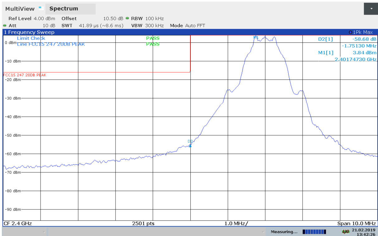
Conducted Emissions, 2402 MHz, Lower Band Edge
