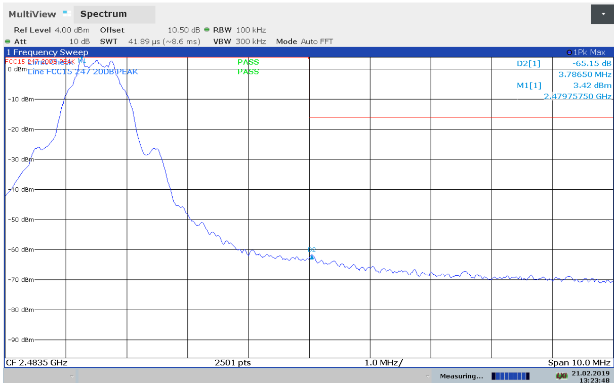
Conducted Emissions, 2480 MHz, Upper Band Edge
