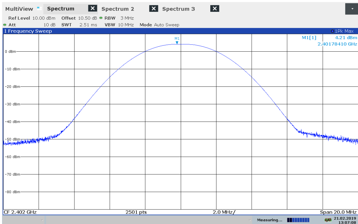
Conducted Power, 2402 MHz
