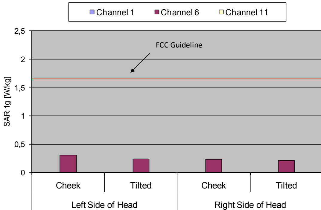
Fig. 8: The measured head SAR values for IEEE 802.11 b for the Ascom WH1-AAAA/PF in head configuration, in comparison to the FCC exposure limit.
