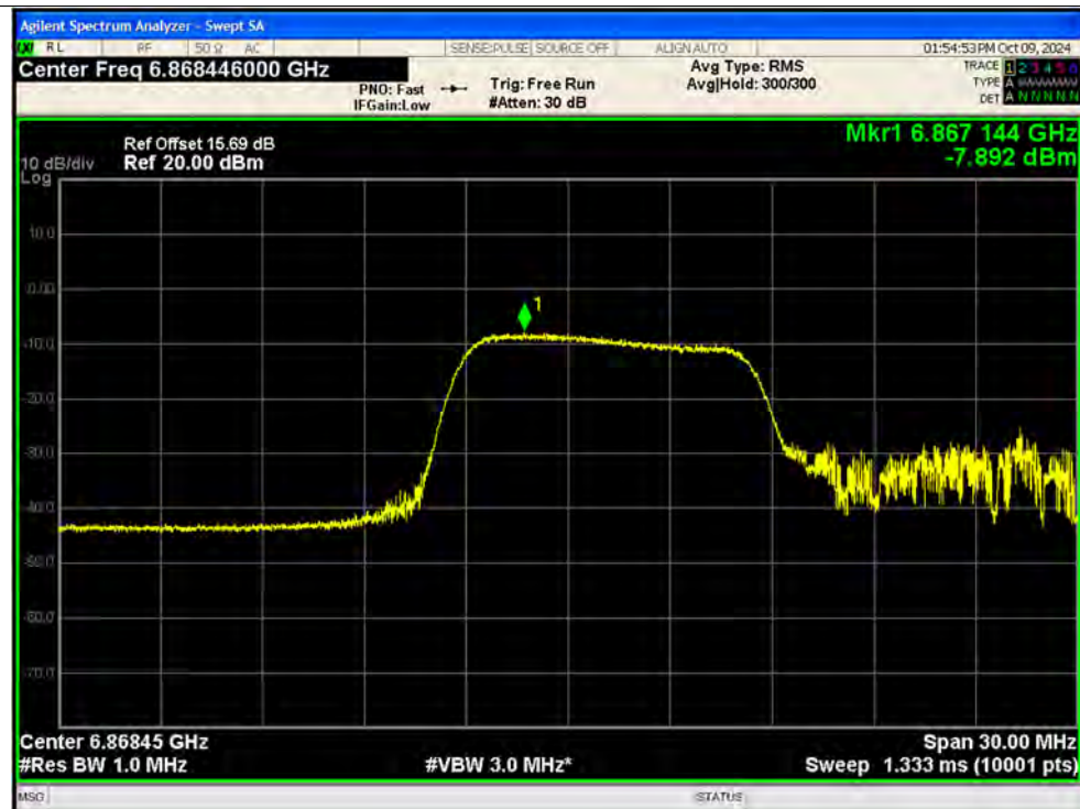
PSD NVNT ax20 106@53 6875MHz Ant2 MIMO
