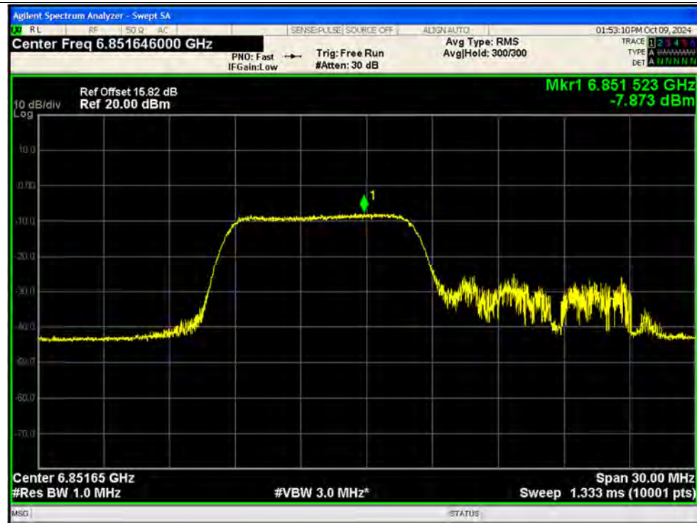
PSD NVNT ax20 106@53 6855MHz Ant2 MIMO
