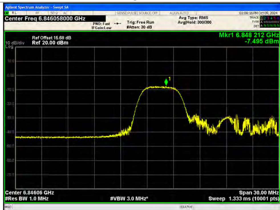
PSD NVNT ax20 52@37 6855MHz Ant2 MIMO
