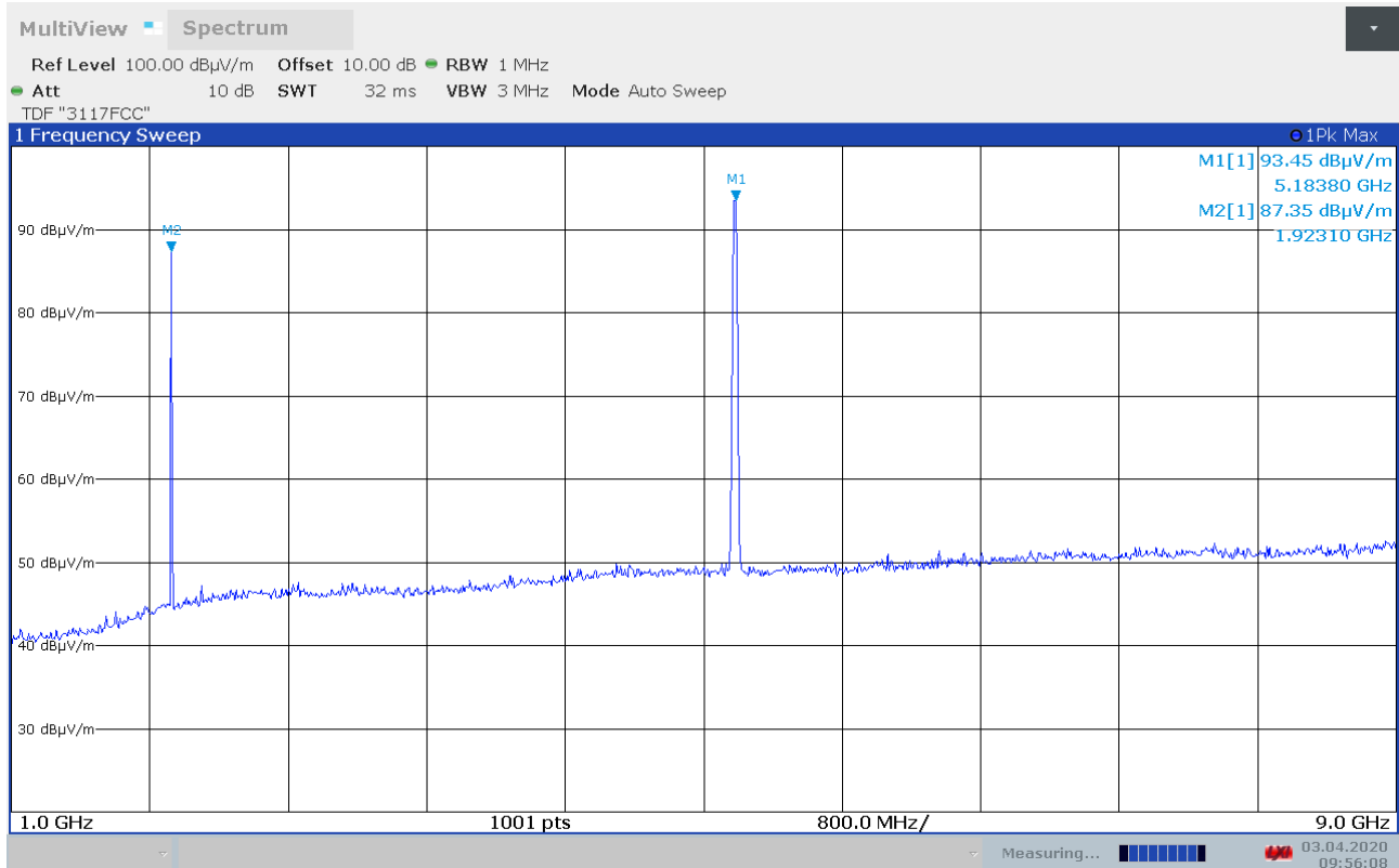
Maximum Emissions 1 – 9 GHz, DECT Ch02 + WiFi Ch36 6Mb, VP
