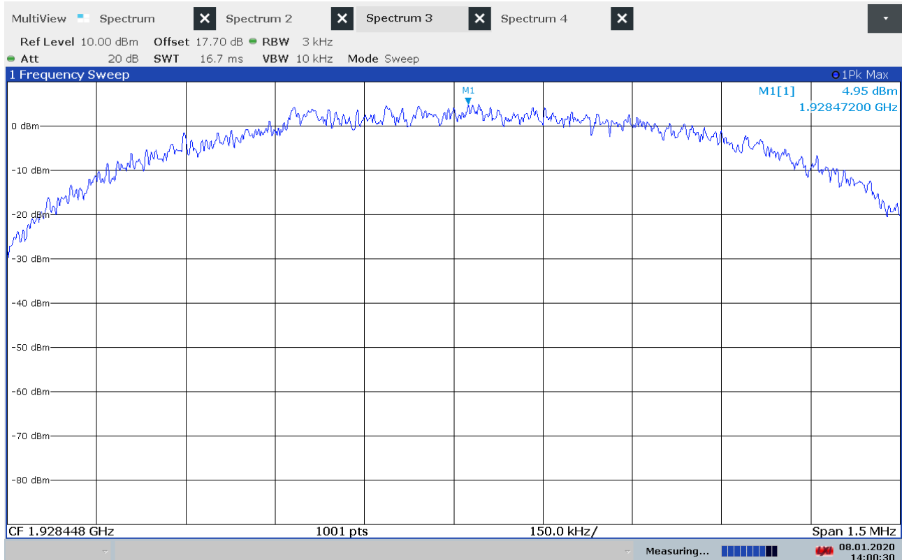
PSD, Overview, Upper Channel
