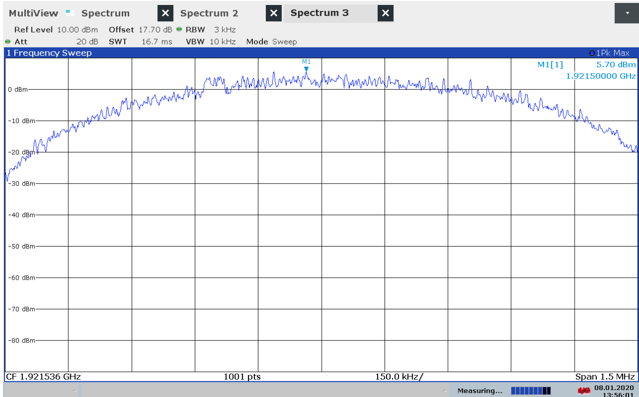
PSD, Overview, Lower Channel
