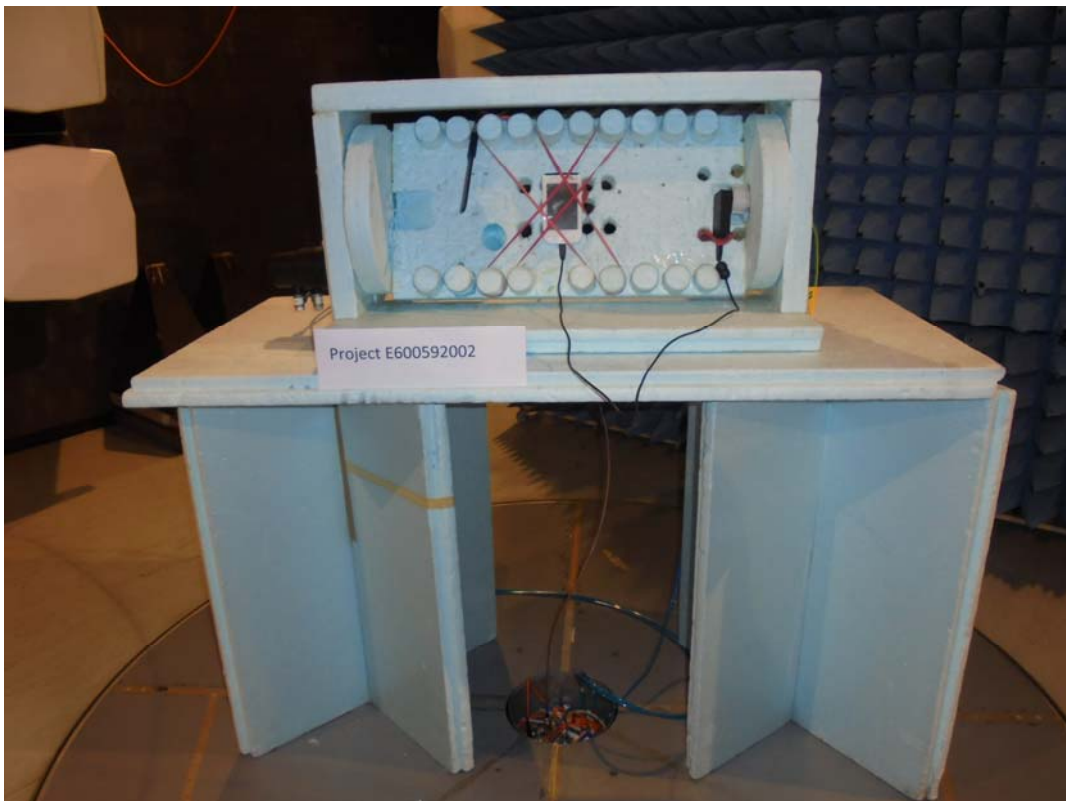
Test setup 30MHz up to 1GHz, close-up view
