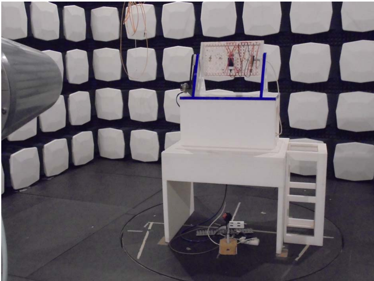
Test set-up, long shot view
