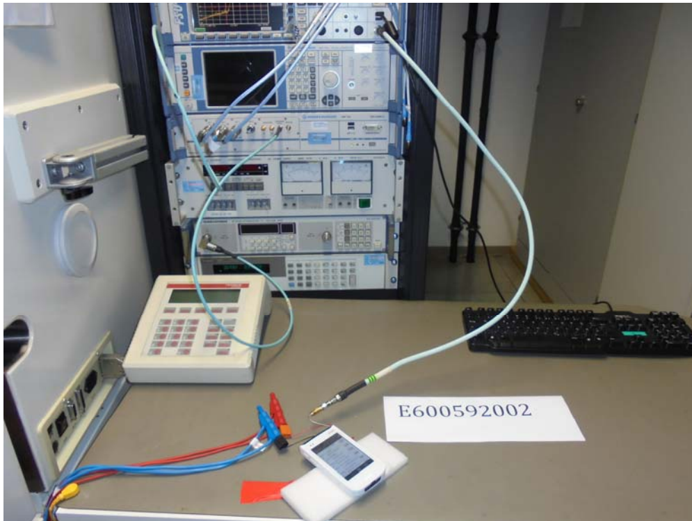
Test setup conducted RF Parameters
