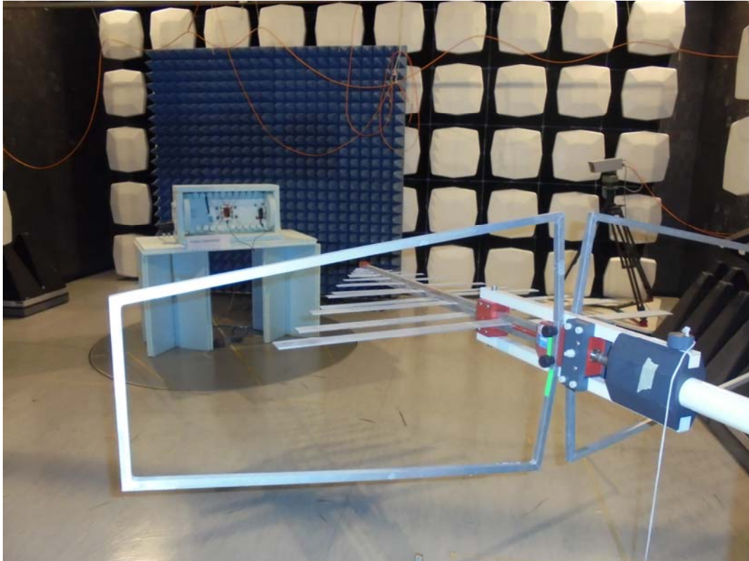
Test setup 30MHz up to 1GHz, long shot view
