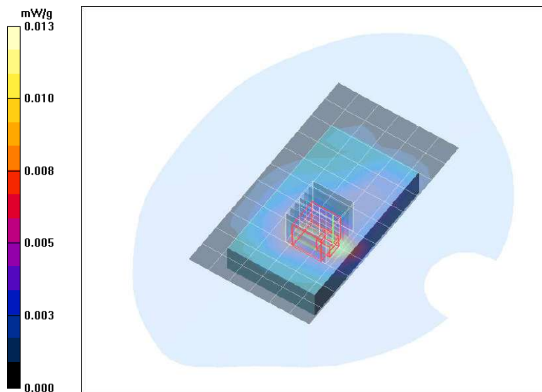
Plot. 6: SAR distribution plot for DECT (Ant.0), channel 2, Body-Worn Configuration, back side, 0mm distance to phantom.
