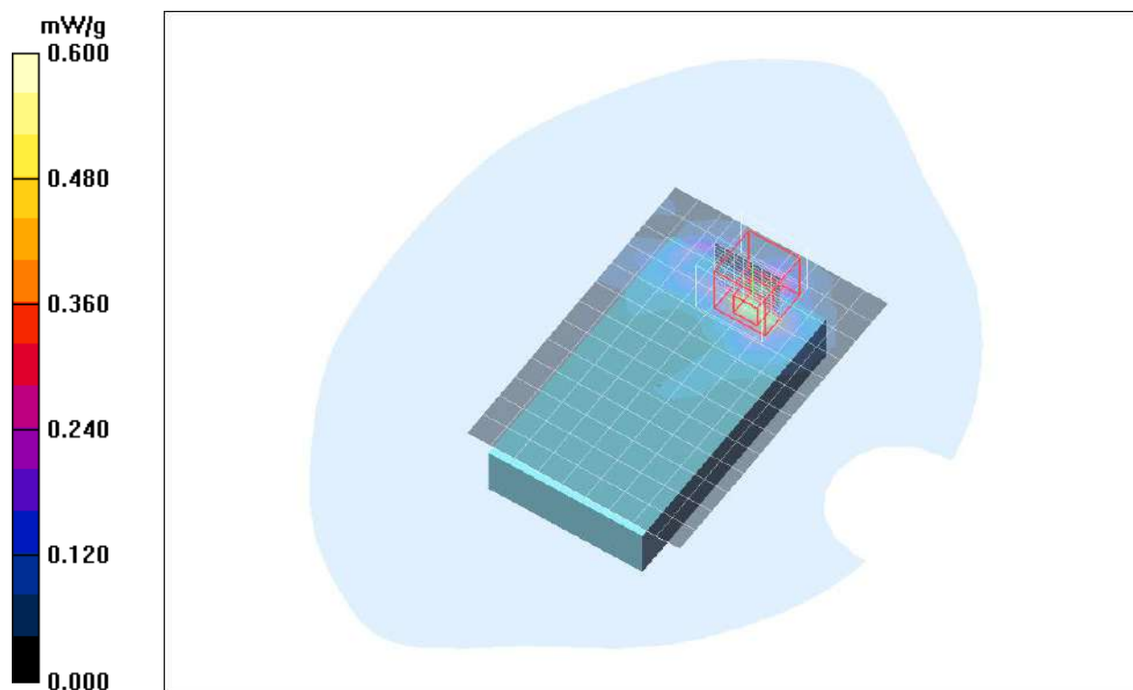
Plot. 9: SAR distribution plot for IEEE802.11a, channel 36, Data Rate 6 MB/s, Body-Worn Configuration, front side, 0mm distance to phantom.
