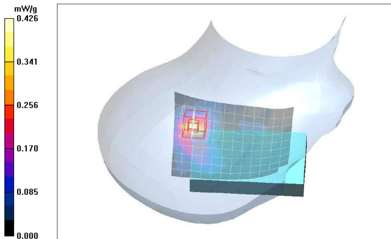
Plot. 4: SAR distribution plot for IEEE802.11a, channel 48, Head Configuration, Right Cheek.
