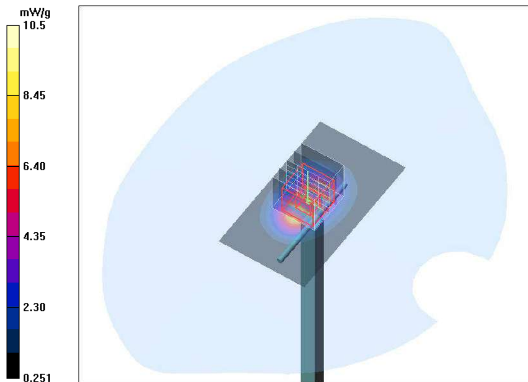
Plot. 11: System Verification Measurement 1900 MHz, Head.
