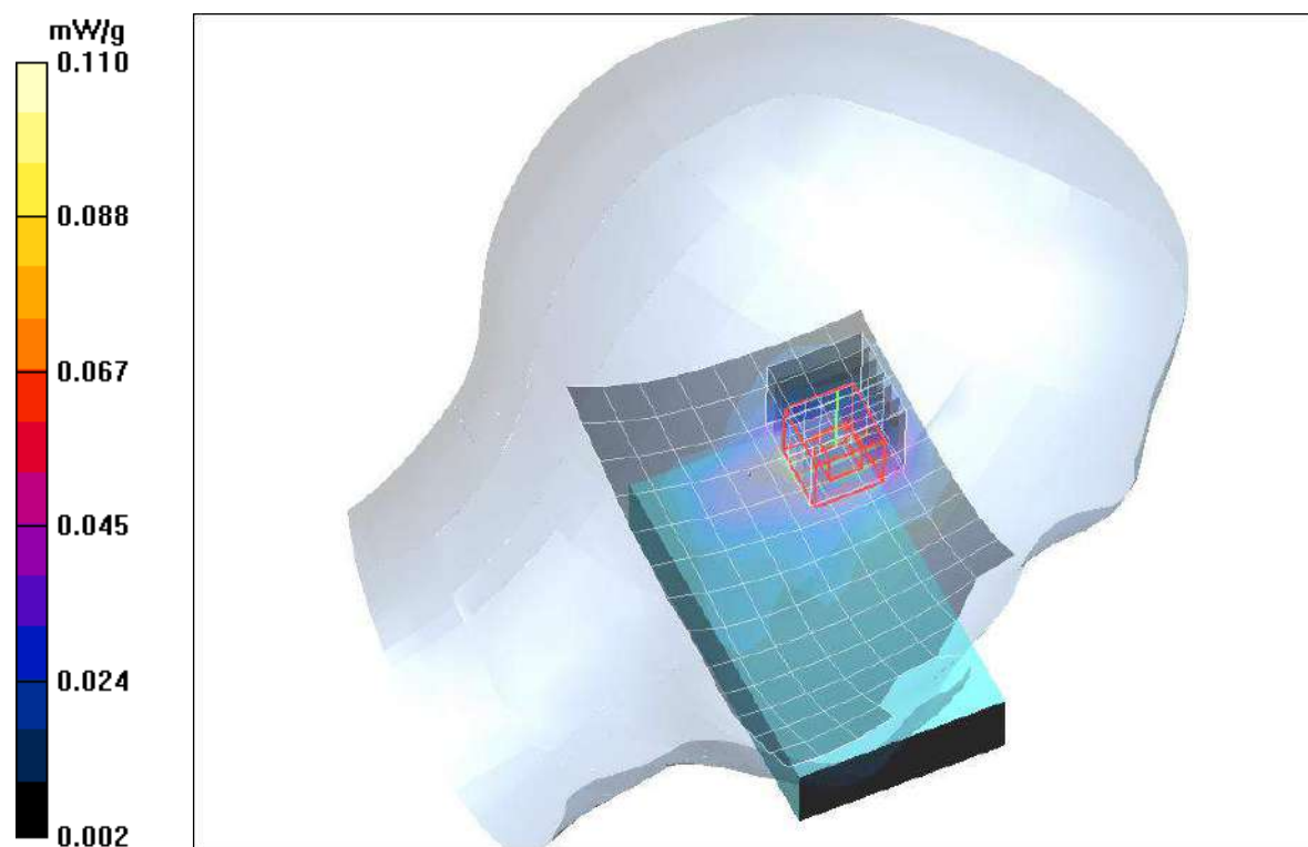
Plot. 3: SAR distribution plot for IEEE802.11 b, channel 1, Head Configuration, Left Cheek.
