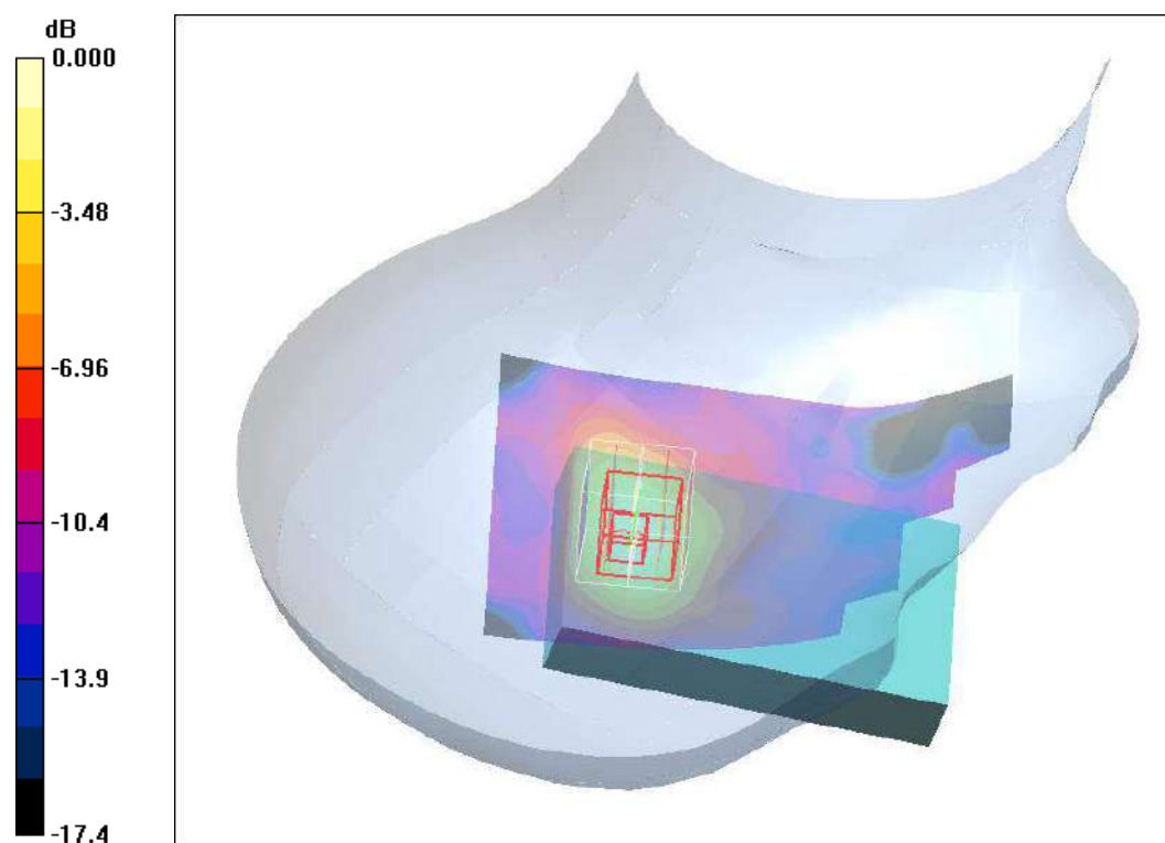
Plot. 1: SAR distribution plot for DECT (Ant.0), channel 2, Head Configuration, Right Tilt.
