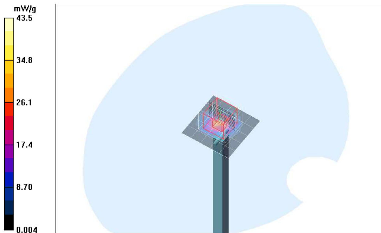
Plot. 14: System Verification Measurement 5600 MHz, Head..
