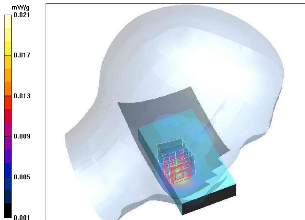
Plot. 2: SAR distribution plot for DECT (Ant.1), channel 0, Head Configuration, Left Cheek.
