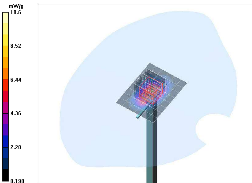
Plot. 16: System Verification Measurement 1900 MHz, Body.
