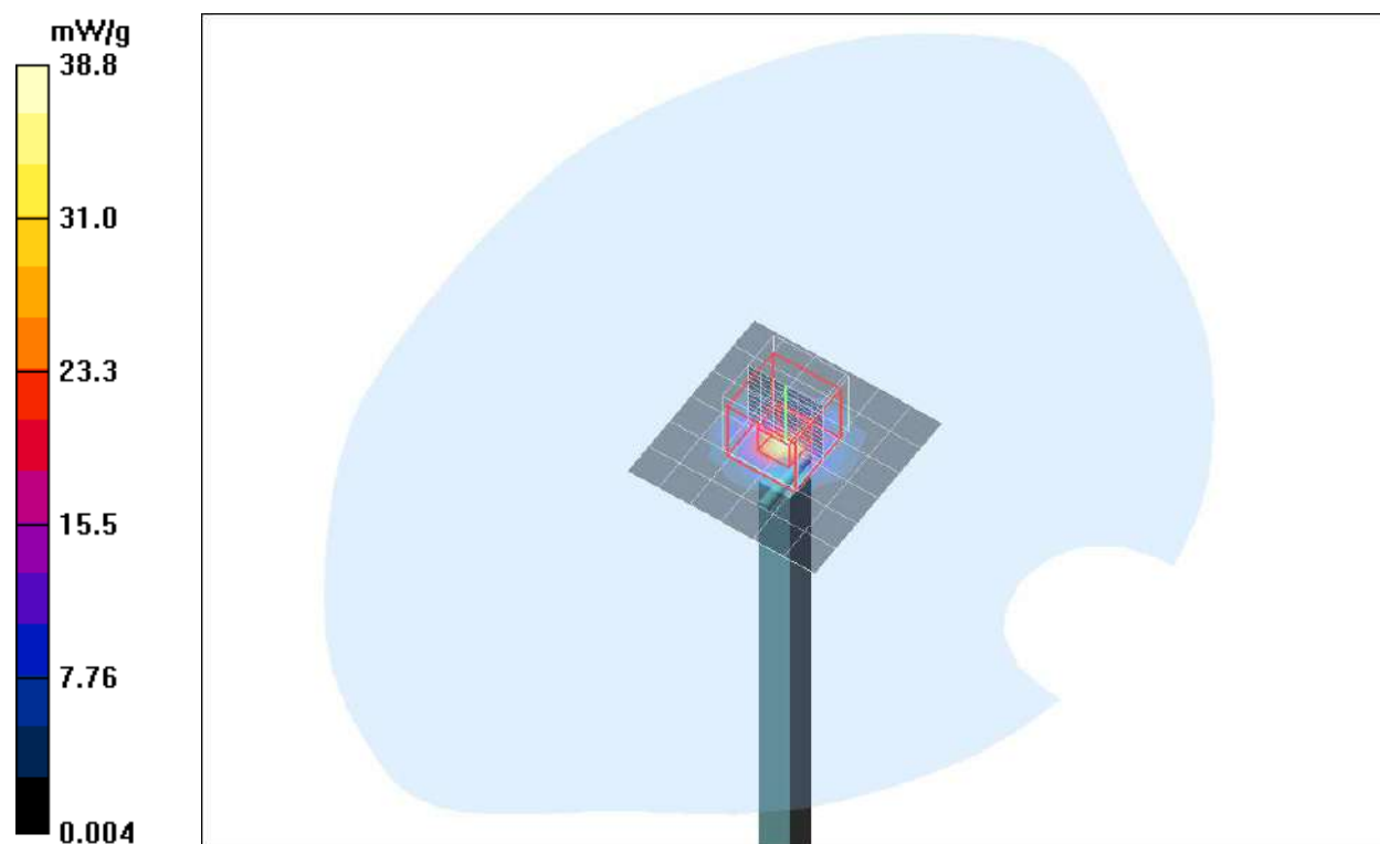
Plot. 20: System Verification Measurement 5750 MHz, Body.
