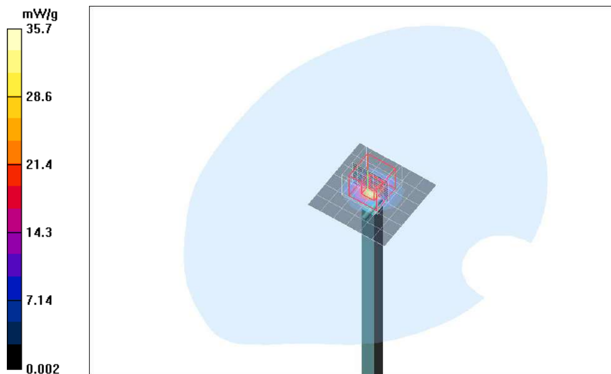
Plot. 18: System Verification Measurement 5250 MHz, Body.
