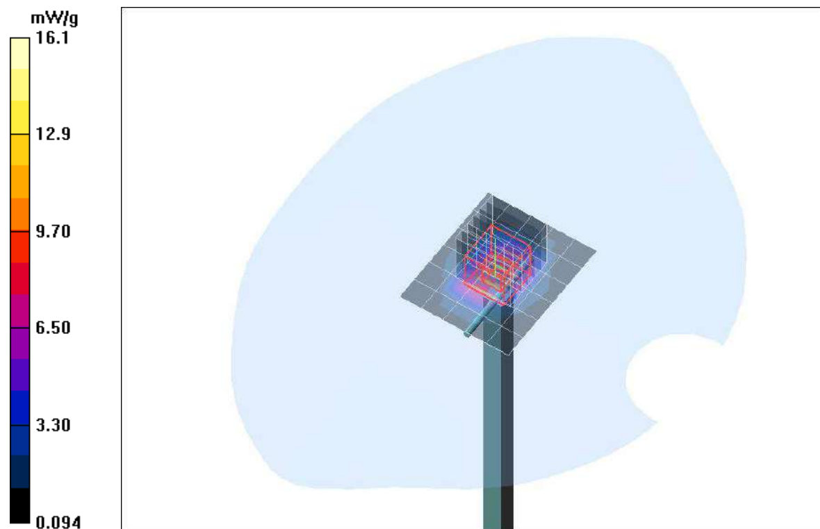
Plot. 12: System Verification Measurement 2450 MHz, Head..
