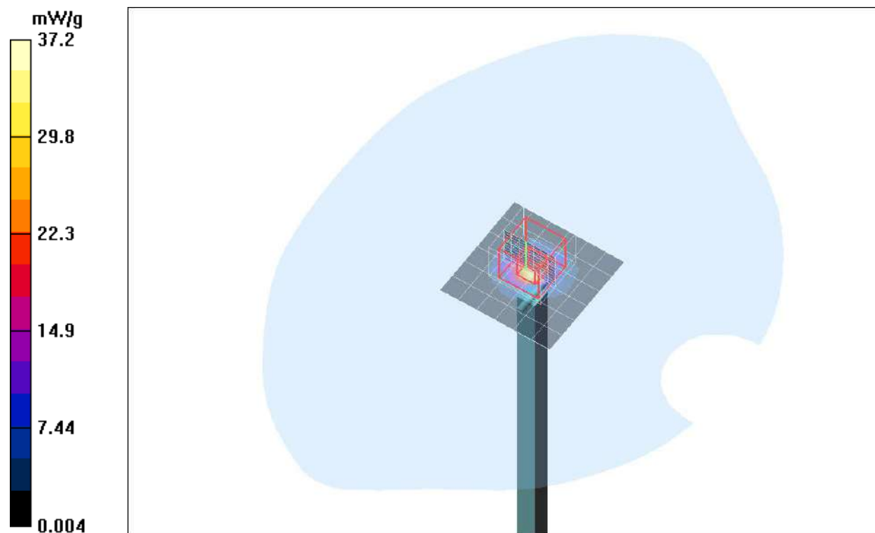
Plot. 19: System Verification Measurement 5600 MHz, Body.
