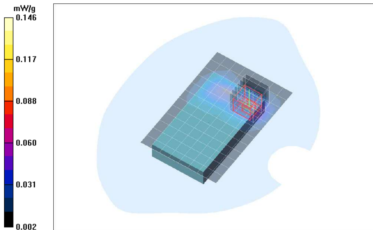
Plot. 8: SAR distribution plot for IEEE802.11b, channel 11, Data Rate 1 MB/s, Body-Worn Configuration, front side, 0mm distance to phantom.
