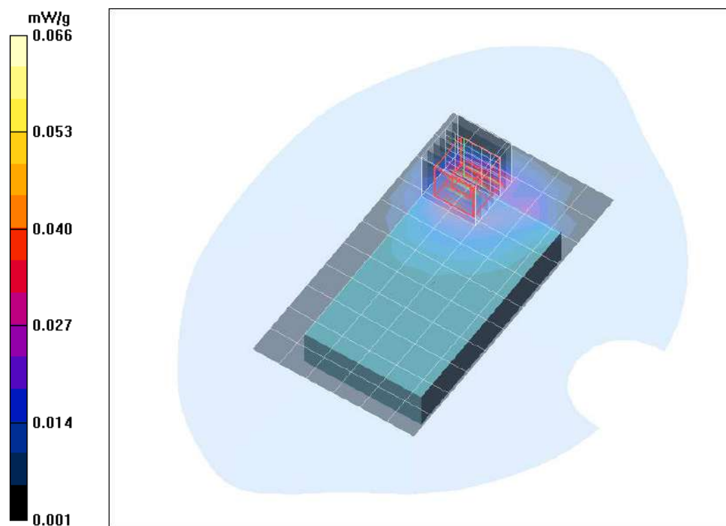
Plot. 7: SAR distribution plot for DECT (Ant.1), channel 2, Body-Worn Configuration, back side, 0mm distance to phantom.
