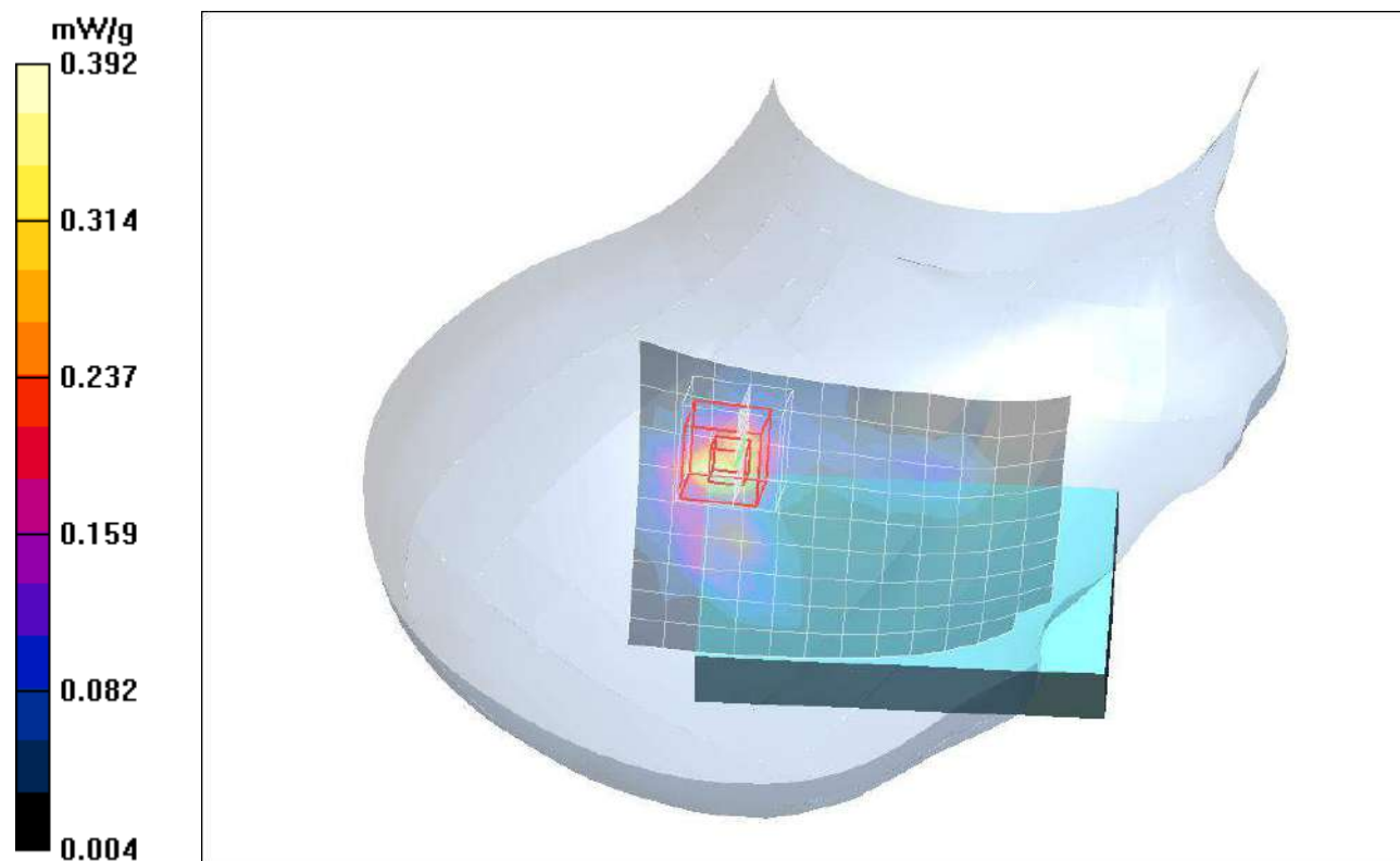
Plot. 5: SAR distribution plot for IEEE802.11a, channel 100, Head Configuration, Right Cheek.
