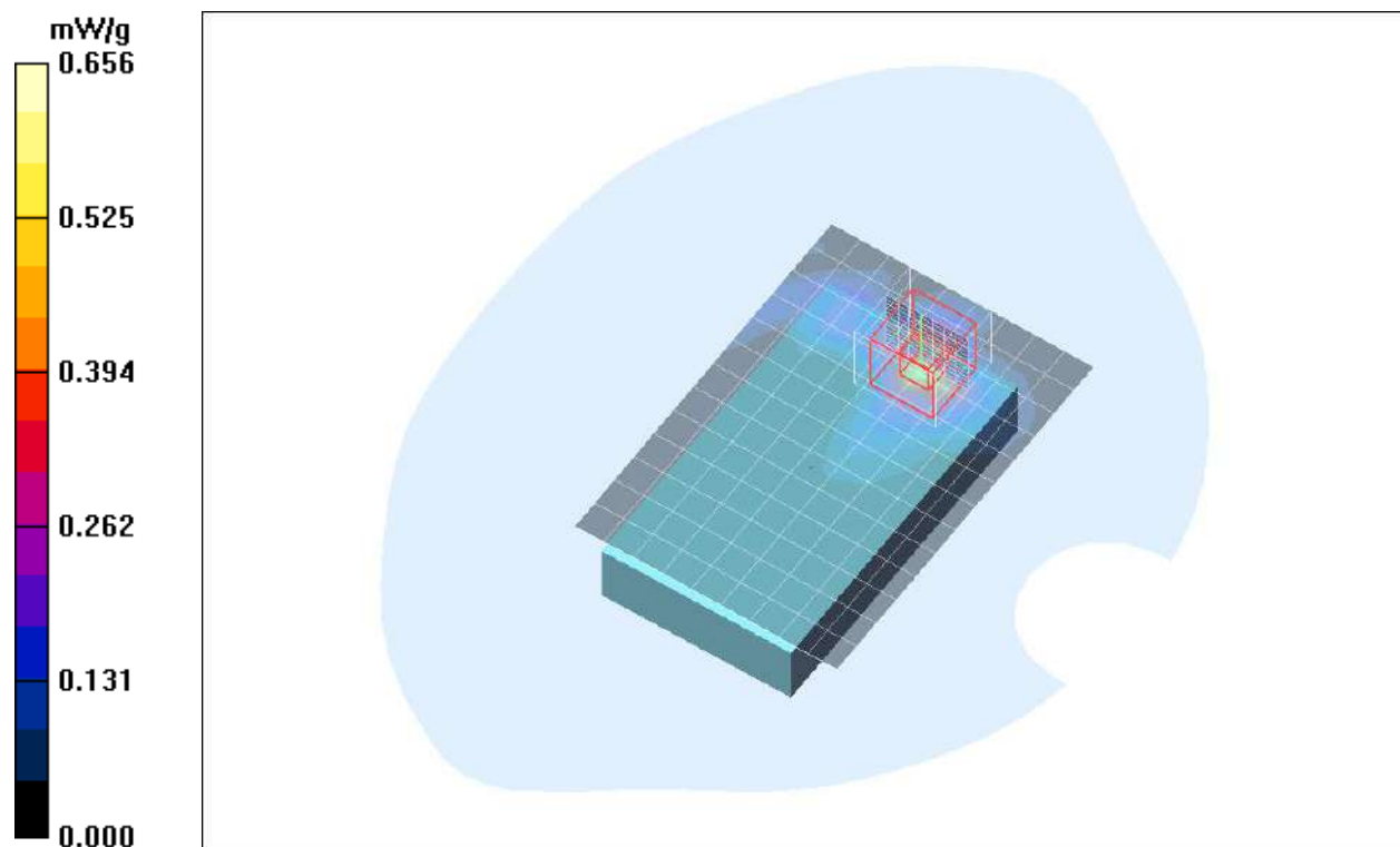
Plot. 10: SAR distribution plot for IEEE802.11a, channel 128, Data Rate 6 MB/s, Body-Worn Configuration, front side, 0mm distance to phantom.
