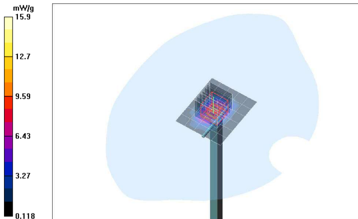
Plot. 17: System Verification Measurement 2450 MHz, Body.
