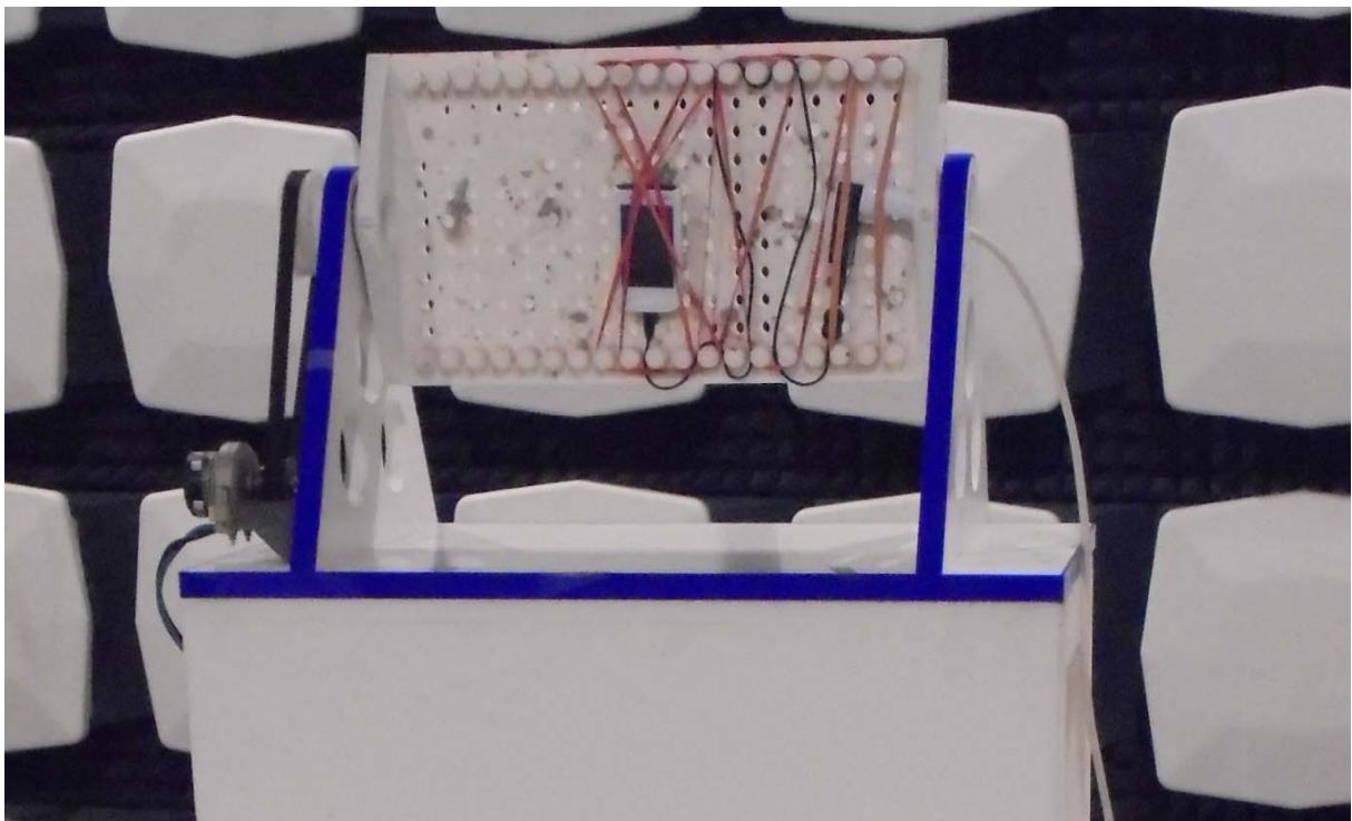
Test set-up, close up view
