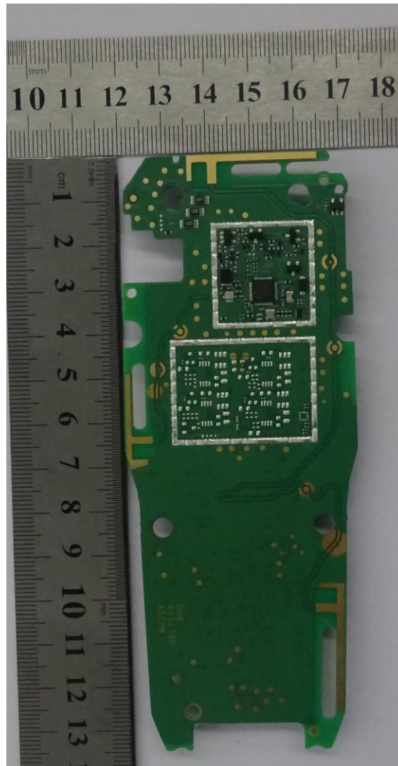
Rear view – main board
