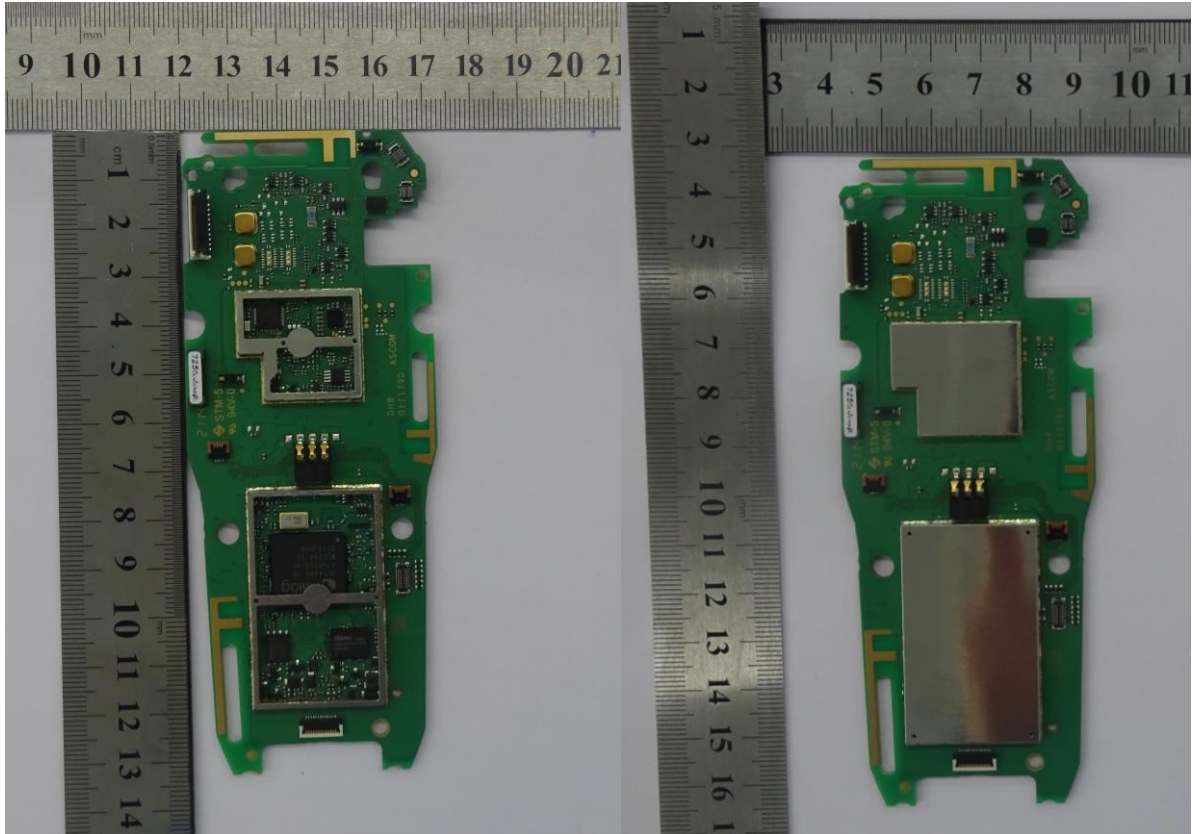
Top view – main board
