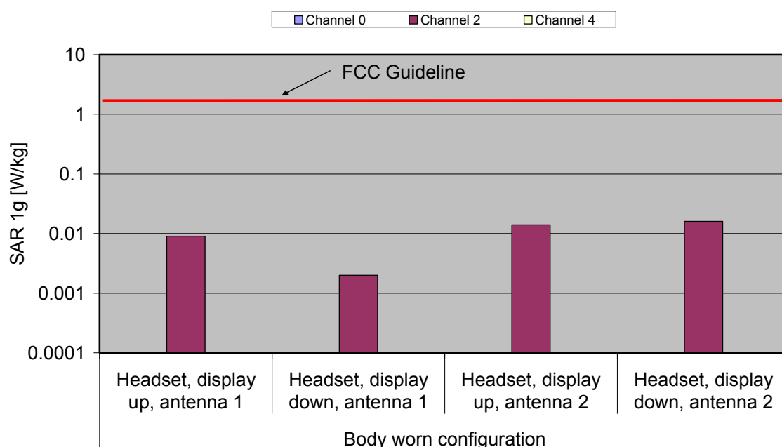
Fig. 10: The measured SAR values in body-worn configuration for the Ascom DH5 for the US DECT standard in comparison to the FCC exposure limit.
