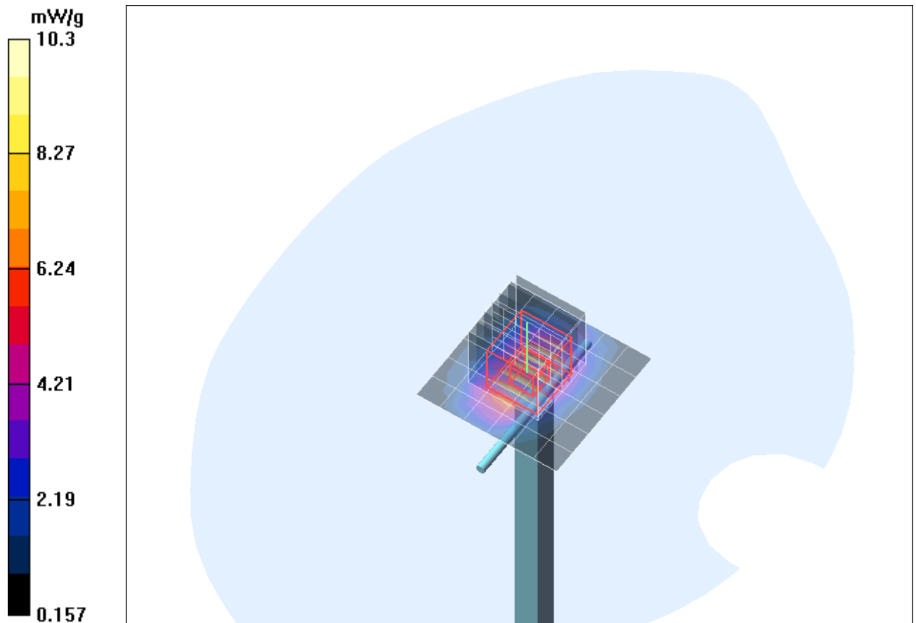
Fig. 11: Validation measurement 1900 MHz Head (February 08, 2010), coarse grid. Ambient Temperature: 20.6° C, Liquid Temperature: 20.1° C.
