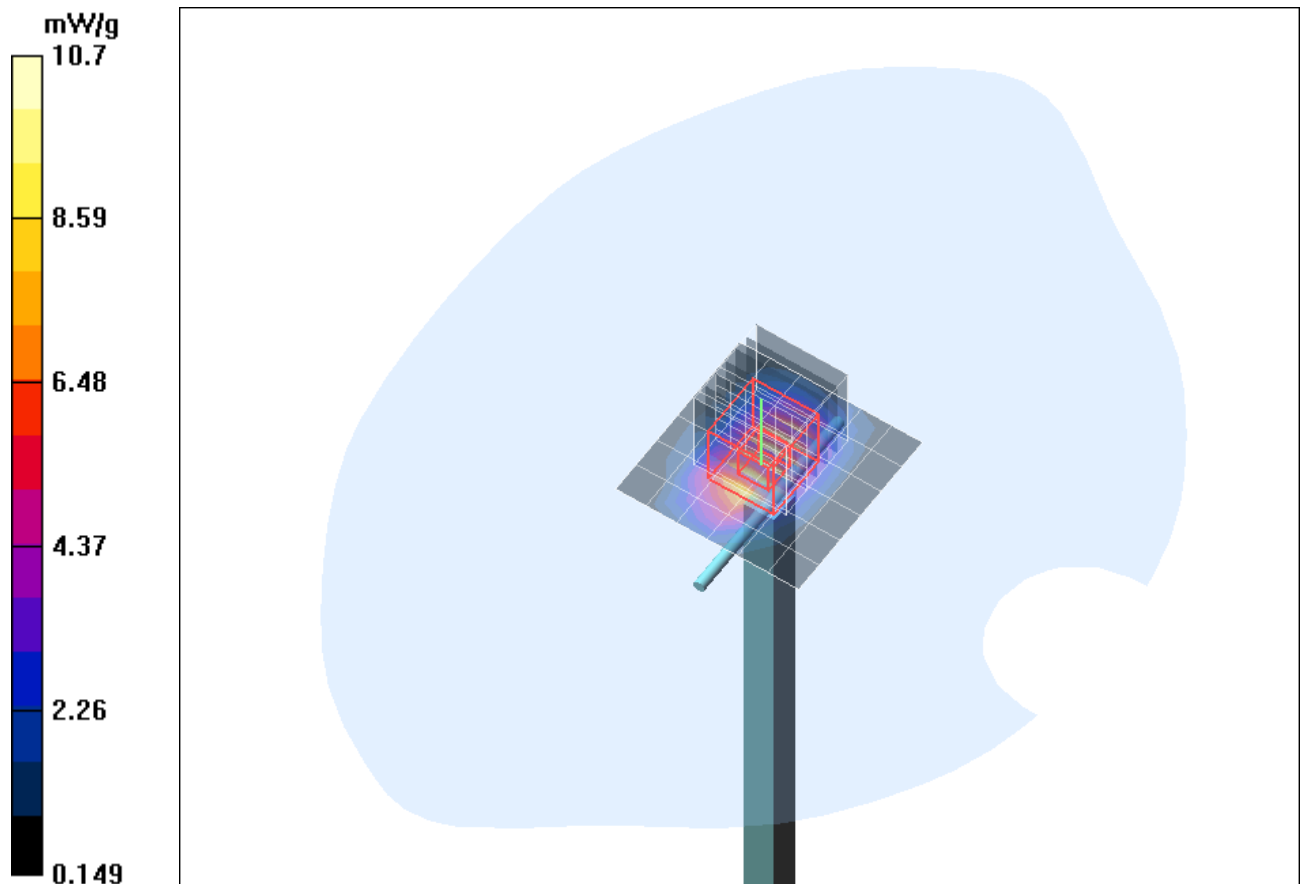
Fig. 12: Validation measurement 1900 MHz body (February 10, 2010), coarse grid. Ambient Temperature: 20.6° C, Liquid Temperature: 20.1° C.
