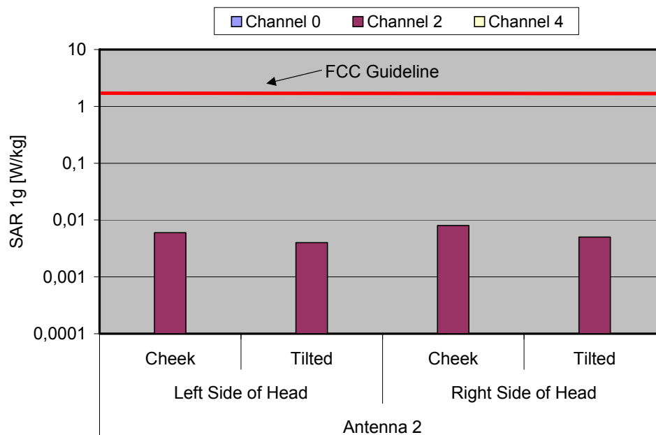
Fig. 9: The measured head phantom SAR values for the Ascom DH5, with antenna 2 for the US DECT standard in comparison to the FCC exposure limit.
