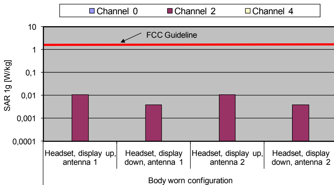
Fig. 10: The measured SAR values in body-worn configuration for the Ascom DH5 for the US DECT standard in comparison to the FCC exposure limit.
