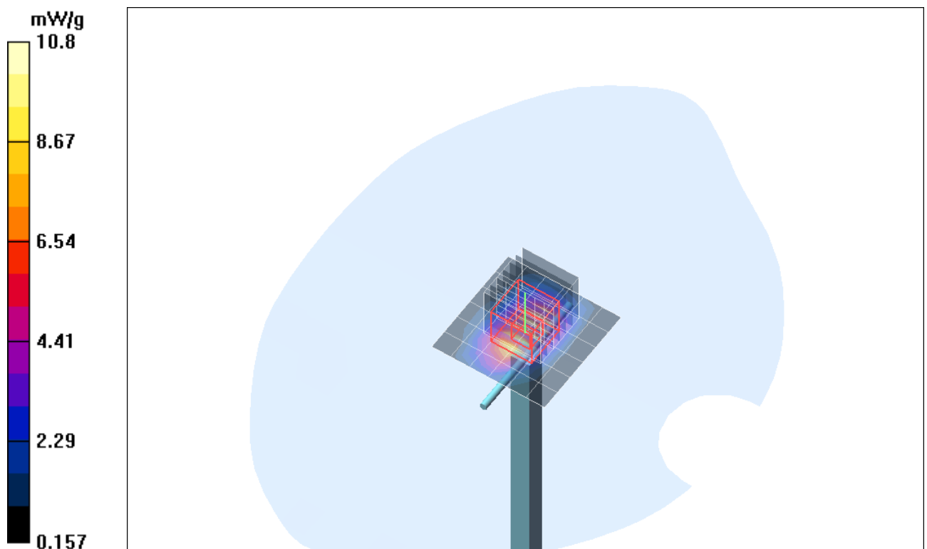
Fig. 12: Validation measurement 1900 MHz body (September 15, 2010), coarse grid. Ambient Temperature: 20.9° C, Liquid Temperature: 20.6° C.
