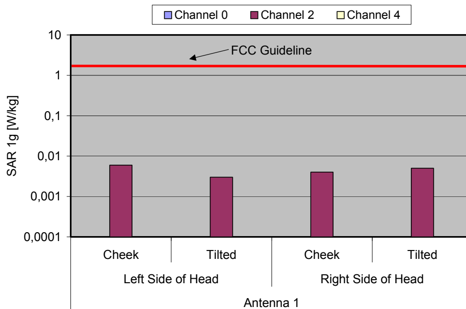
Fig. 8: The measured head phantom SAR values for the Ascom DH5, with antenna 1 for the US DECT standard in comparison to the FCC exposure limit.
