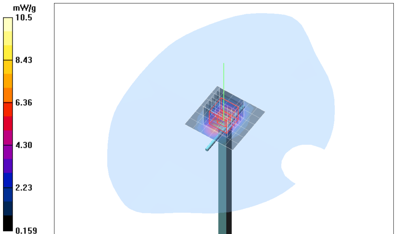
Fig. 11: Validation measurement 1900 MHz Head (September 13, 2010), coarse grid. Ambient Temperature: 20.9° C, Liquid Temperature: 20.5° C.
